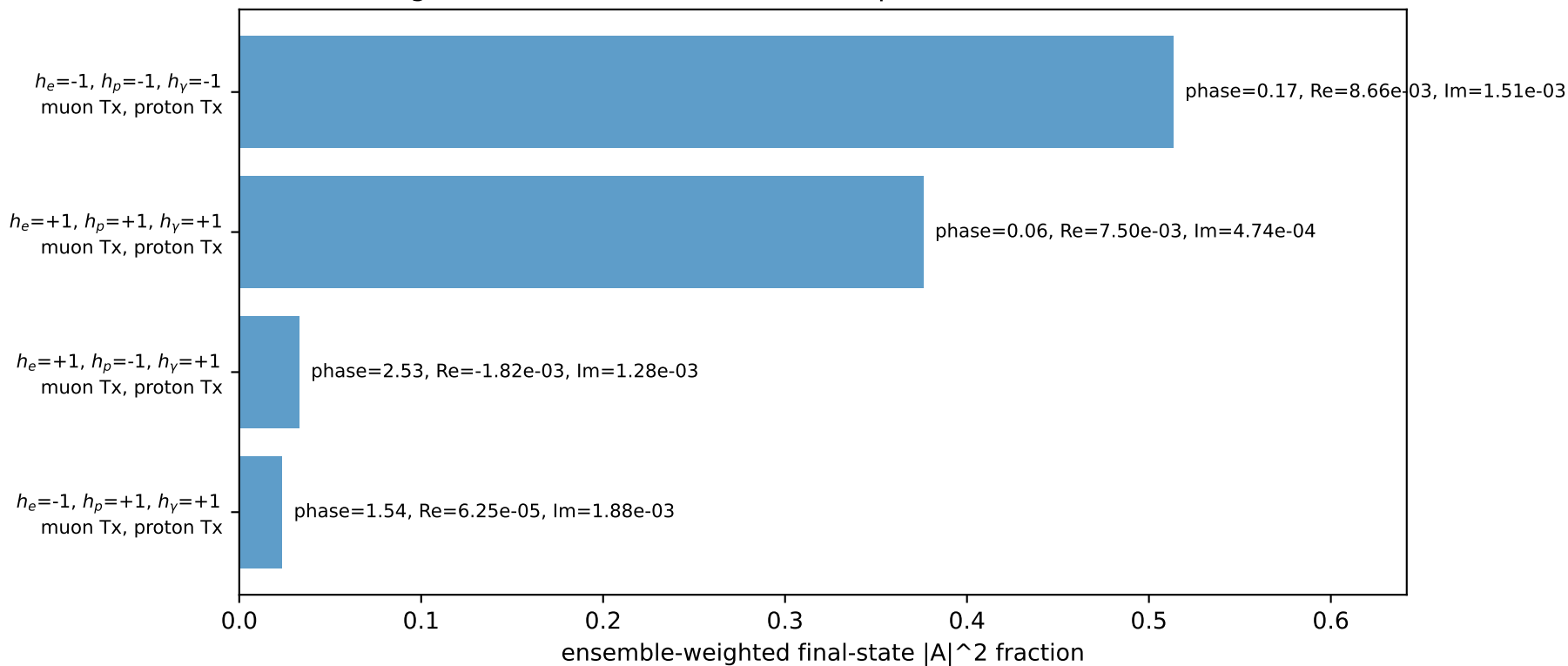
Leading initial-ensemble/final-state components (N=4, retained=94.6%)
