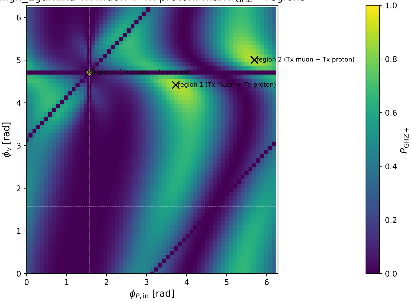
high_Egamma Tx muon + Tx proton: max P_{\text{GHZ}+} regions
