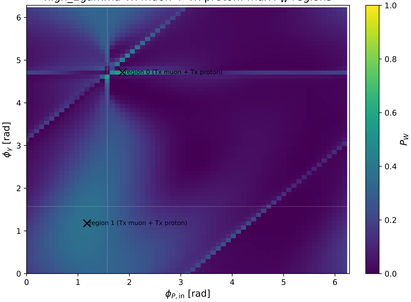
high_Egamma Tx muon + Tx proton: max P_W regions
