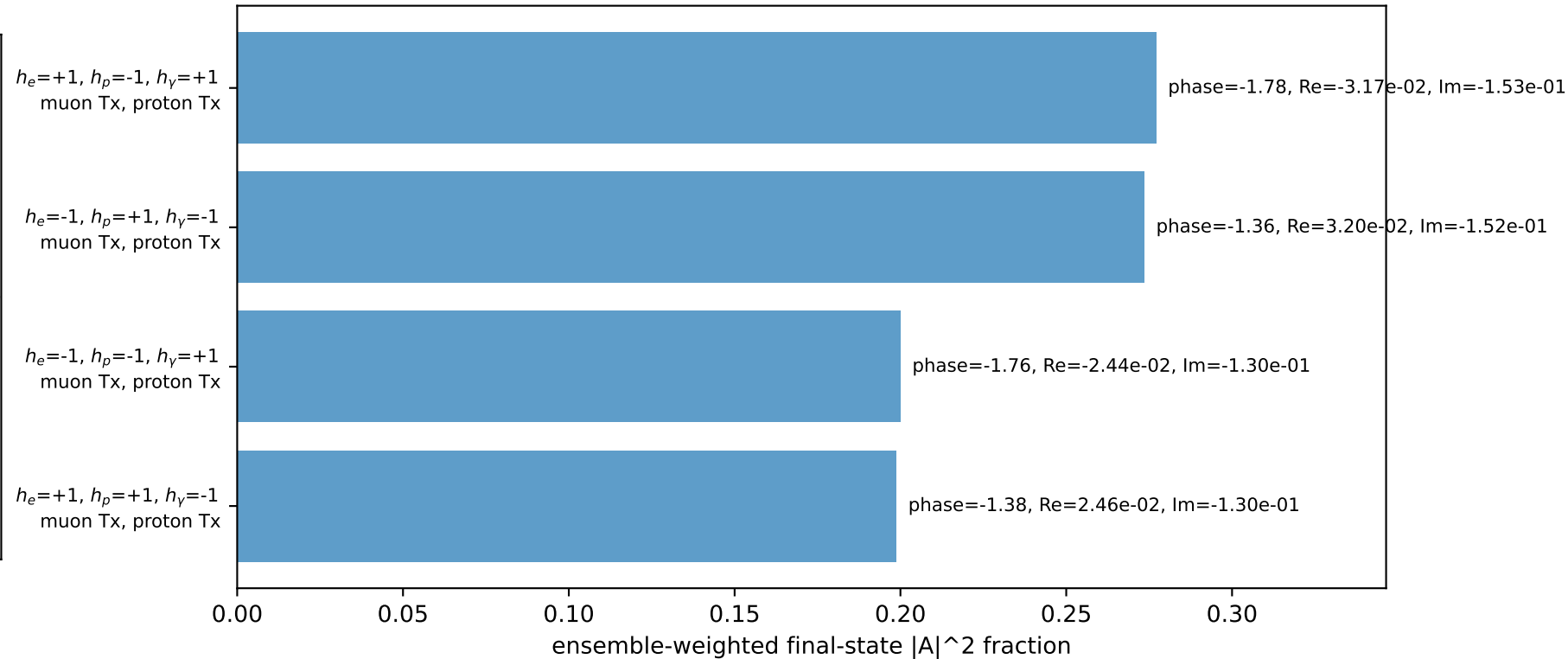
Leading initial-ensemble/final-state components (N=4, retained=95.0%)
