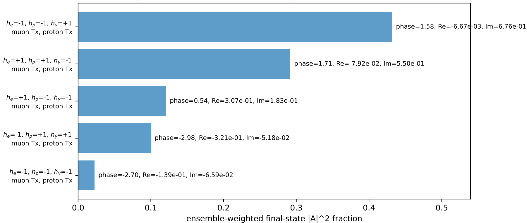
Leading initial-ensemble/final-state components (N=5, retained=96.6%)
