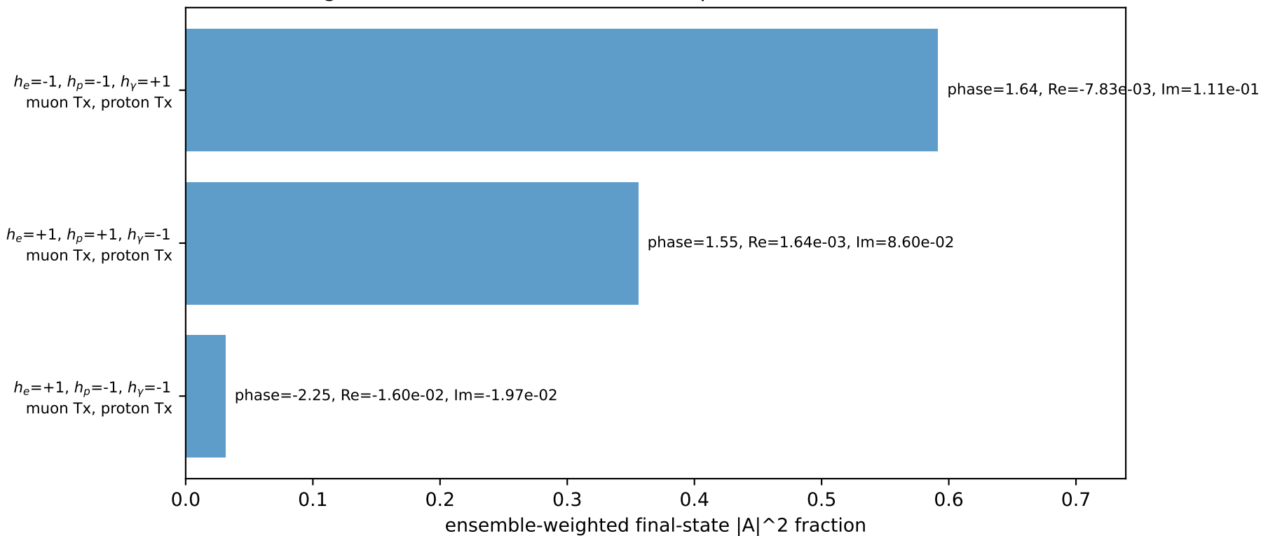
Leading initial-ensemble/final-state components (N=3, retained=97.8%)
