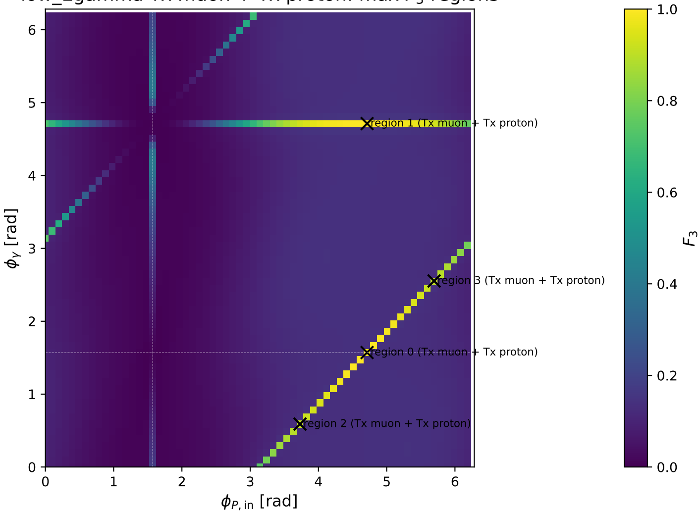
low_Egamma Tx muon + Tx proton: max F_3 regions
