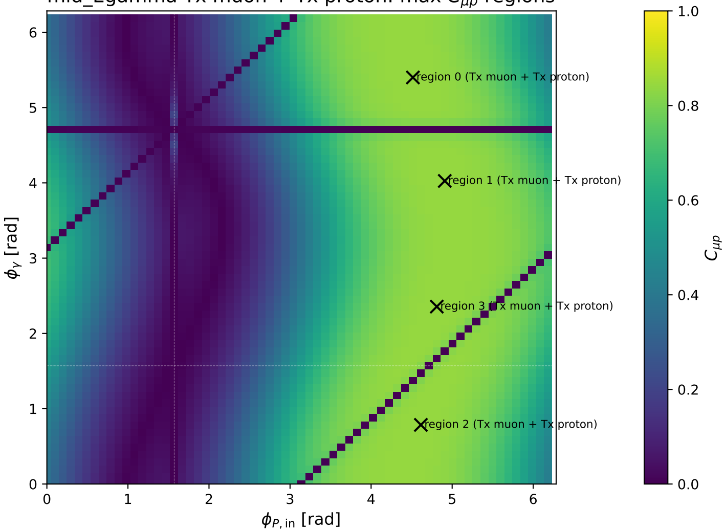
mid_Egamma Tx muon + Tx proton: max C_{\mu p} regions
