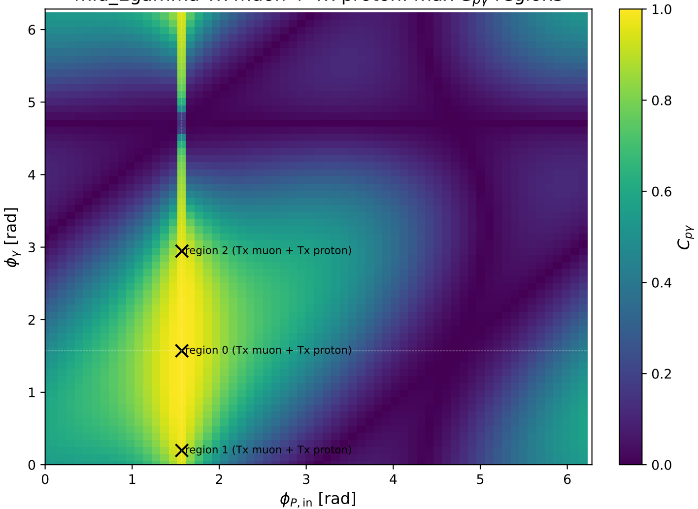
mid_Egamma Tx muon + Tx proton: max C_{p\gamma} regions
