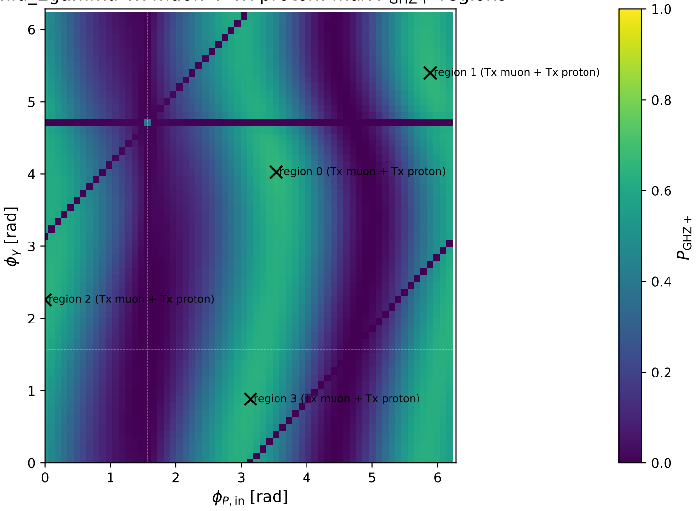
mid_Egamma Tx muon + Tx proton: max P_{\text{GHz}+} regions
