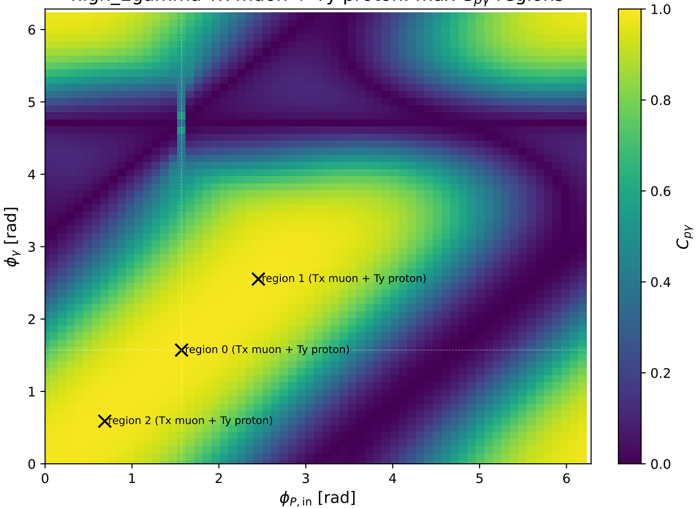
high_Egamma Tx muon + Ty proton: max C_{p\gamma} regions
