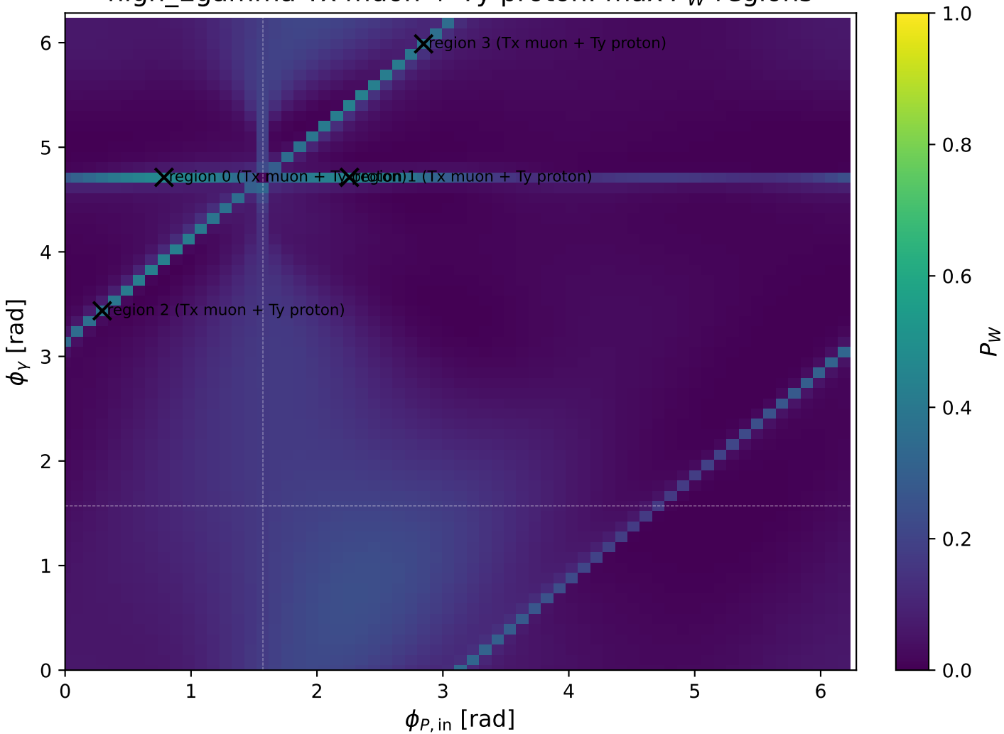
high_Egamma Tx muon + Ty proton: max P_W regions
