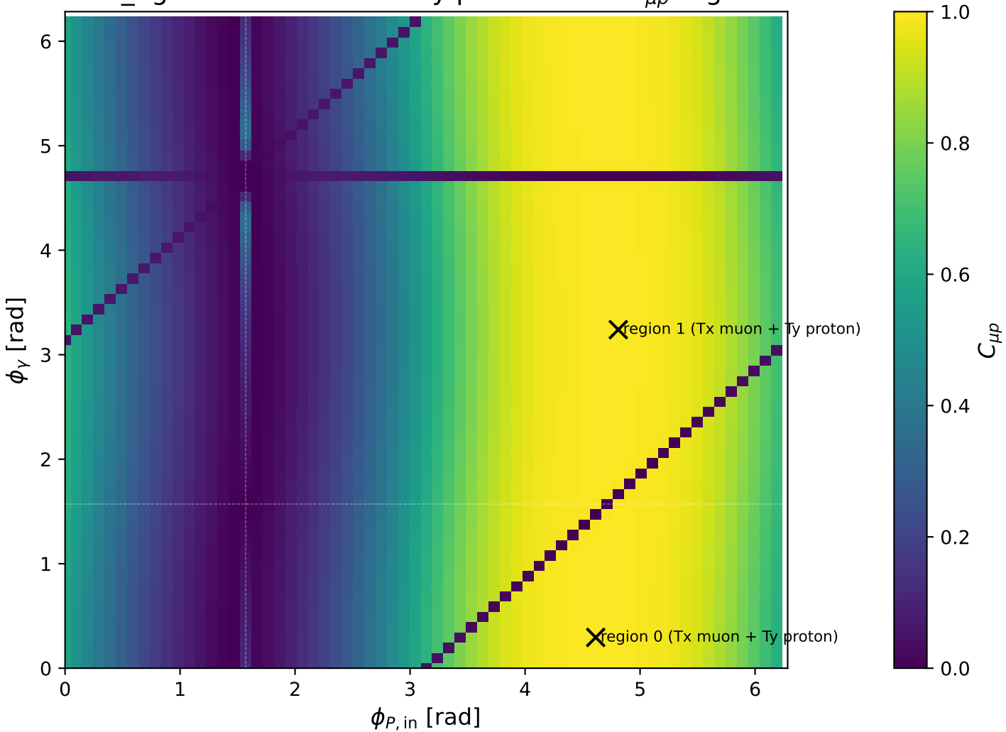
low_Egamma Tx muon + Ty proton: max C_{\mu p} regions
