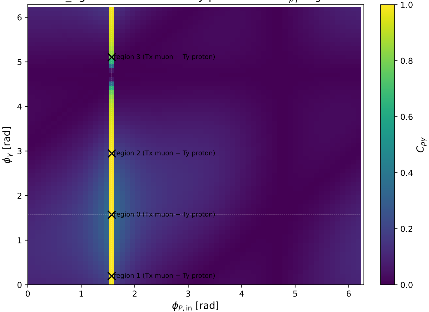
low_Egamma Tx muon + Ty proton: max C_{p\gamma} regions
