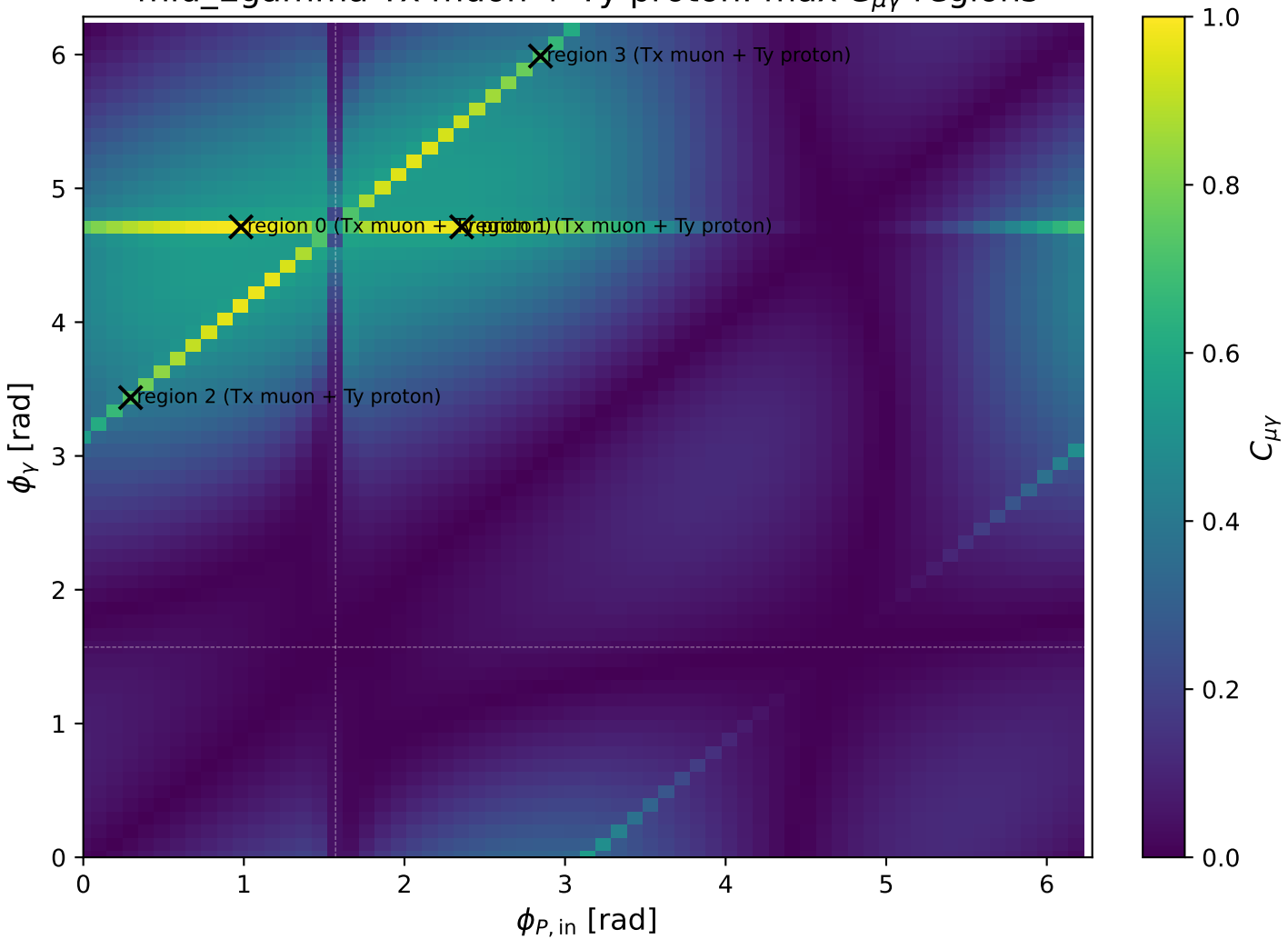
mid_Egamma Tx muon + Ty proton: max C_{\mu\gamma} regions
