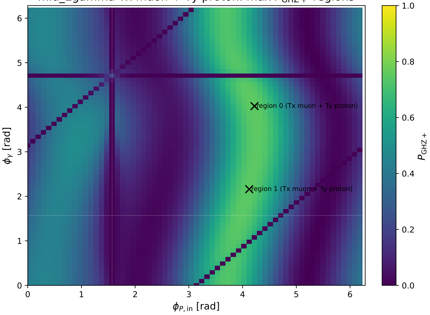
mid_Egamma Tx muon + Ty proton: max P_{\text{GHZ}+} regions
