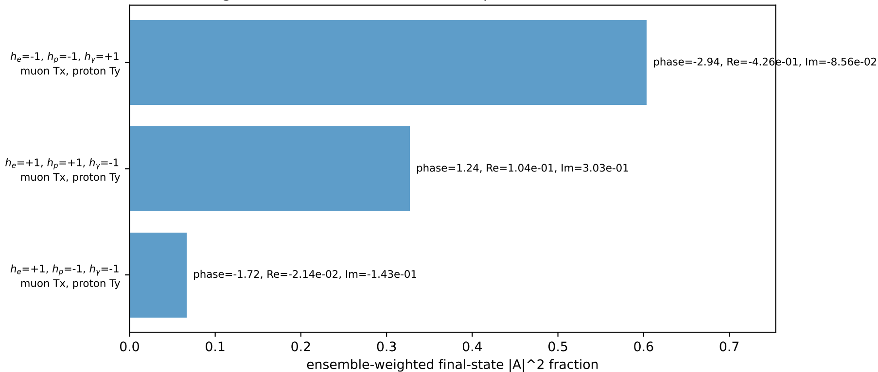
Leading initial-ensemble/final-state components (N=3, retained=99.7%)
