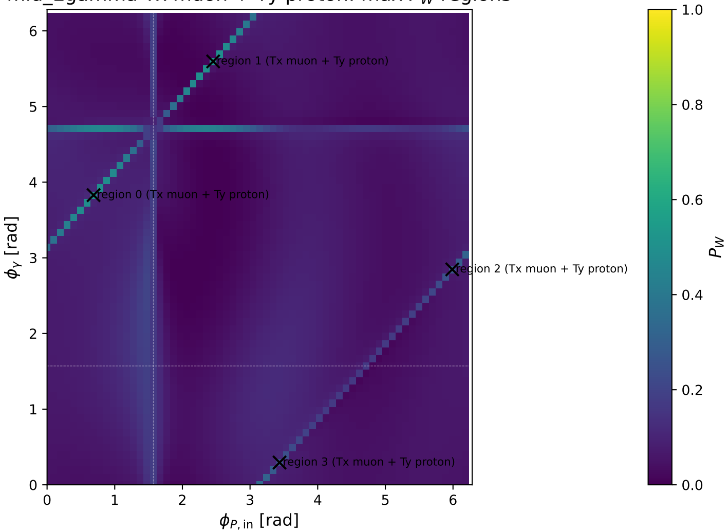
mid_Egamma Tx muon + Ty proton: max P_W regions
