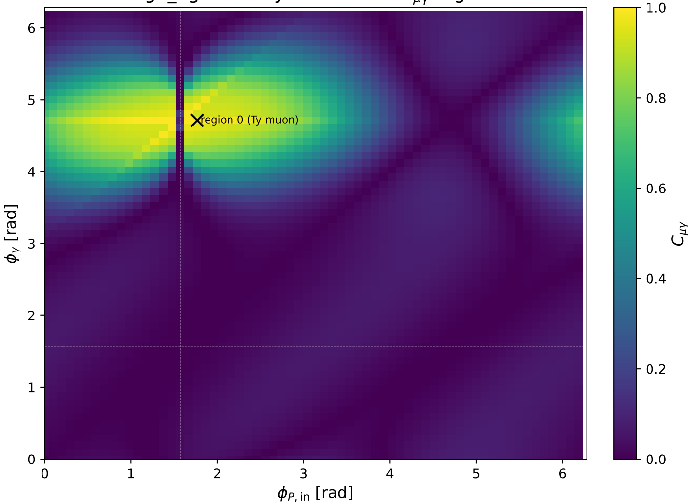
high_Egamma Ty muon: max C_{\mu\gamma} regions
