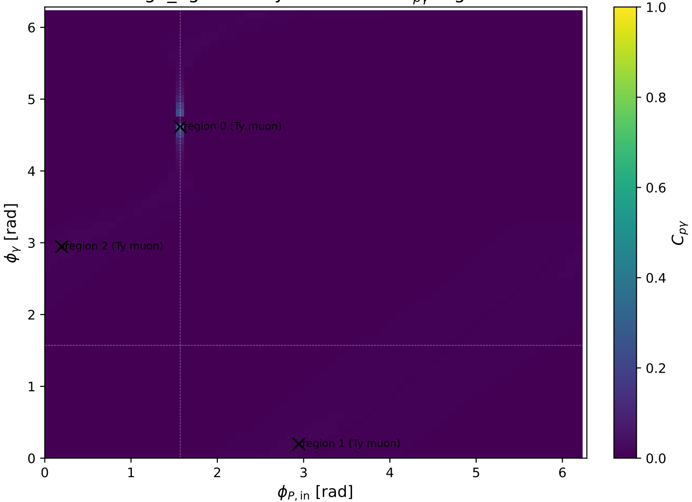
high_Egamma Ty muon: max C_{p\gamma} regions
