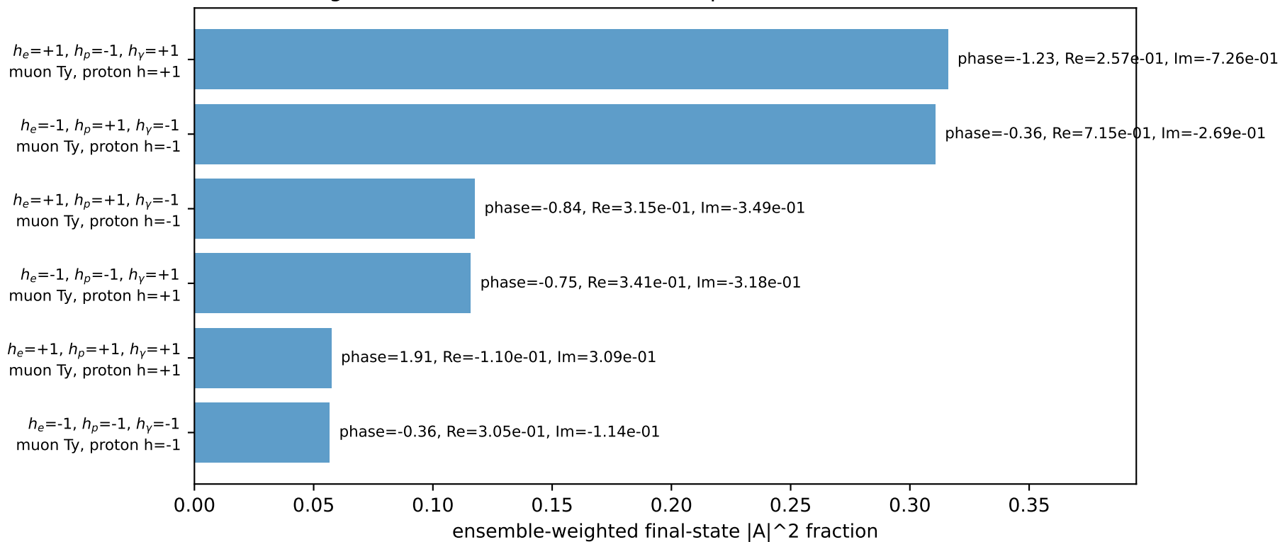
Leading initial-ensemble/final-state components (N=6, retained=97.4%)
