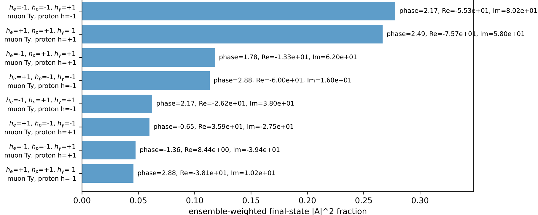
Leading initial-ensemble/final-state components (N=8, retained=99.1%)
