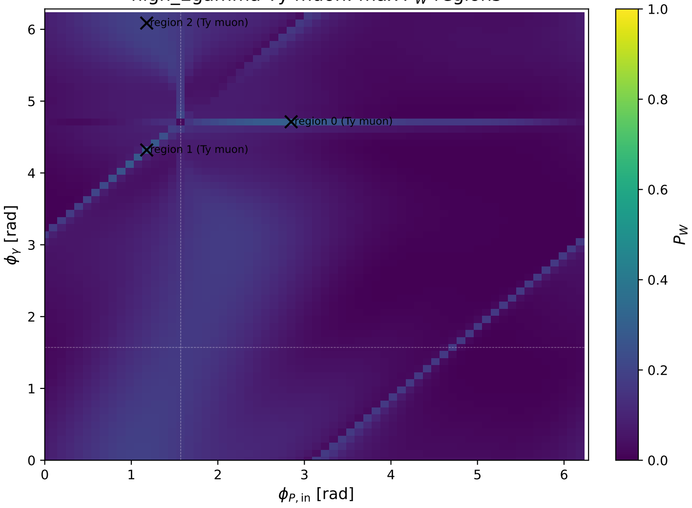
high_Egamma Ty muon: max P_W regions
