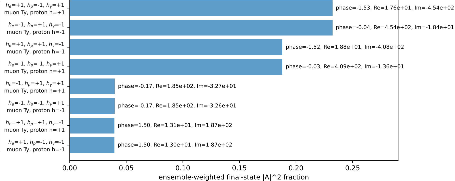
Leading initial-ensemble/final-state components (N=8, retained=99.9%)
