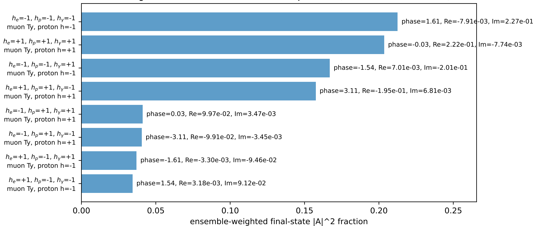
Leading initial-ensemble/final-state components (N=8, retained=89.3%)
