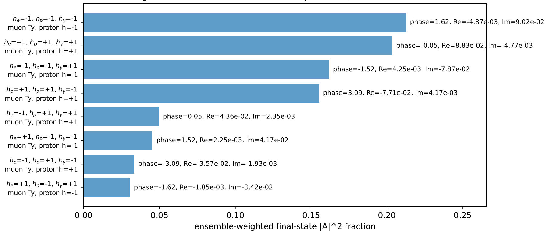
Leading initial-ensemble/final-state components (N=8, retained=89.2%)
