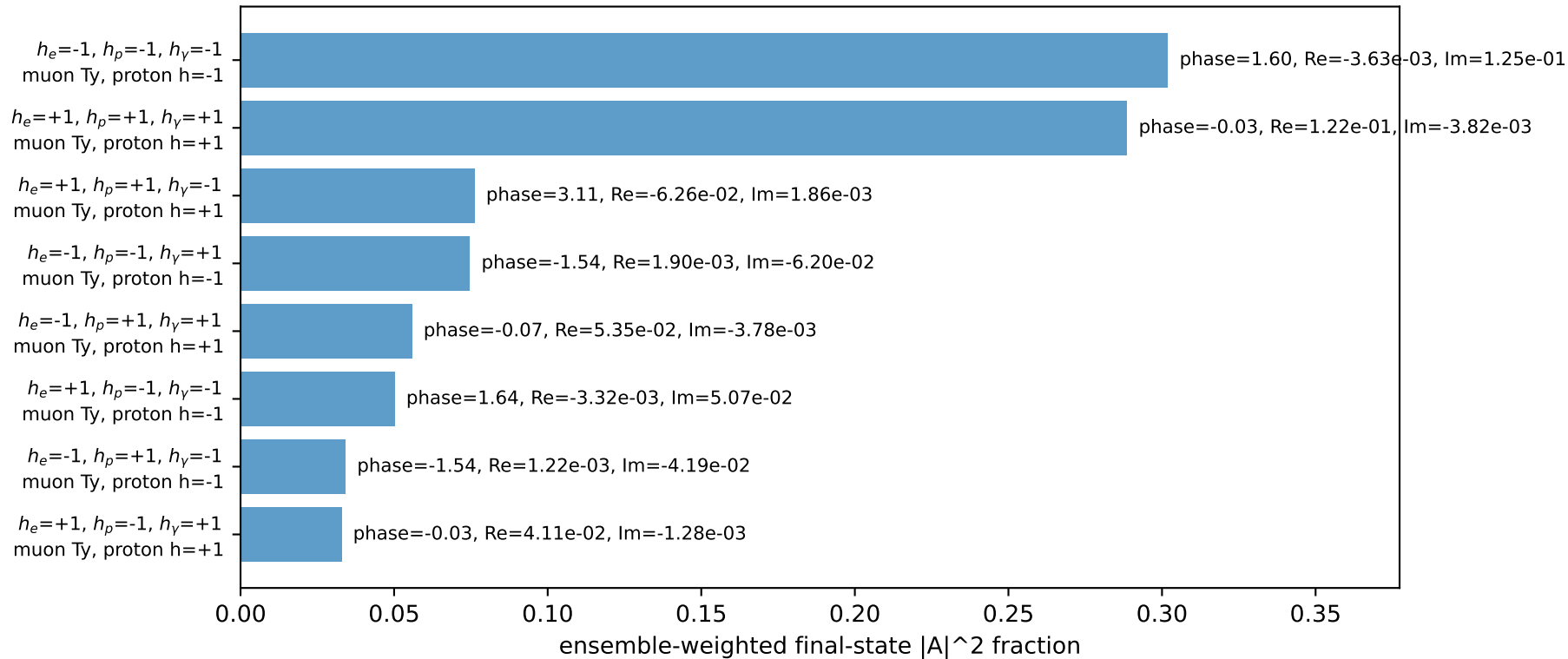
Leading initial-ensemble/final-state components (N=8, retained=91.4%)
