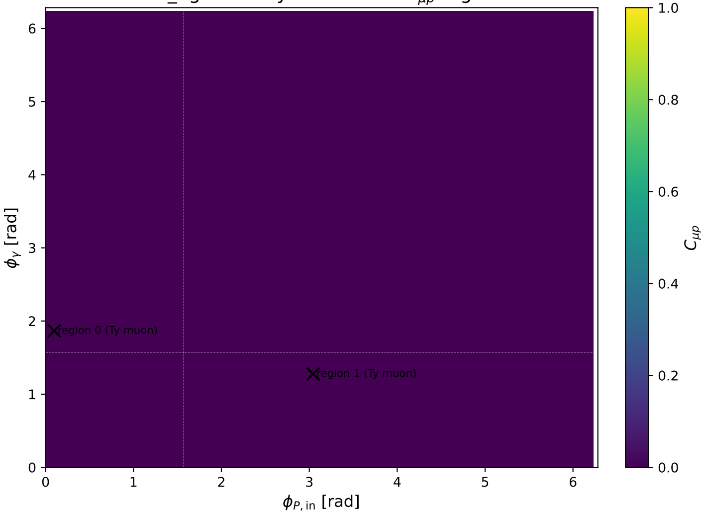
mid_Egamma Ty muon: max C_{\mu p} regions
