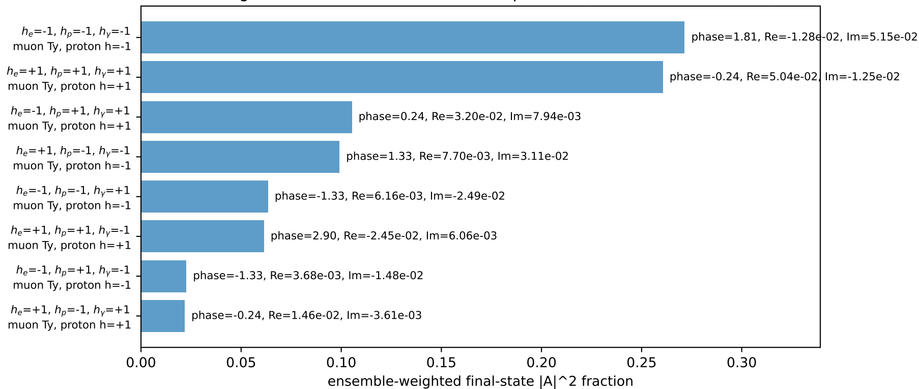
Leading initial-ensemble/final-state components (N=8, retained=90.5%)
