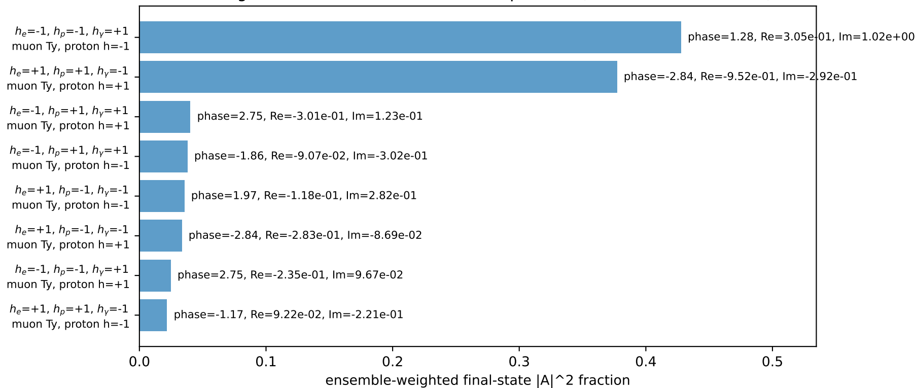
Leading initial-ensemble/final-state components (N=8, retained=99.8%)
