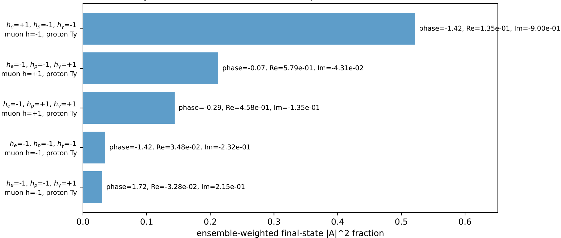
Leading initial-ensemble/final-state components (N=5, retained=94.2%)
