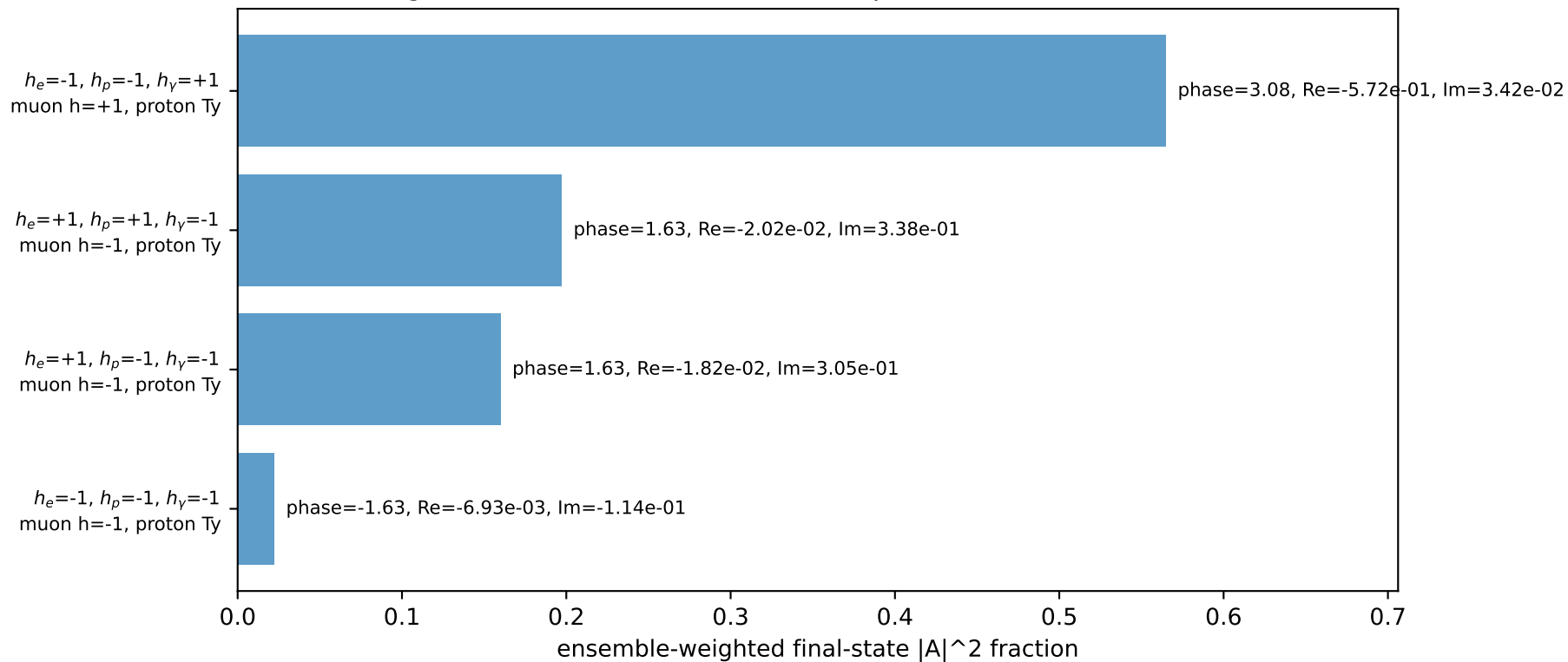
Leading initial-ensemble/final-state components (N=4, retained=94.4%)
