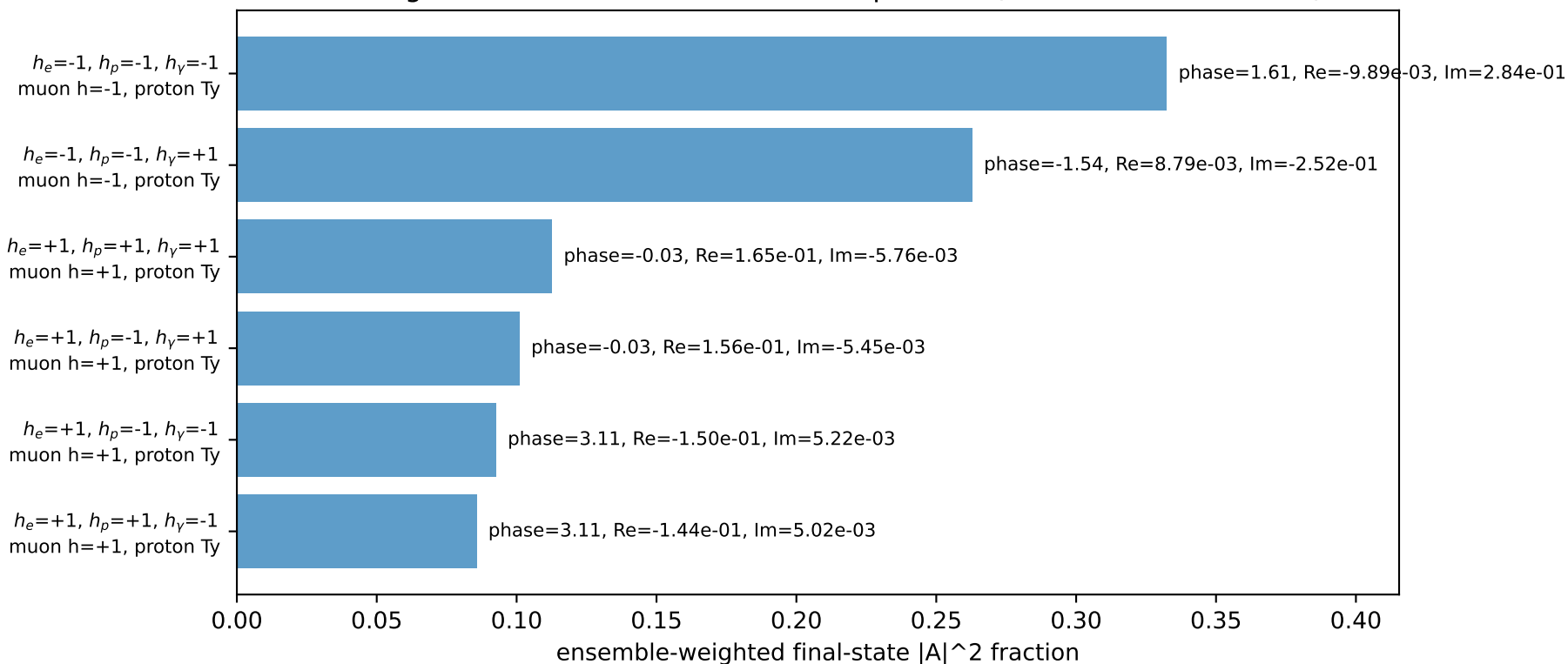
Leading initial-ensemble/final-state components (N=6, retained=98.7%)
