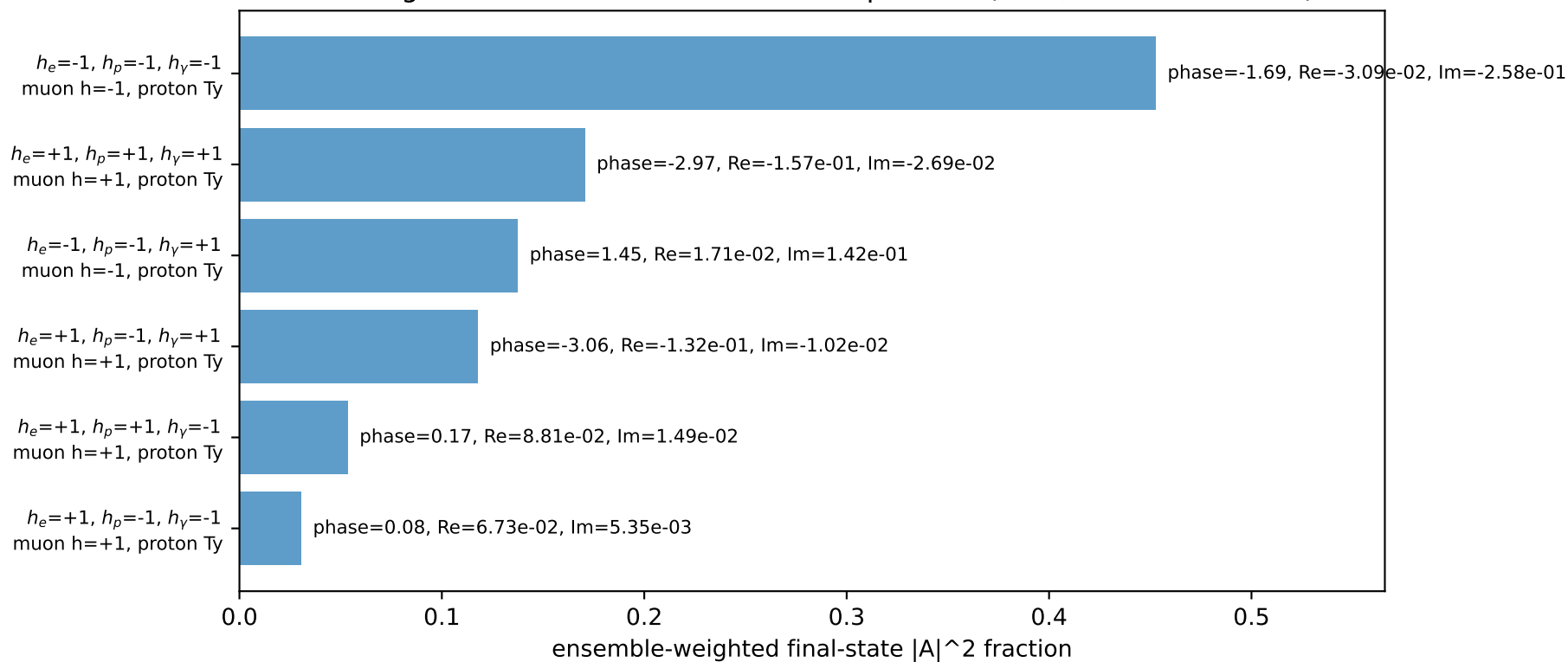
Leading initial-ensemble/final-state components (N=6, retained=96.3%)
