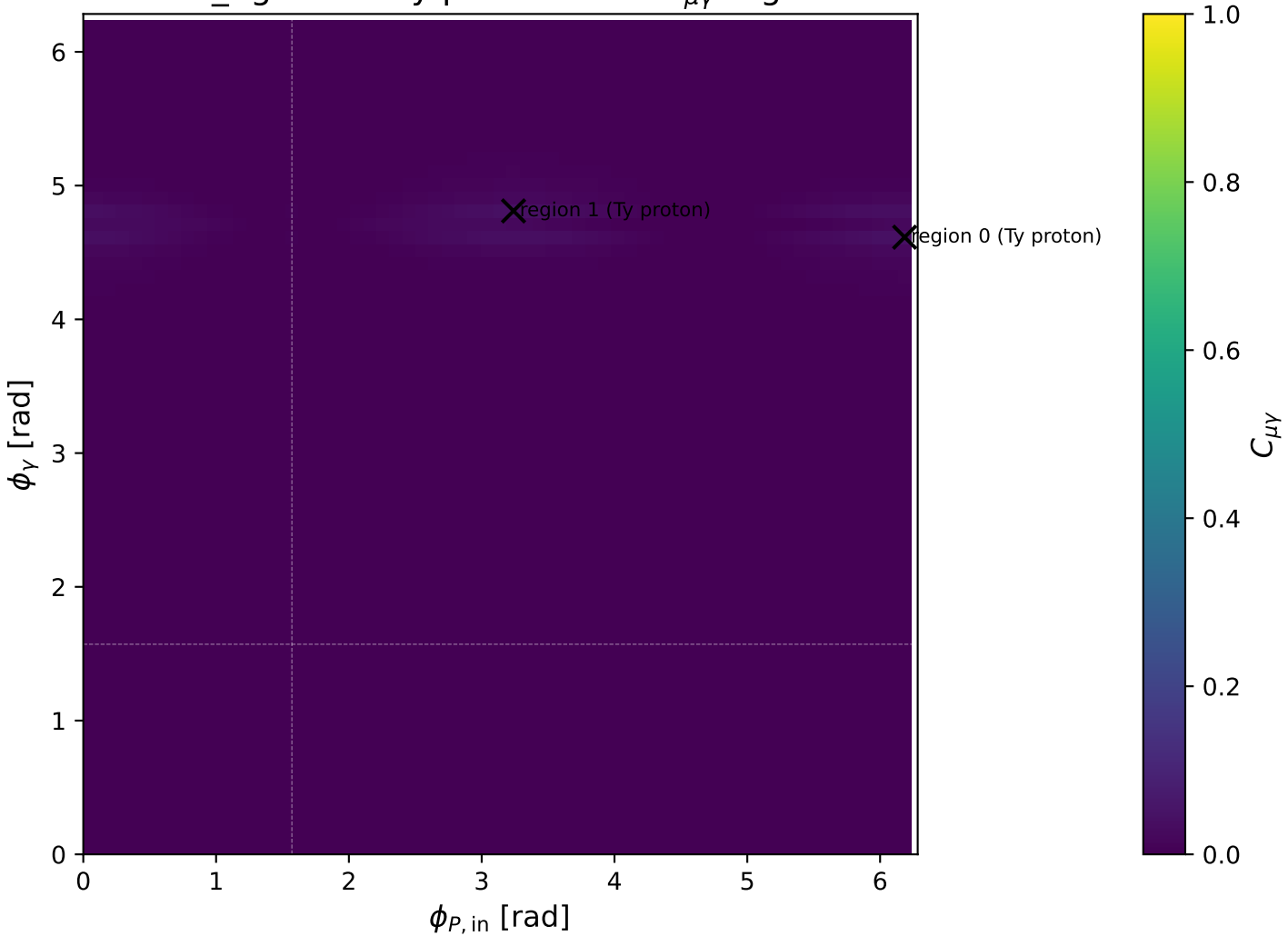
mid_Egamma Ty proton: max C_{\mu\gamma} regions
