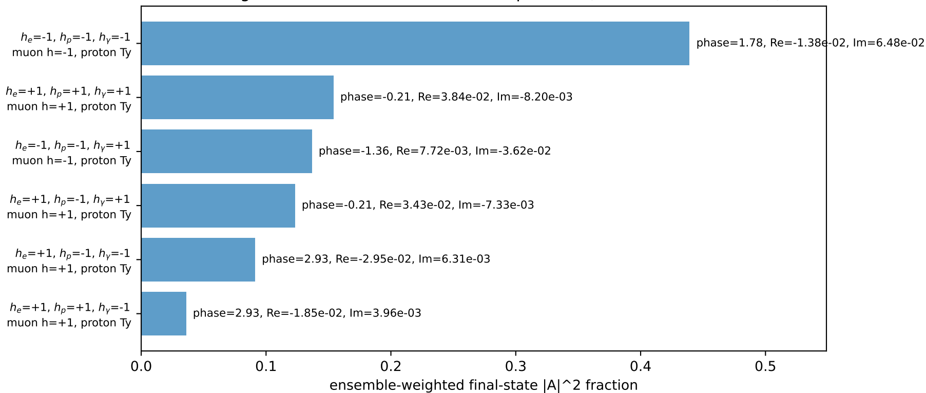
Leading initial-ensemble/final-state components (N=6, retained=97.9%)
