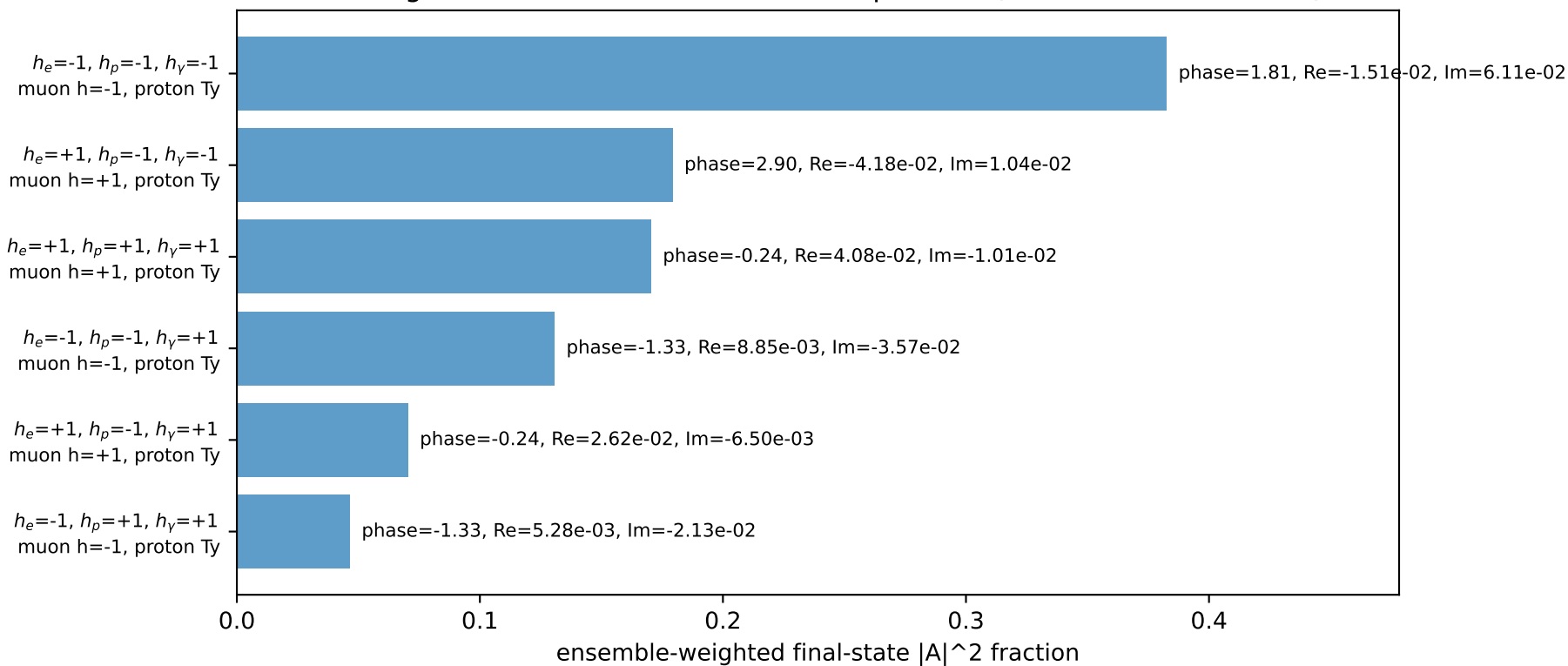
Leading initial-ensemble/final-state components (N=6, retained=98.0%)
