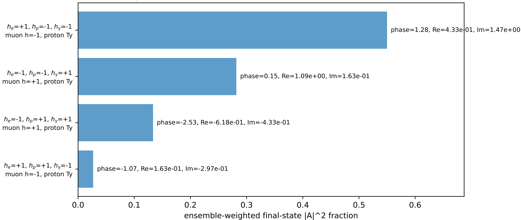
Leading initial-ensemble/final-state components (N=4, retained=99.1%)
