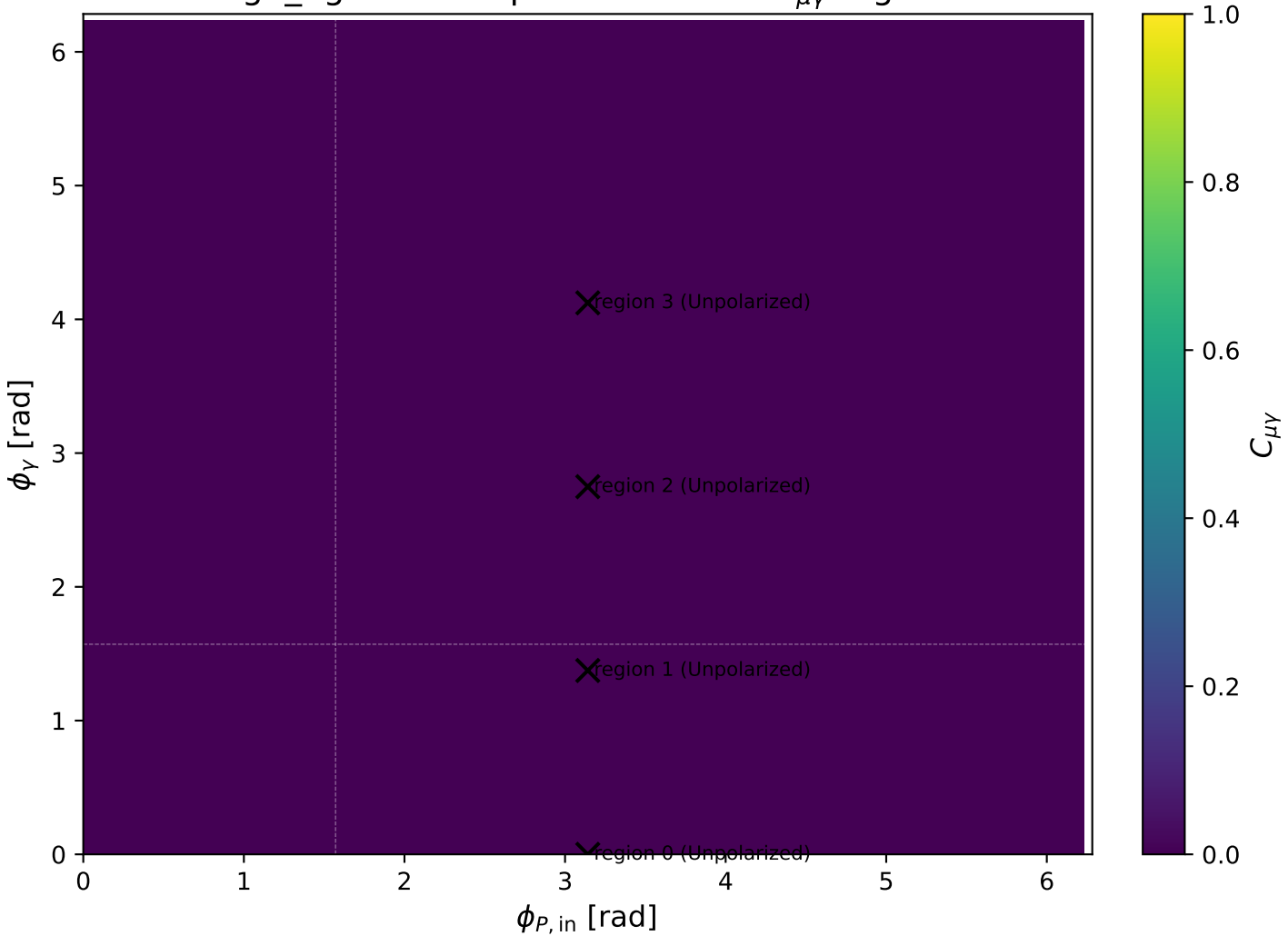
high_Egamma Unpolarized: max C_{\mu\gamma} regions
