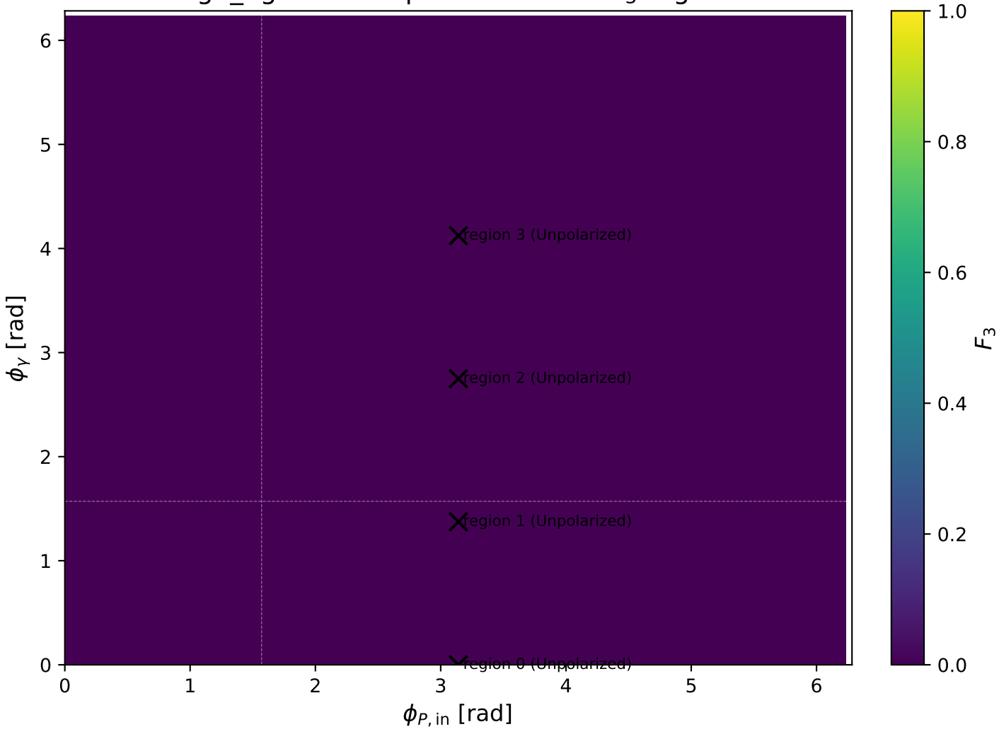
high_Egamma Unpolarized: max F_3 regions
