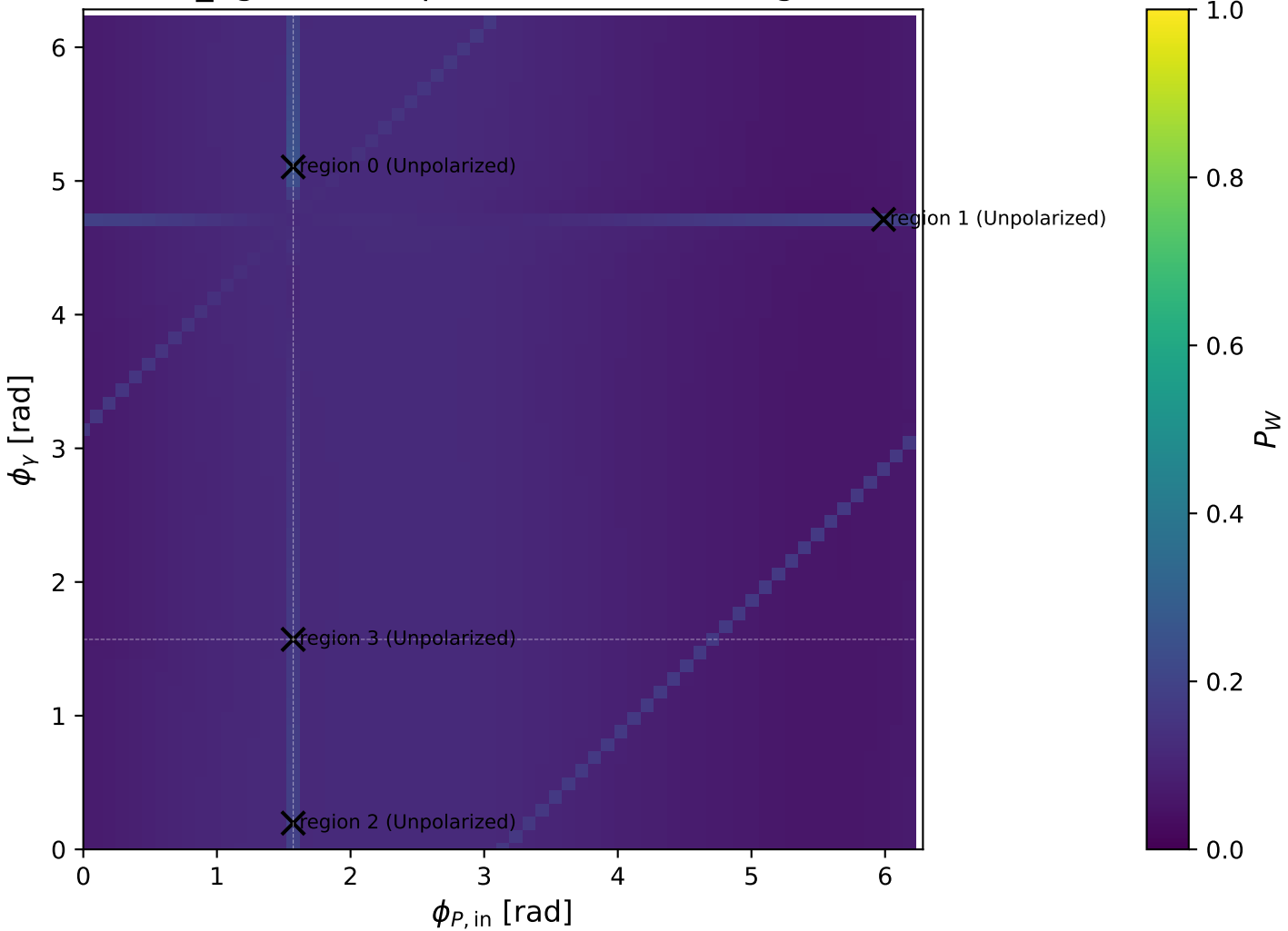
low_Egamma Unpolarized: max P_W regions
