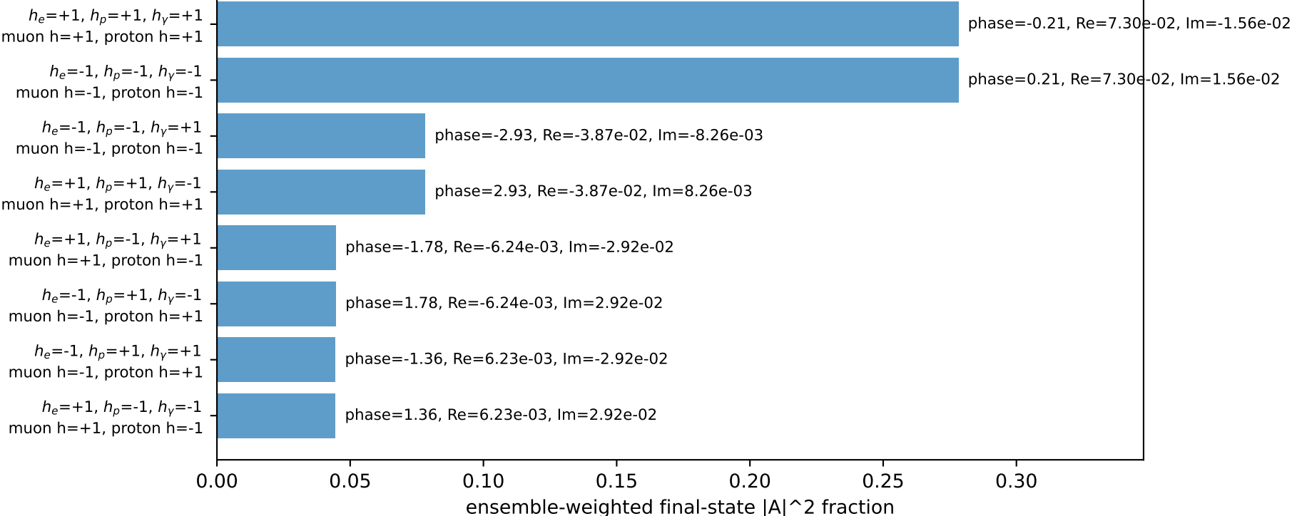
Leading initial-ensemble/final-state components (N=8, retained=89.0%)
