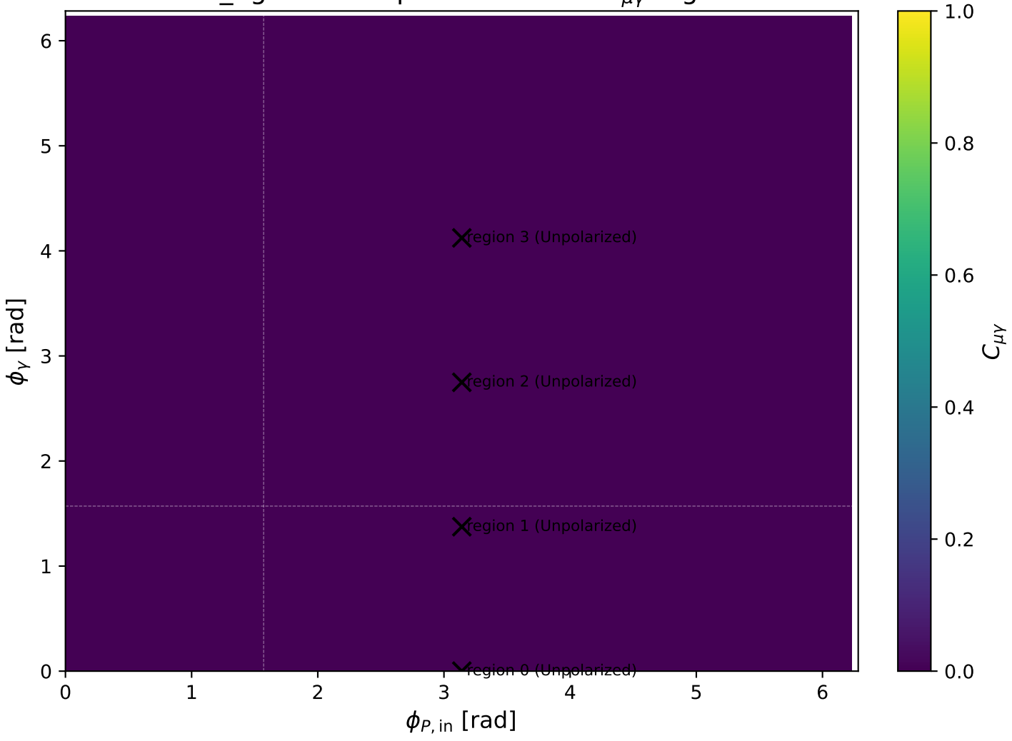
mid_Egamma Unpolarized: max C_{\mu\gamma} regions
