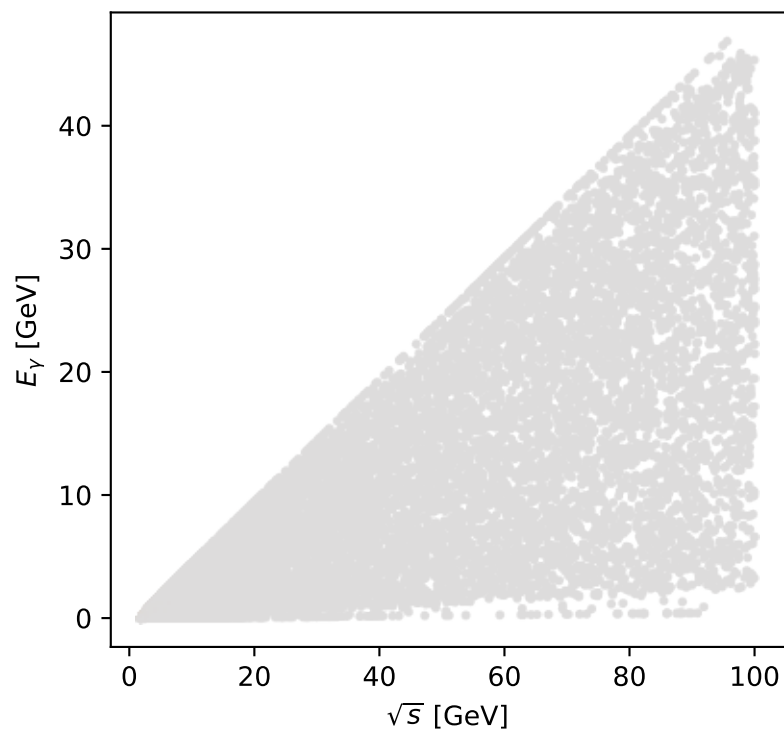
Phase-space scan: L auxiliary lepton + L proton [LL], max M_p=0.15709
