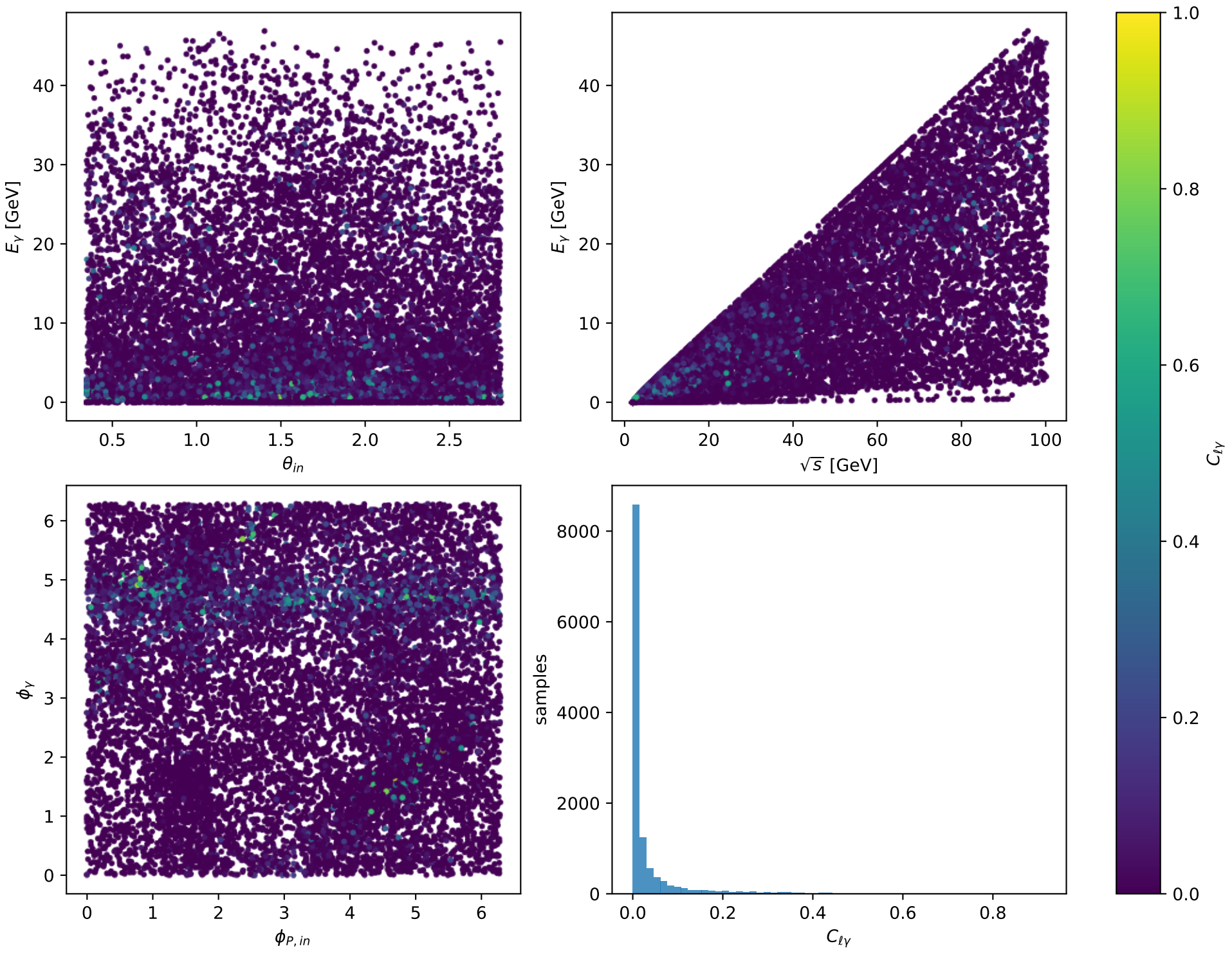
Phase-space scan: L auxiliary lepton + L proton [LL], max C_{\ell\gamma}=0.9173
