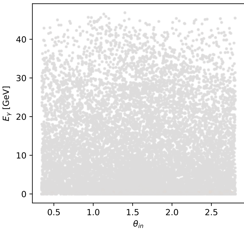
Phase-space scan: L auxiliary lepton + L proton [LL], max M_\ell=0.15709
