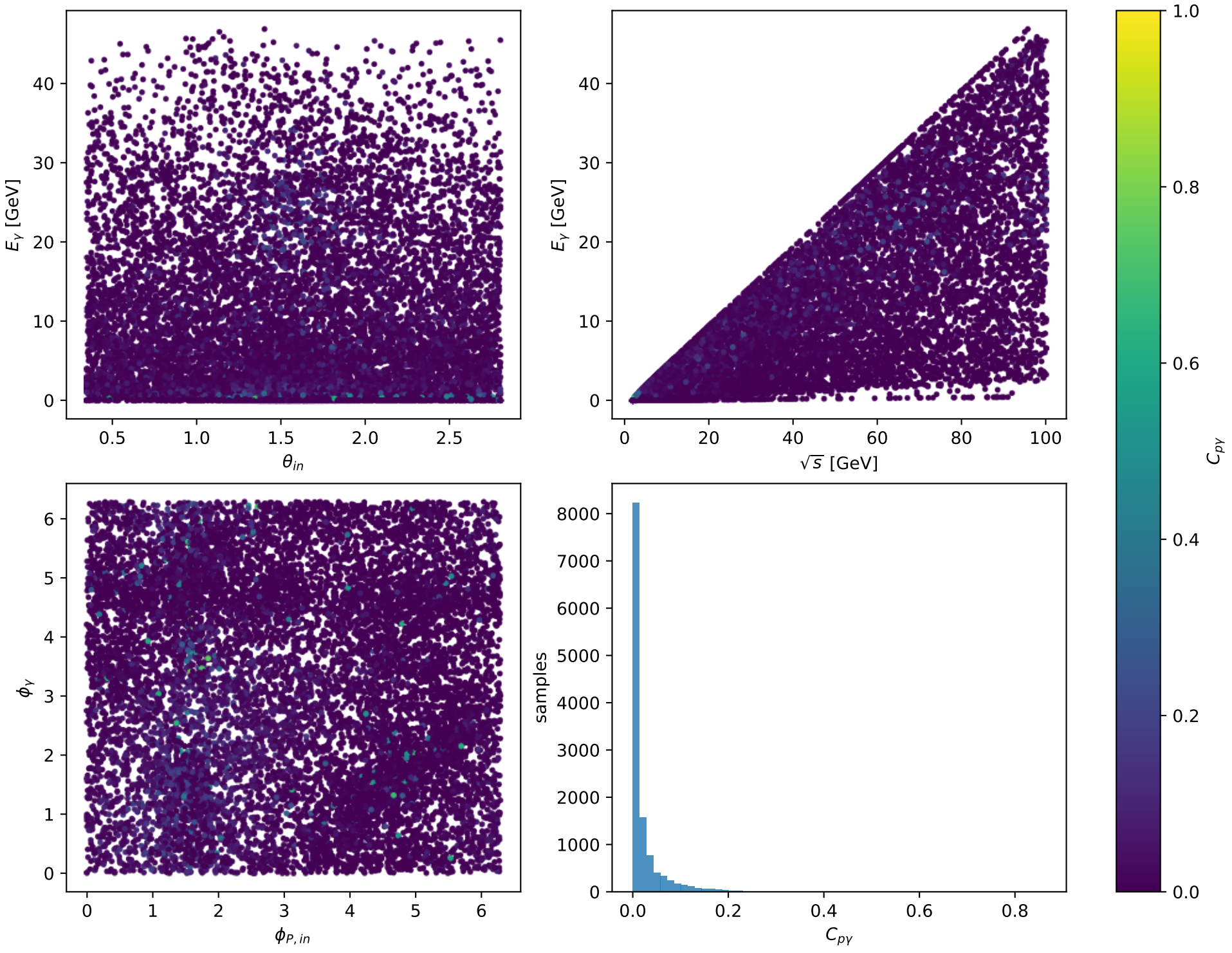
Phase-space scan: L auxiliary lepton + L proton [LL], max C_{p\gamma}=0.86431
