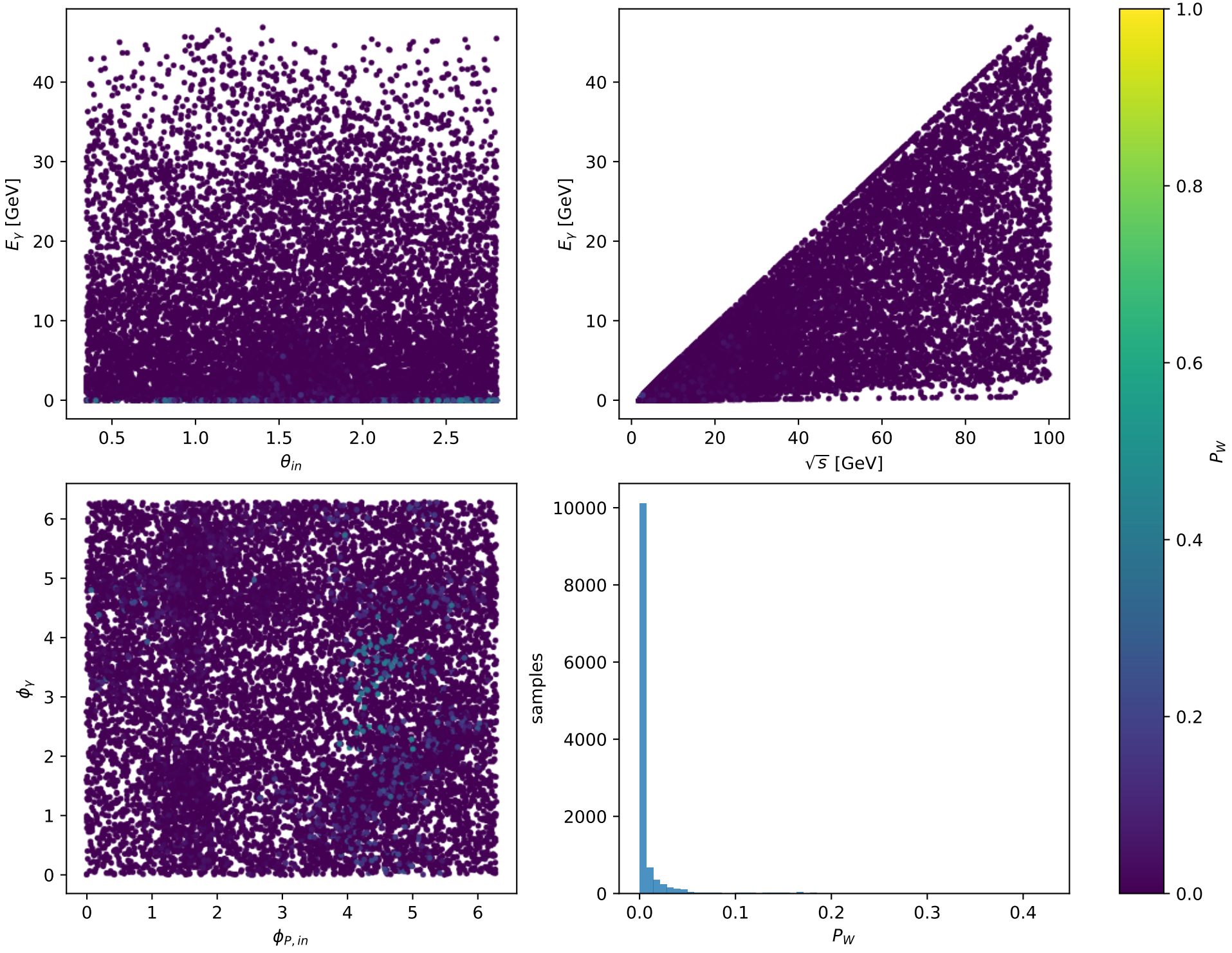
Phase-space scan: L auxiliary lepton + L proton [LL], max P_W=0.42693
