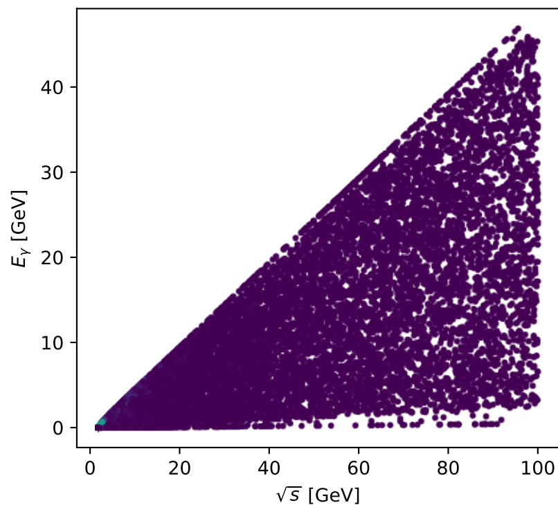
Phase-space scan: L auxiliary lepton + L proton [LL], max C_{lp}=0.91562
