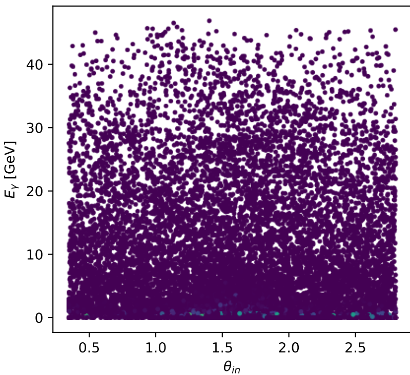
Phase-space scan: L auxiliary lepton+ L proton [LL], max F_3=0.84806
