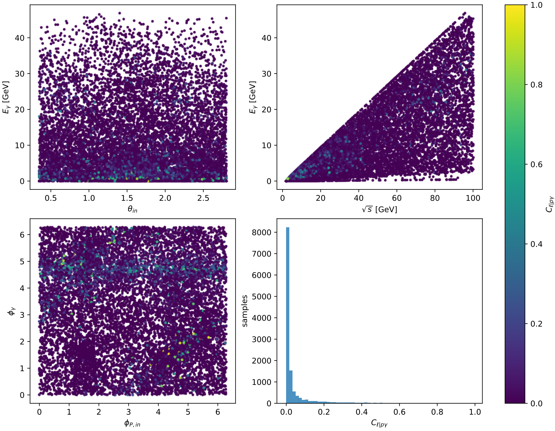
Phase-space scan: L auxiliary lepton + L proton [LL], max C_{\ell|p\gamma}=0.98975
