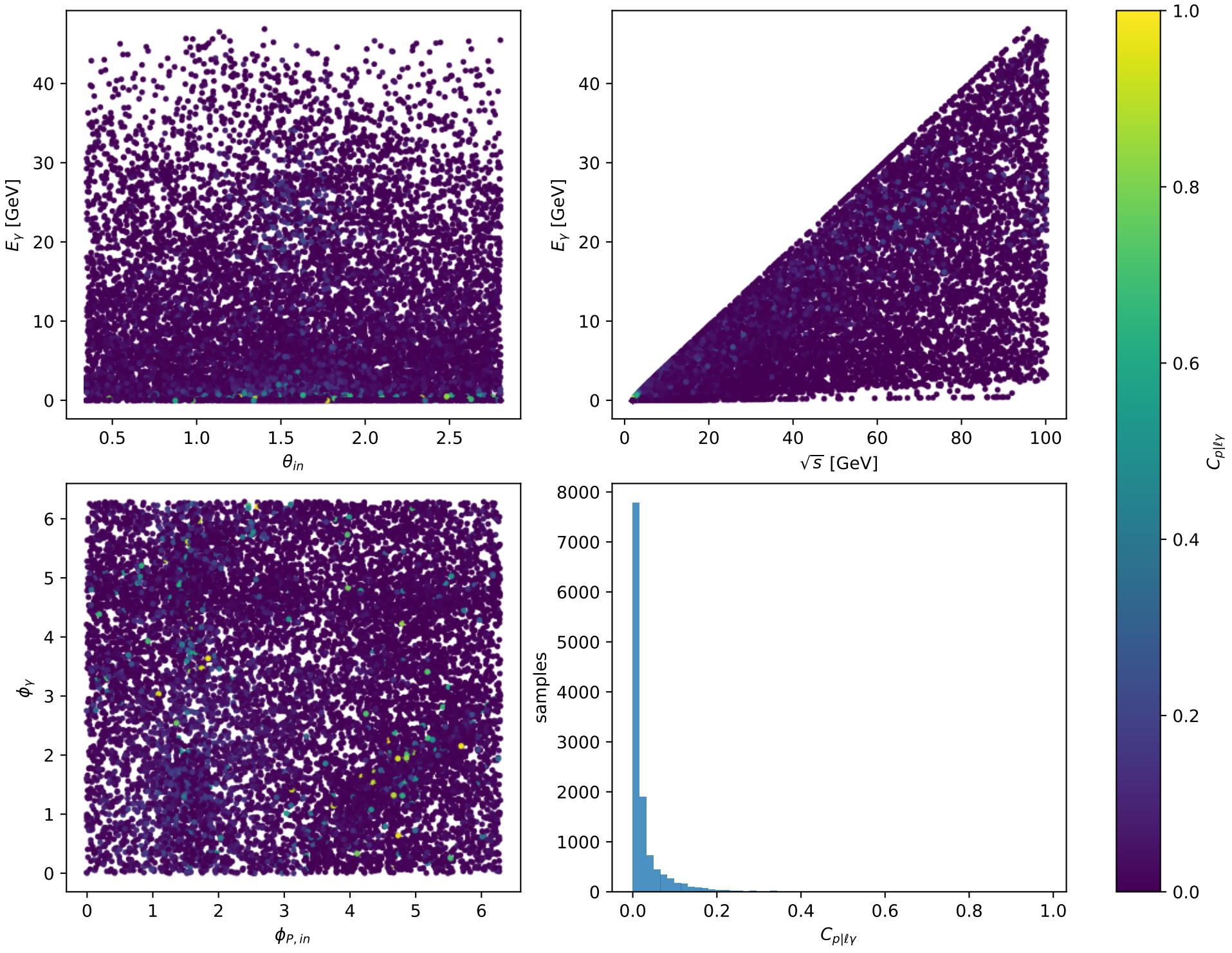
Phase-space scan: L auxiliary lepton + L proton [LL], max C_{p|l\gamma}=0.98208
