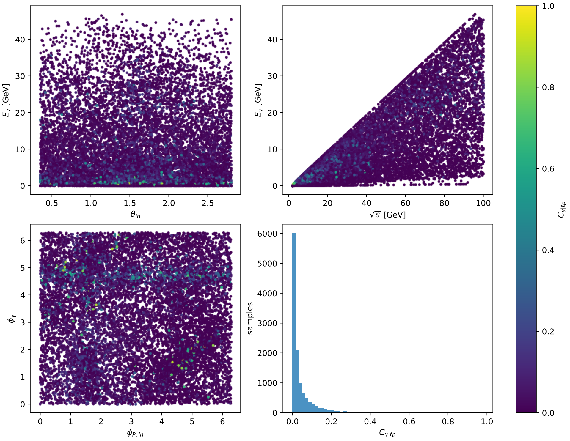
Phase-space scan: L auxiliary lepton + L proton [LL], max C_{\gamma lp}=0.98139
