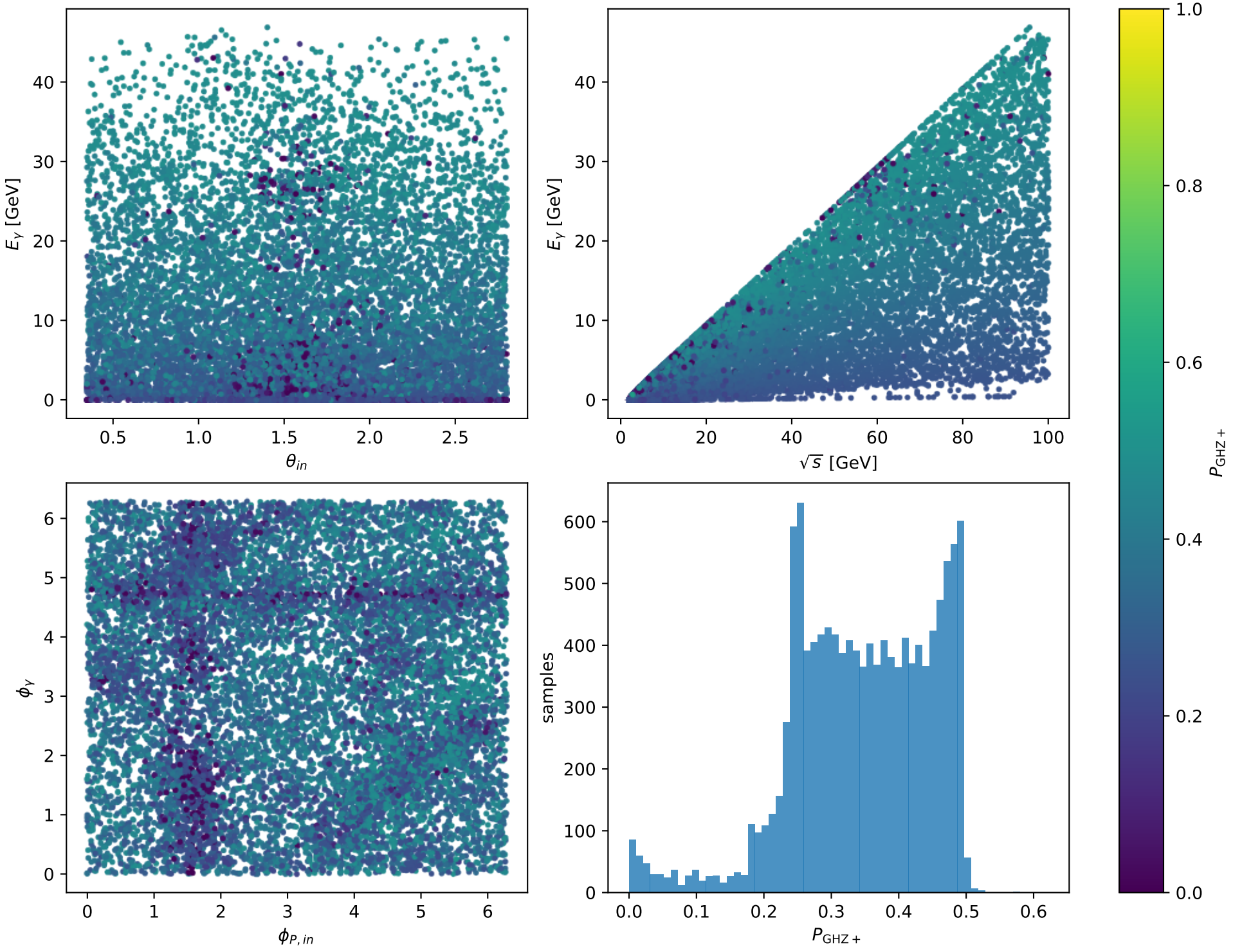
Phase-space scan: L auxiliary lepton + L proton [LL], max P_{\text{GHZ}+}=0.62168
