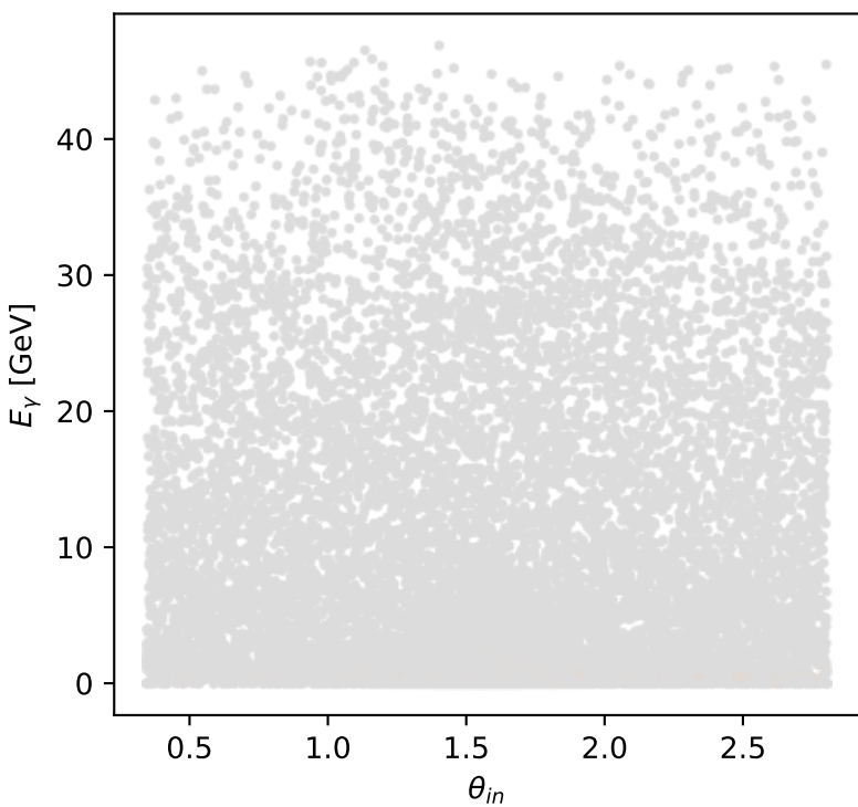
Phase-space scan: L auxiliary lepton + L proton [LL], max M_\gamma=0.15709
