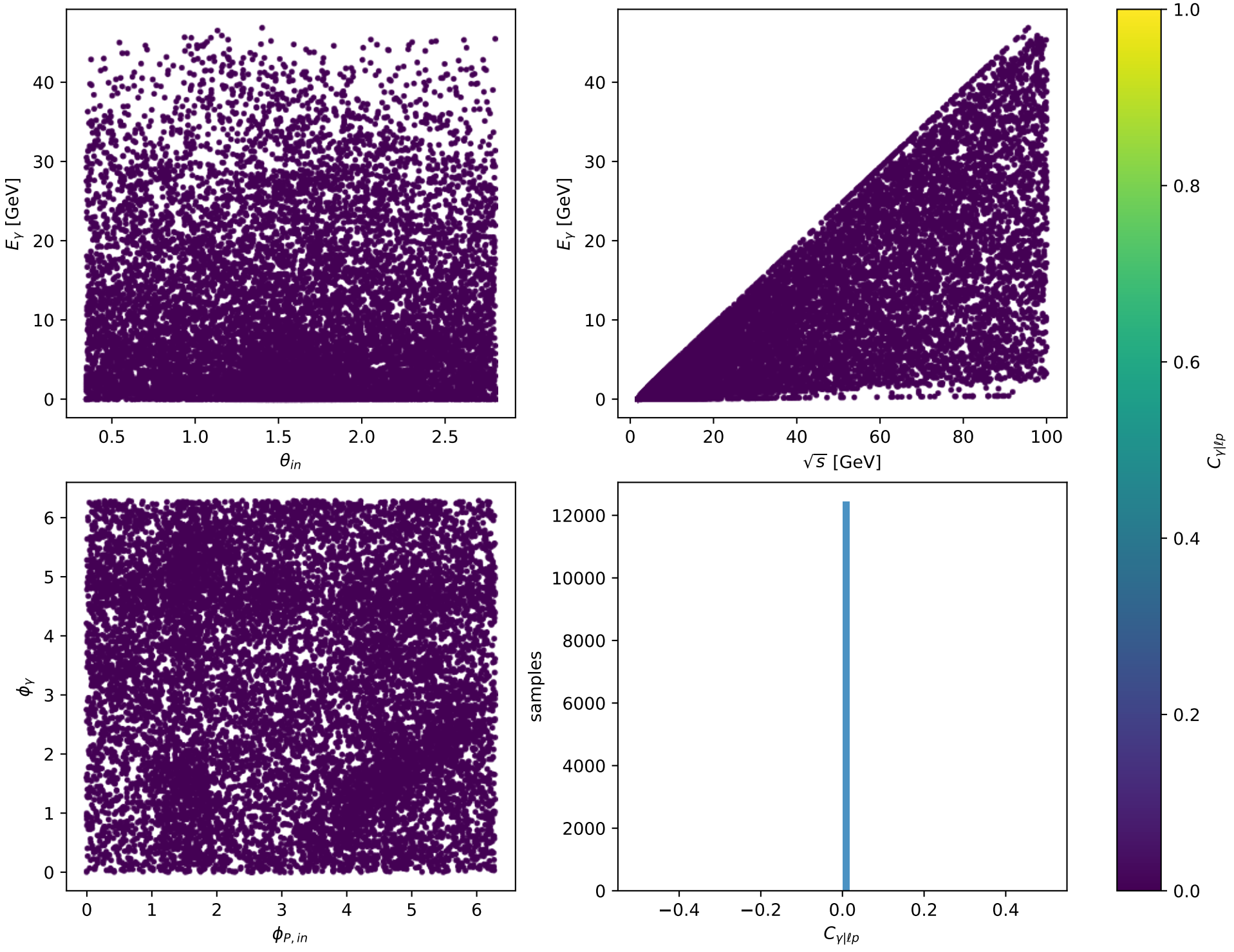
Phase-space scan: L auxiliary lepton [L_electron], max C_{\gamma|\ell p}=0
