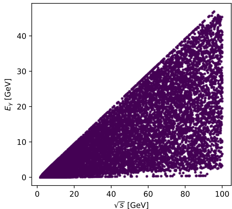
Phase-space scan: L auxiliary lepton [L_electron], max F_3=0
