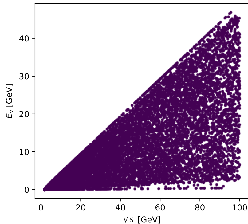
Phase-space scan: L auxiliary lepton [L_electron], max C_{p|\ell\gamma}=0
