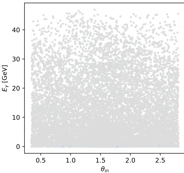
Phase-space scan: L auxiliary lepton [L_electron], max M_p=-0
