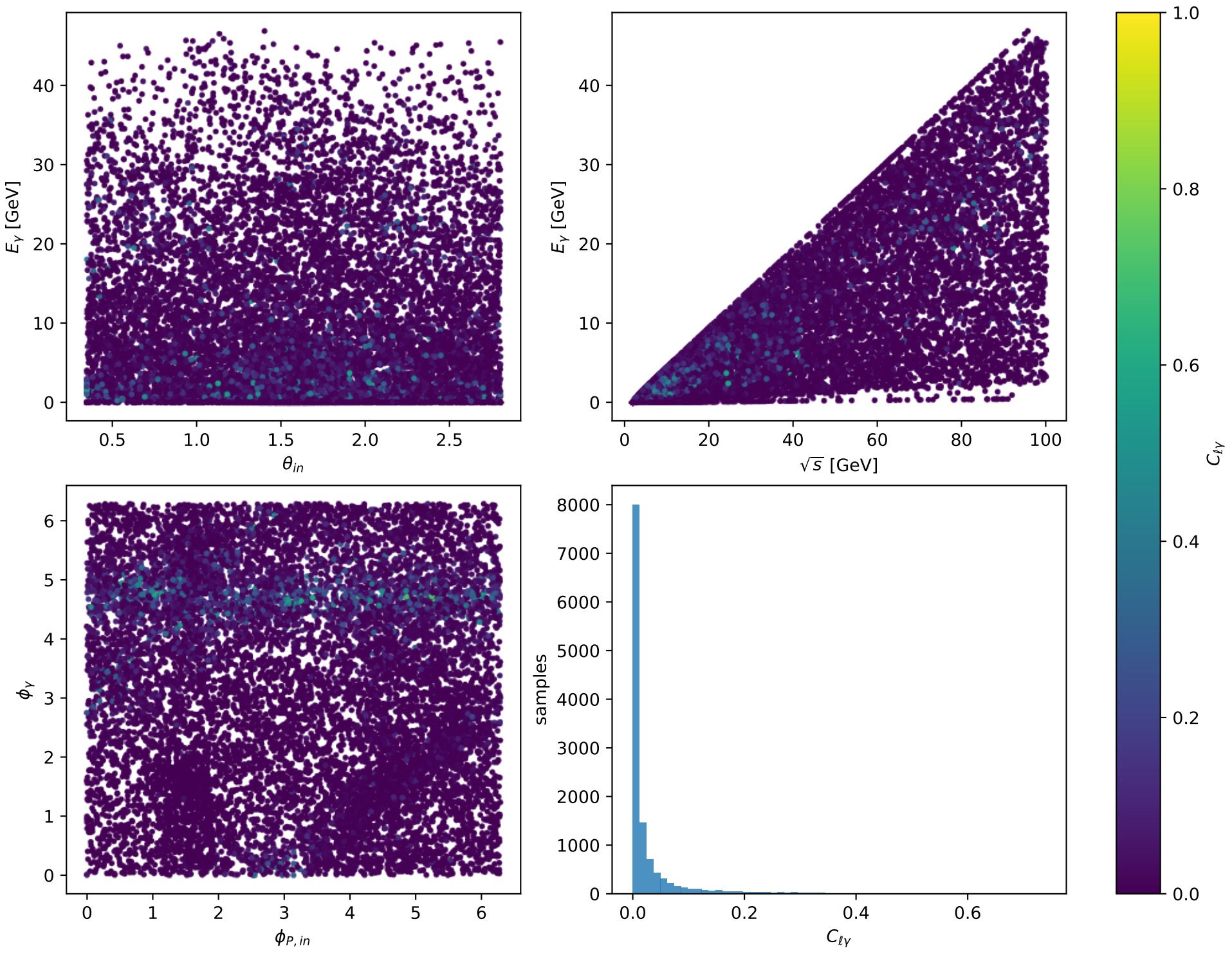
Phase-space scan: L auxiliary lepton [L_electron], max C_{\ell\gamma}=0.73974
