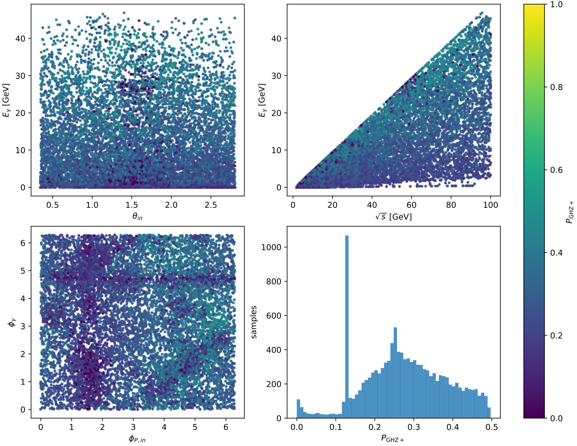
Phase-space scan: L auxiliary lepton [L_electron], max P_{\text{GHZ}+}=0.49703
