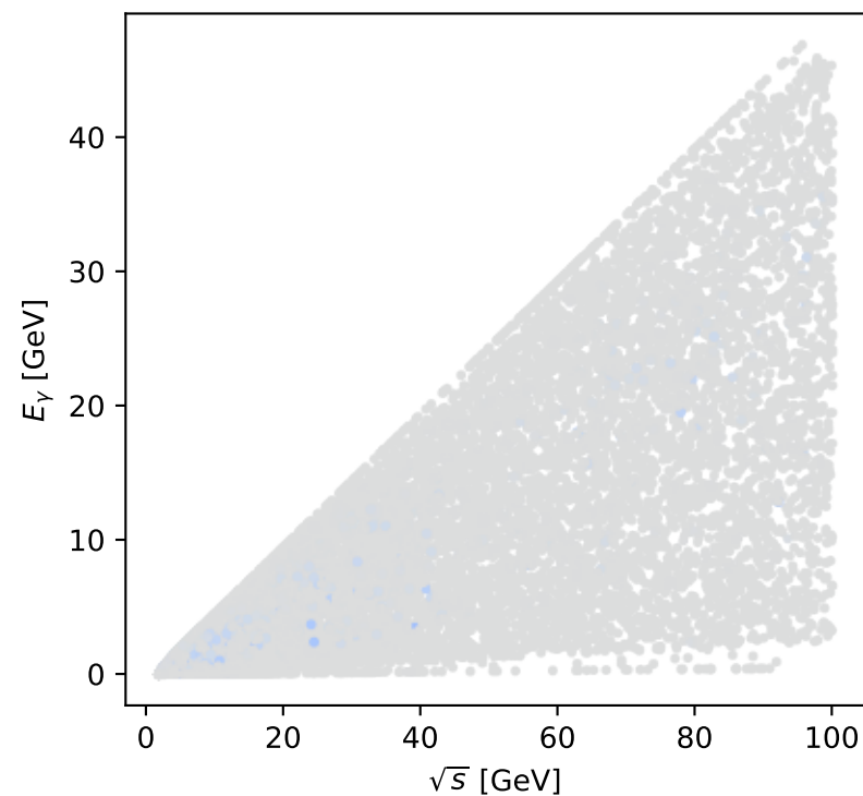
Phase-space scan: L auxiliary lepton [L_electron], max M_\gamma = -0
