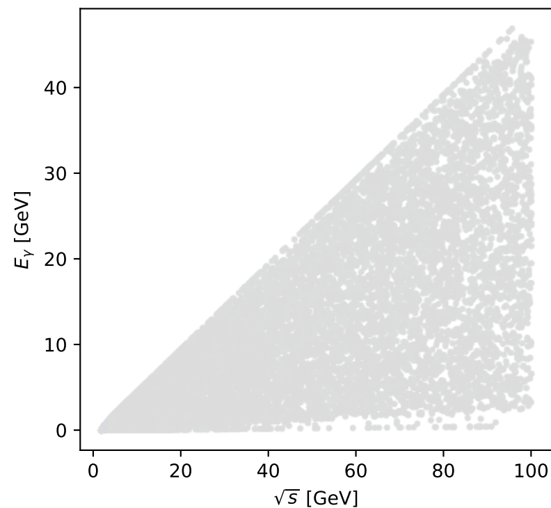
Phase-space scan: L auxiliary lepton [L_electron], max M_p=-0
