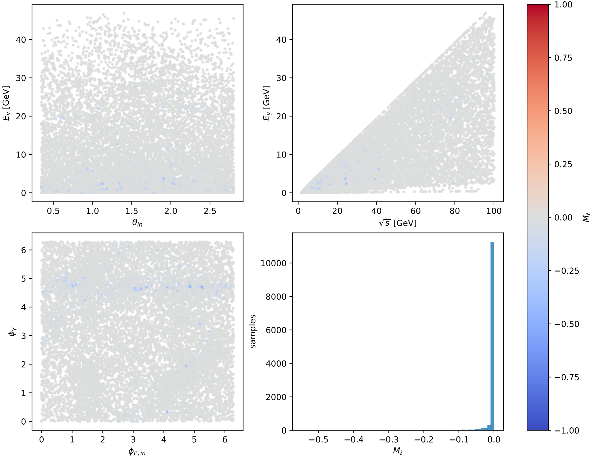
Phase-space scan: L auxiliary lepton [ L_{\text{electron}} ], max M_\ell = -5.3147\text{e-}17
