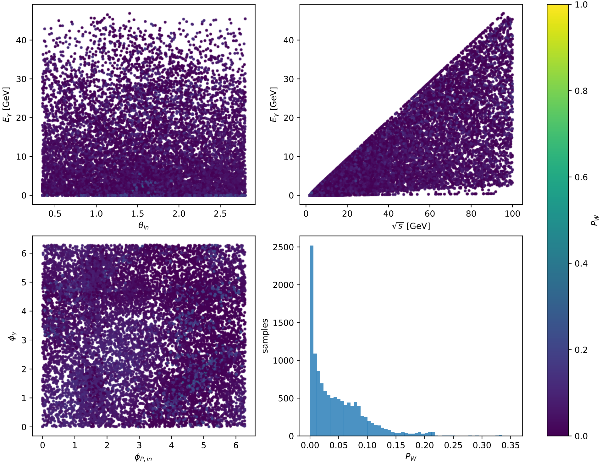
Phase-space scan: L auxiliary lepton [L_electron], max P_W=0.35313
