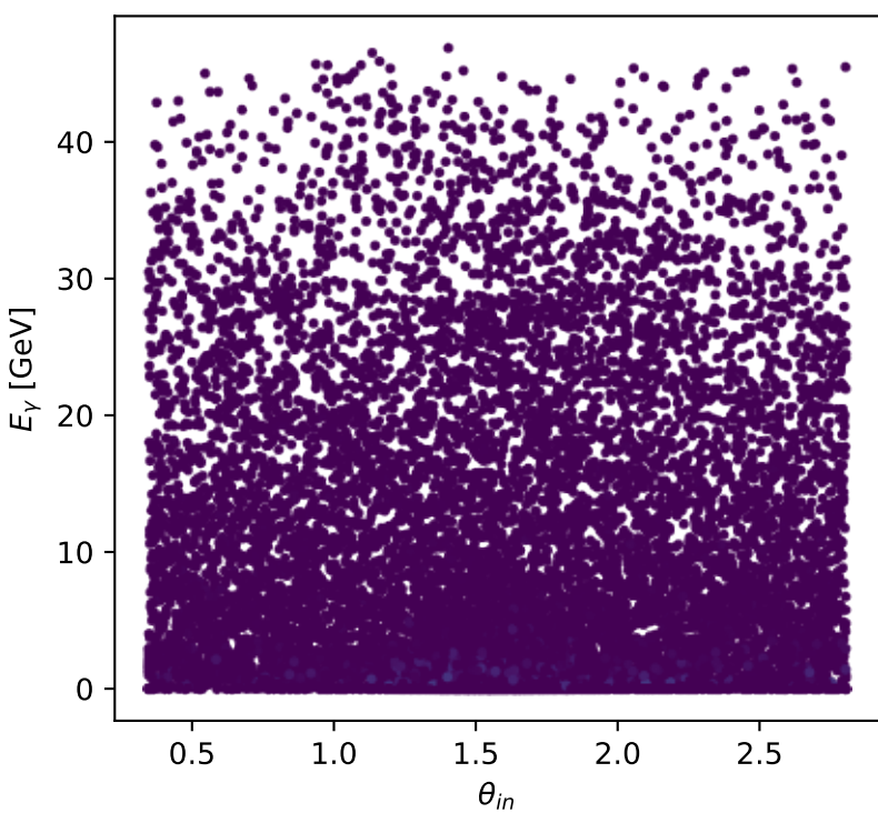
Phase-space scan: L auxiliary lepton [L_electron], max C_{p\gamma}=0.17107
