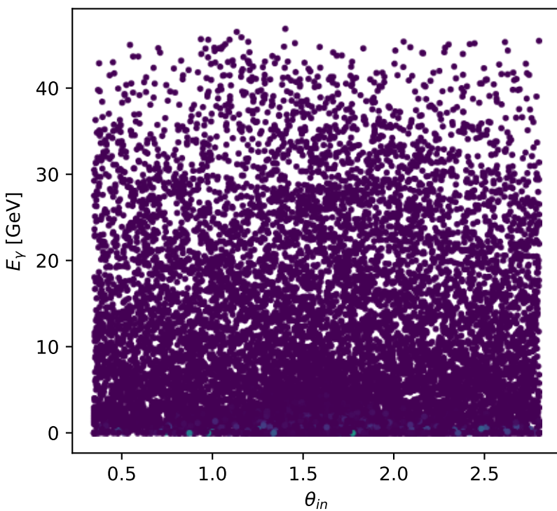
Phase-space scan: L auxiliary lepton [L_electron], max C_{lp}=0.62449
