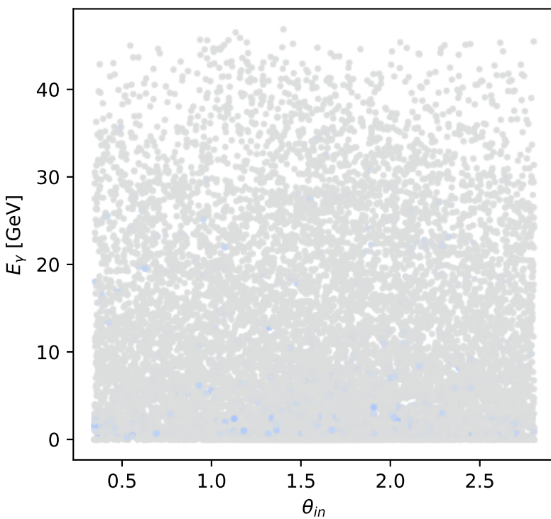
Phase-space scan: L auxiliary lepton [L_electron], max M_\gamma = -0
