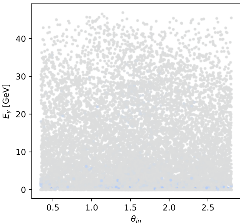
Phase-space scan: L proton [L_proton], max M_\gamma = -0
