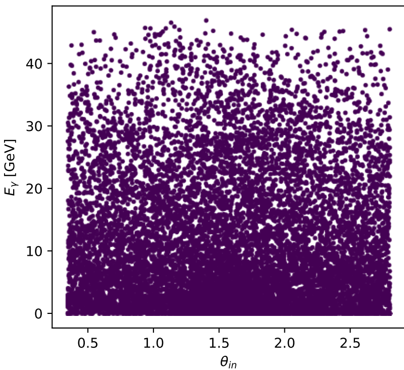
Phase-space scan: L proton [L_proton], max F_3=0
