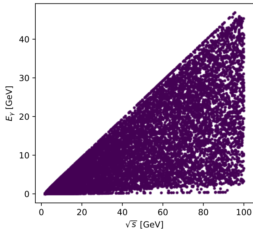
Phase-space scan: L proton [L_proton], max C_{p|\ell\gamma}=0
