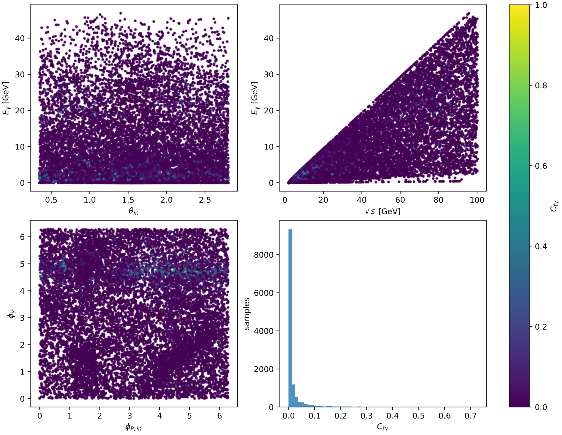
Phase-space scan: L proton [L_proton], max C_{\ell\gamma}=0.7245
