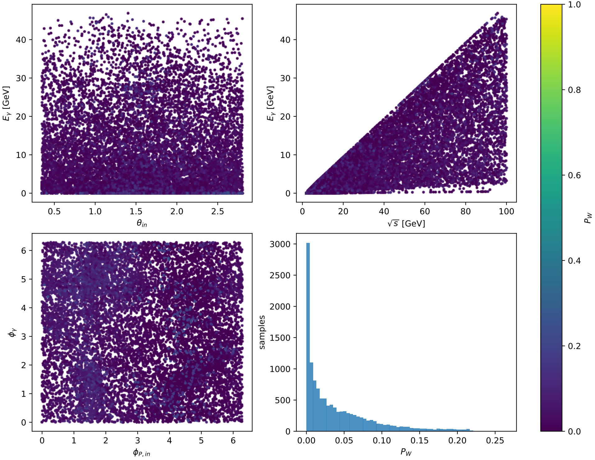
Phase-space scan: L proton [L_proton], max P_W=0.26503
