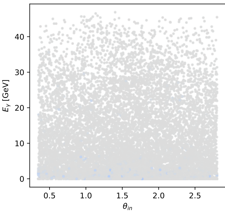
Phase-space scan: L proton [L_proton], max M_\ell = -0
