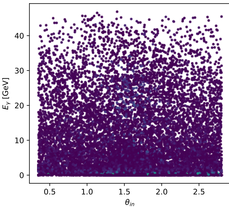
Phase-space scan: L proton [L_proton], max C_{p\gamma}=0.8154
