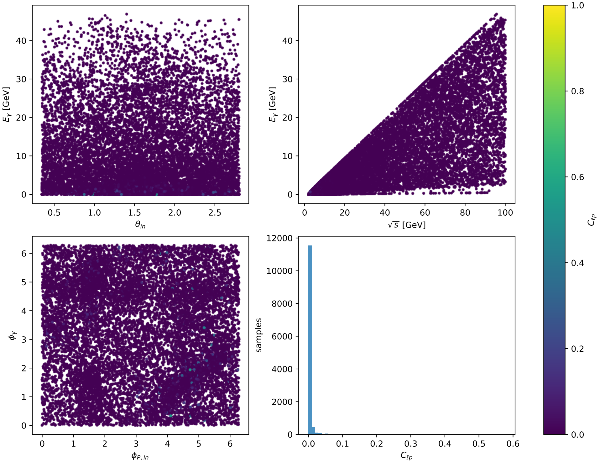
Phase-space scan: L proton [L_proton], max C_{lp}=0.57717
