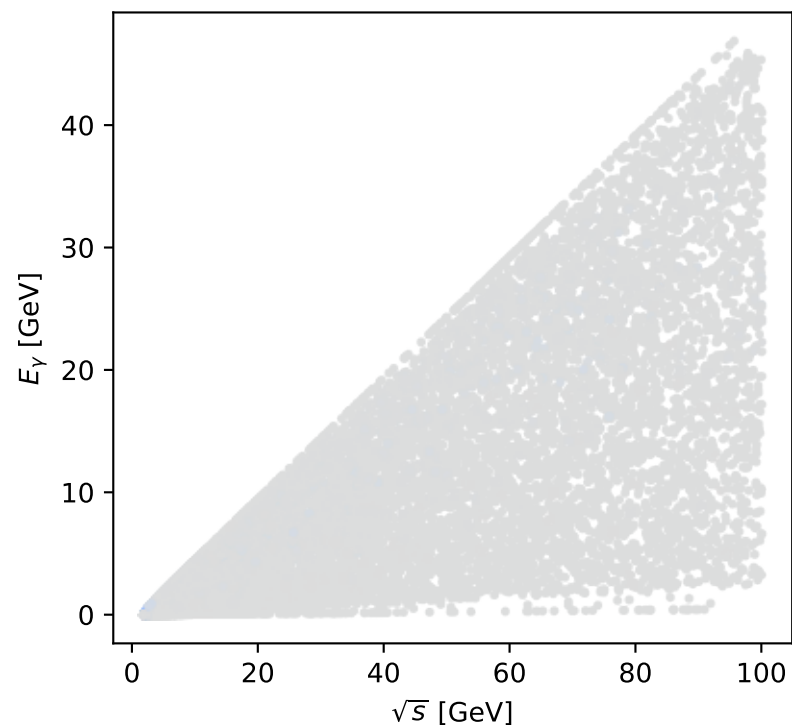
Phase-space scan: L proton [L_proton], max M_p=-0
