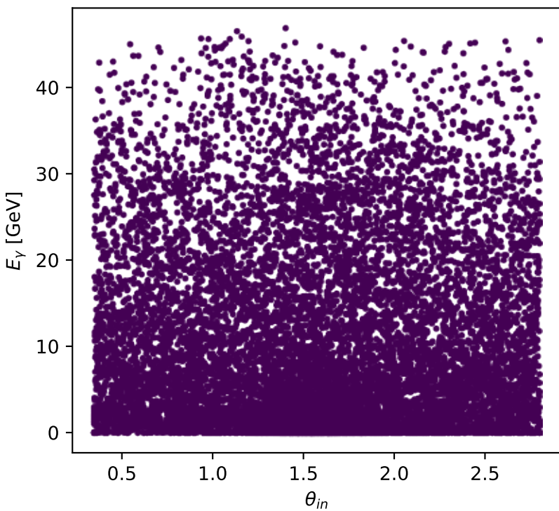
Phase-space scan: L proton [L_proton], max C_{p|\ell\gamma}=0
