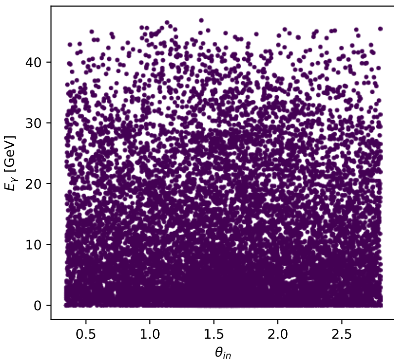
Phase-space scan: L proton [L_proton], max C_{\gamma|\ell p}=0
