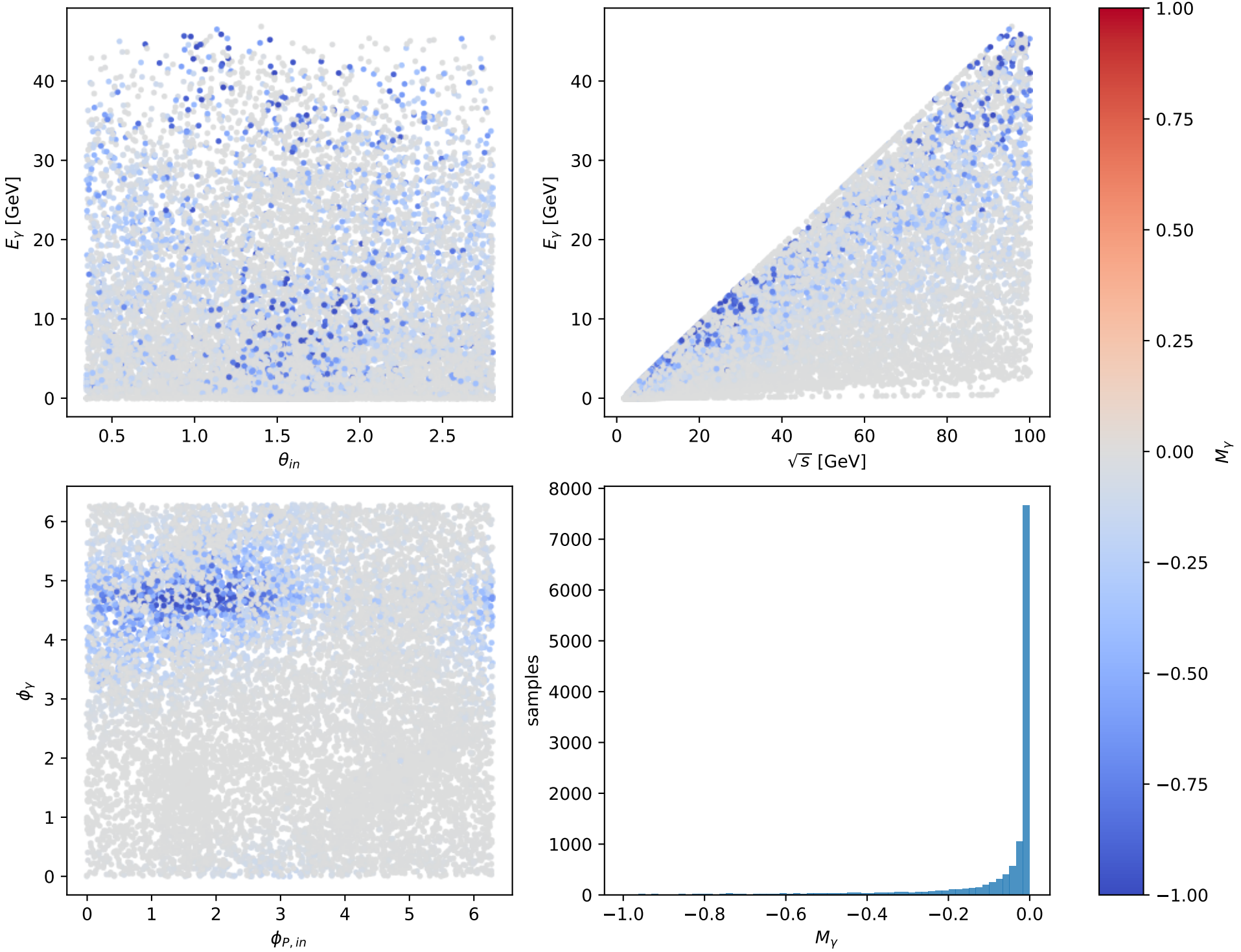
Phase-space scan: Tx auxiliary lepton [Tx_electron], max M_Y = -8.1158\text{e-}26
