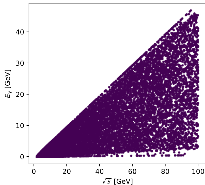
Phase-space scan: Tx auxiliary lepton [Tx_electron], max C_{p|\ell\gamma}=0
