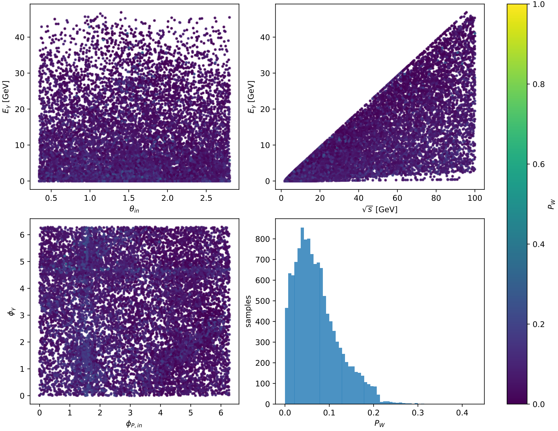
Phase-space scan: Tx auxiliary lepton [Tx_electron], max P_W=0.42857
