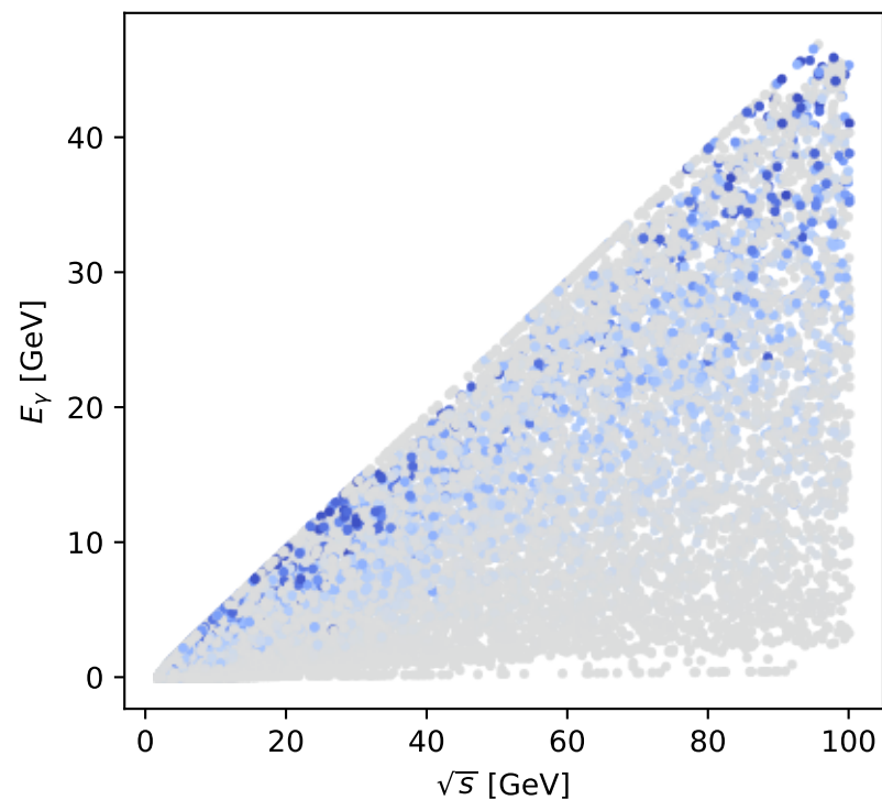
Phase-space scan: Tx auxiliary lepton [Tx_electron], max M_\ell = -0
