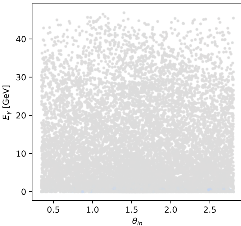
Phase-space scan: Tx auxiliary lepton [Tx_electron], max M_p = -0
