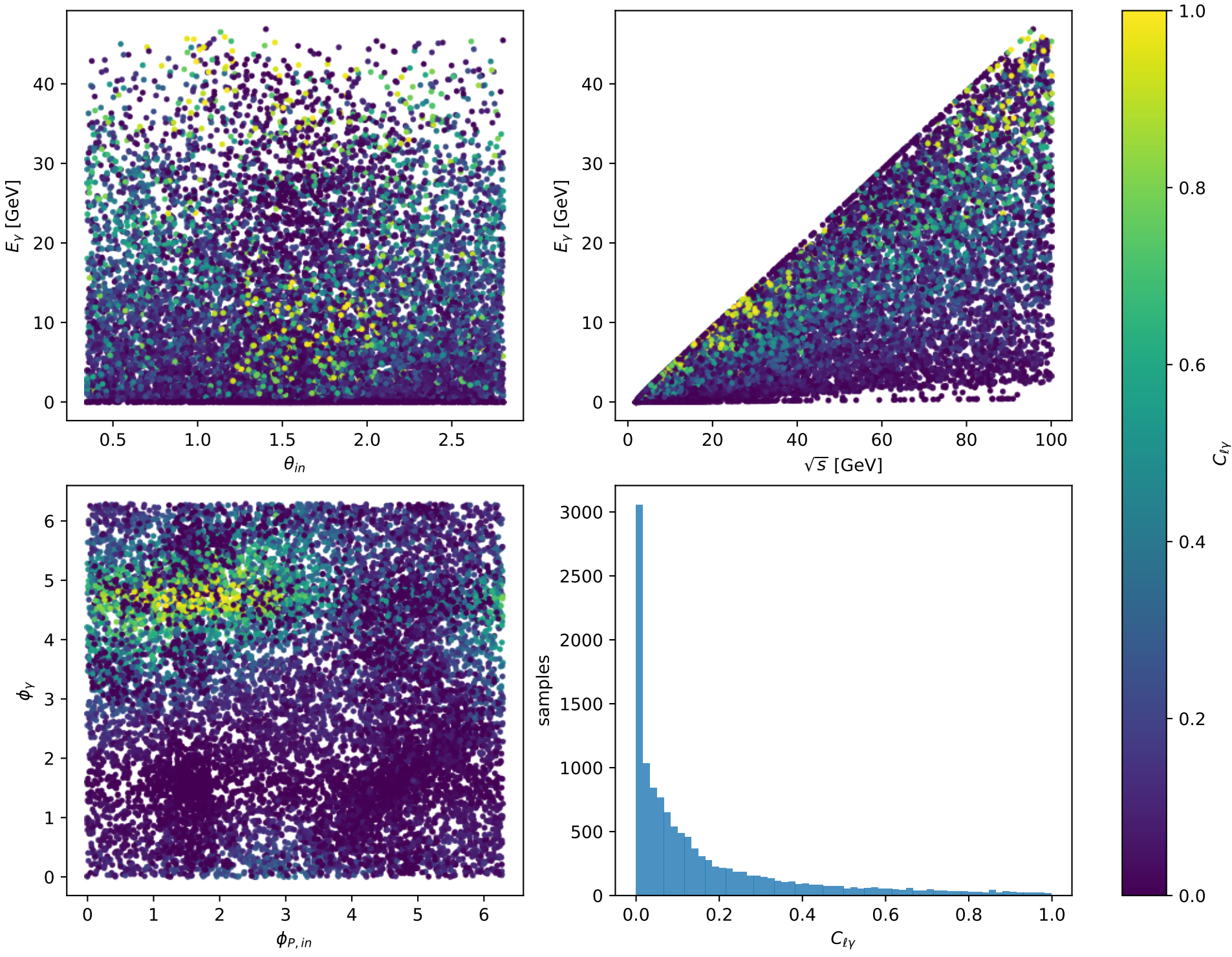
Phase-space scan: Tx auxiliary lepton [Tx_electron], max C_{\ell\gamma}=0.99815
