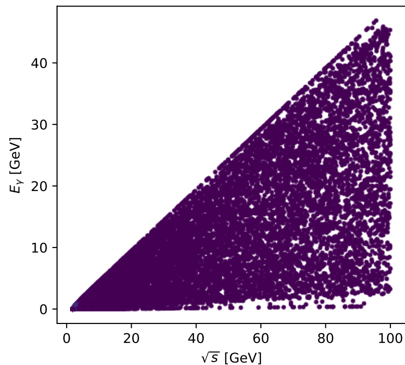
Phase-space scan: Tx auxiliary lepton [Tx_electron], max C_{lp}=0.50078
