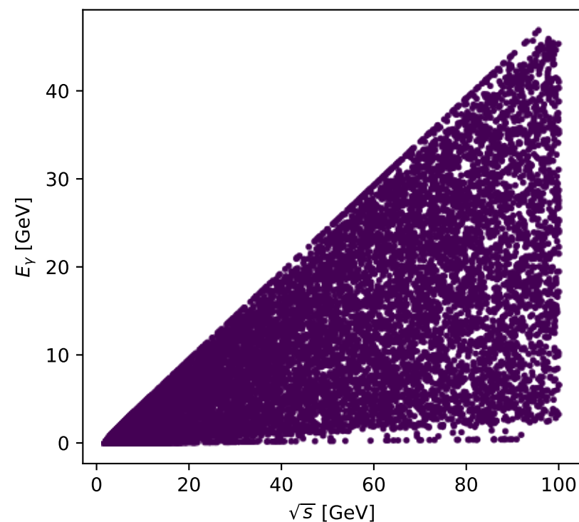
Phase-space scan: Tx auxiliary lepton [Tx_electron], max F_3=0
