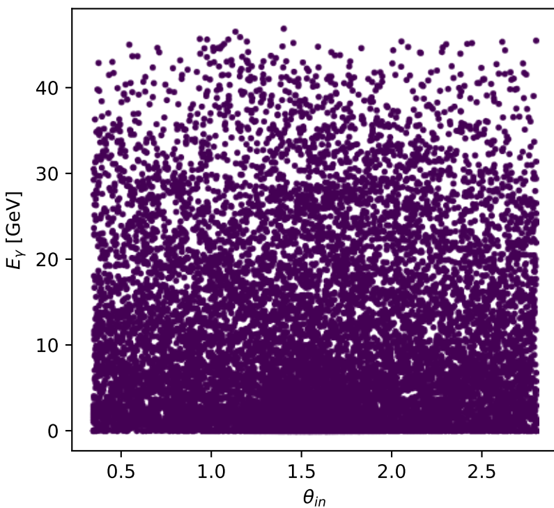
Phase-space scan: Tx auxiliary lepton [Tx_electron], max C_{\gamma|\ell p}=0
