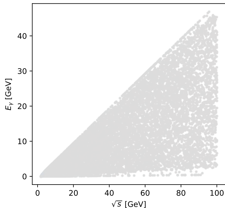
Phase-space scan: Tx auxiliary lepton [Tx_electron], max M_p = -0
