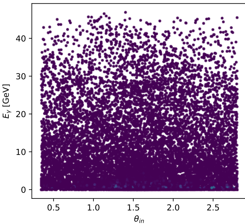
Phase-space scan: Tx auxiliary lepton [Tx_electron], max C_{p\gamma}=0.34849
