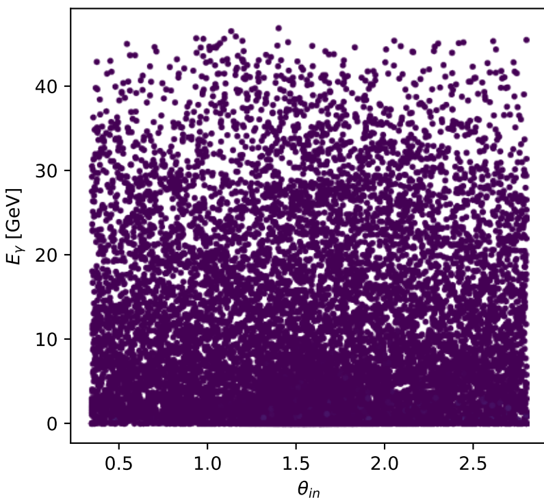
Phase-space scan: Tx proton [Tx_proton], max C_{\ell\gamma}=0.1779
