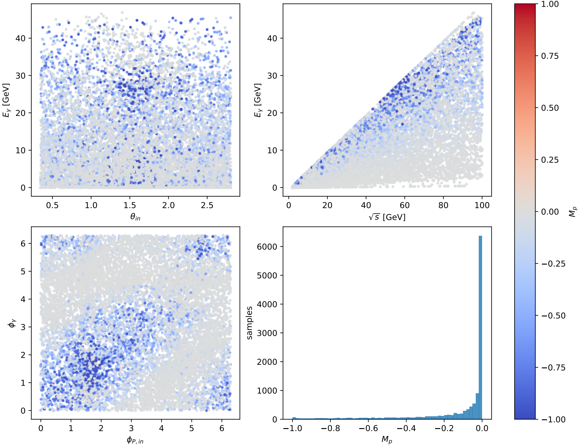
Phase-space scan: Tx proton [Tx_proton], max M_p = -0
