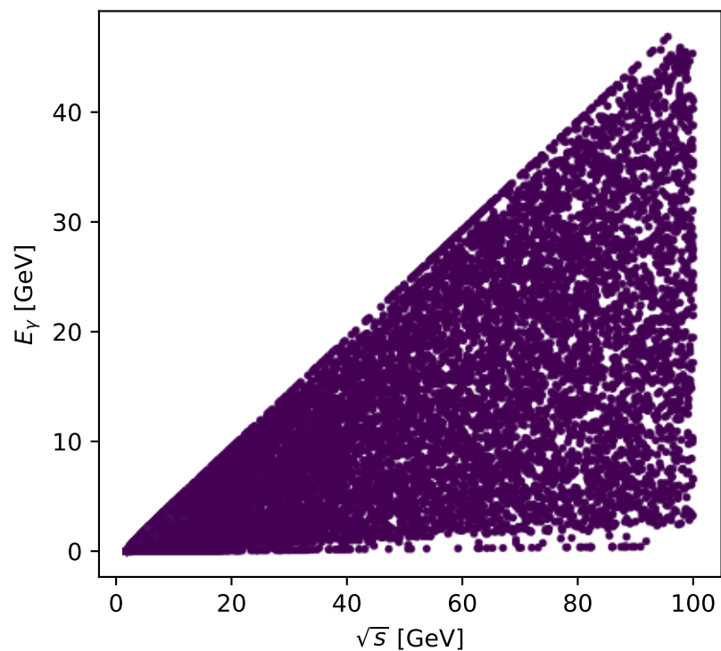
Phase-space scan: Tx proton [Tx_proton], max C_{\ell\gamma}=0.1779
