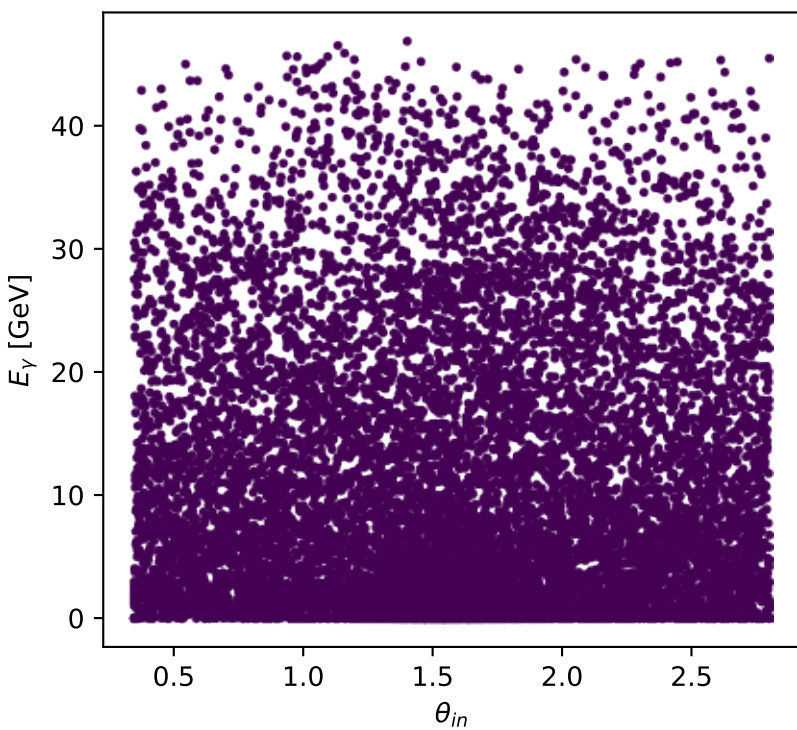
Phase-space scan: Tx proton [Tx_proton], max C_{p|l\gamma}=0
