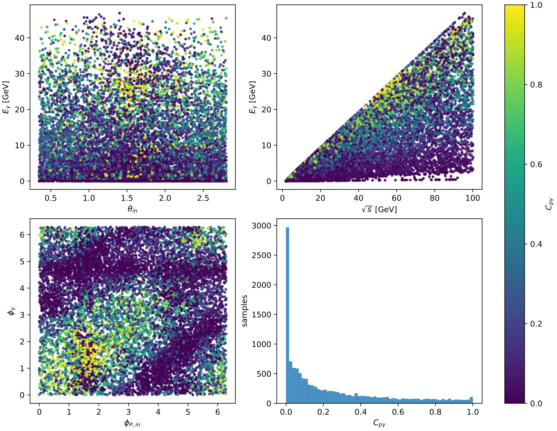
Phase-space scan: Tx proton [Tx_proton], max C_{p\gamma}=0.99998
