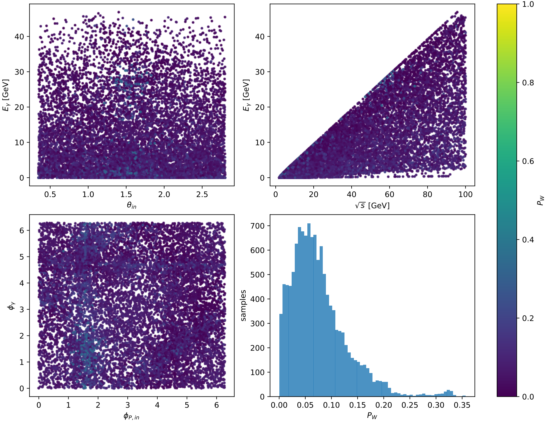
Phase-space scan: Tx proton [Tx_proton], max P_W=0.35646
