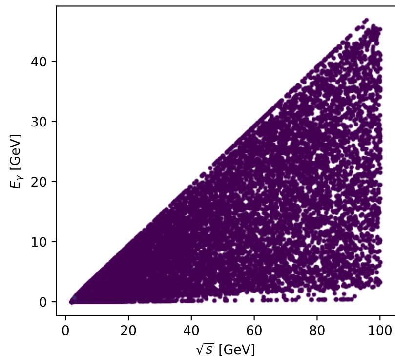
Phase-space scan: Tx proton [Tx_proton], max C_{lp}=0.58402
