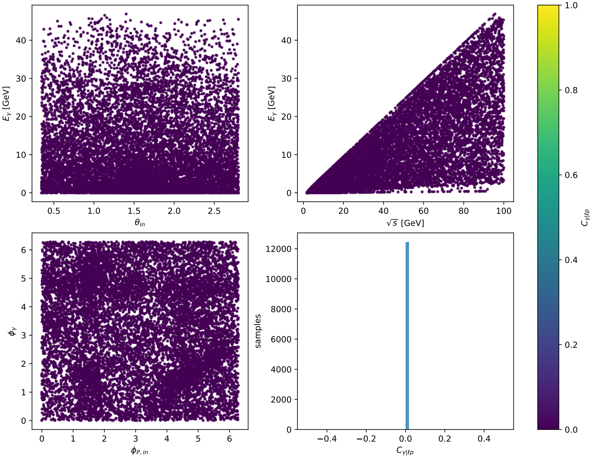
Phase-space scan: Tx proton [Tx_proton], max C_{\gamma|lp}=0
