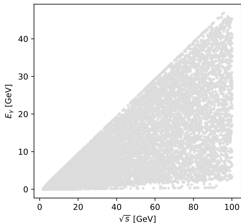
Phase-space scan: Tx proton [Tx_proton], max M_\ell = -0
