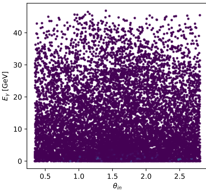
Phase-space scan: Tx proton [Tx_proton], max C_{lp}=0.58402
