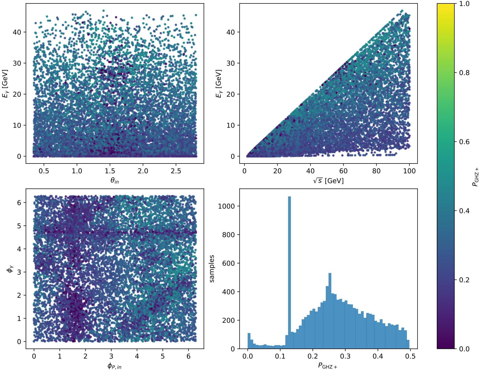
Phase-space scan: Tx proton [Tx_proton], max P_{\text{GHZ}+}=0.49703
