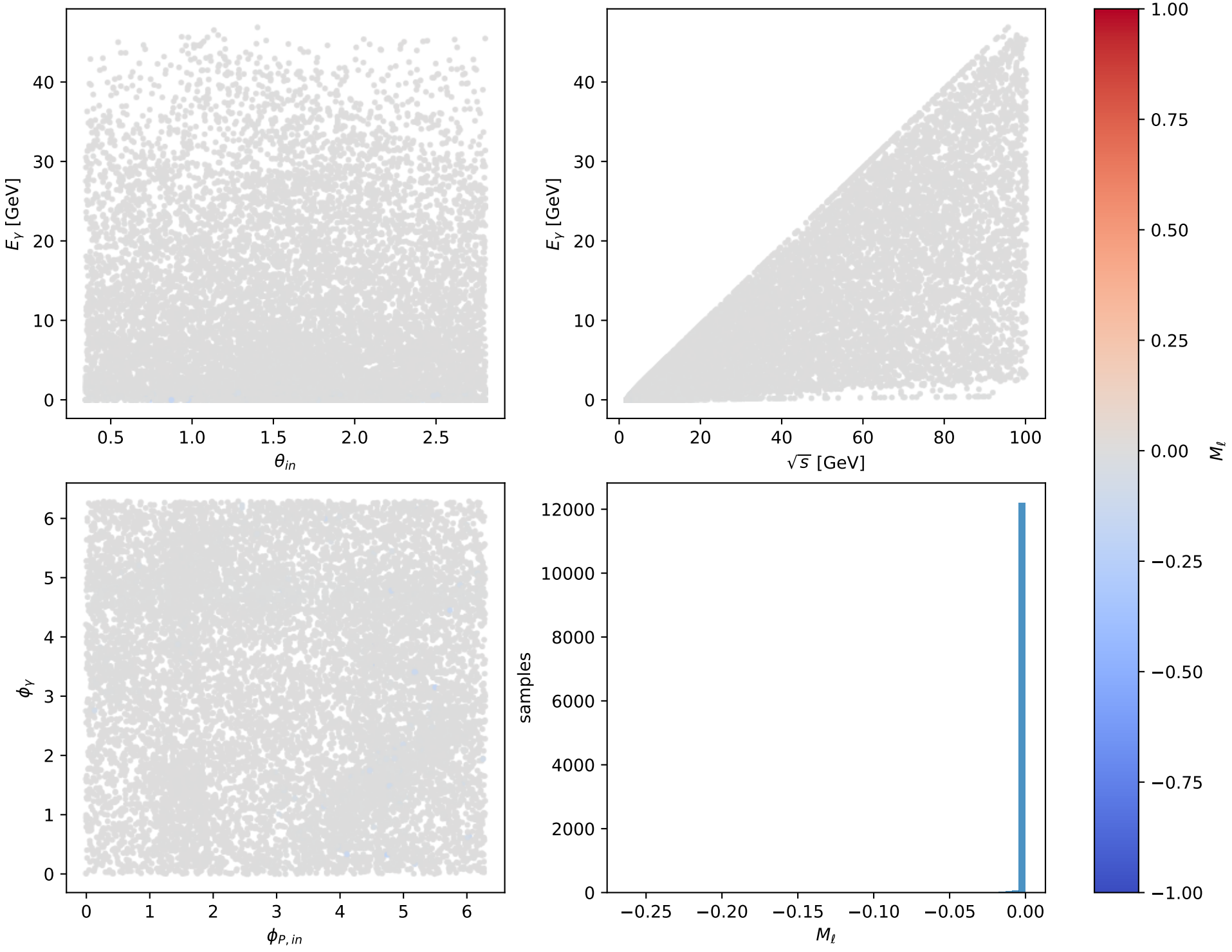
Phase-space scan: Ty proton [Ty_proton], max M_\ell=-0
