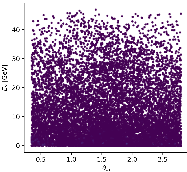
Phase-space scan: Ty proton [Ty_proton], max C_{\ell\gamma}=0.20796
