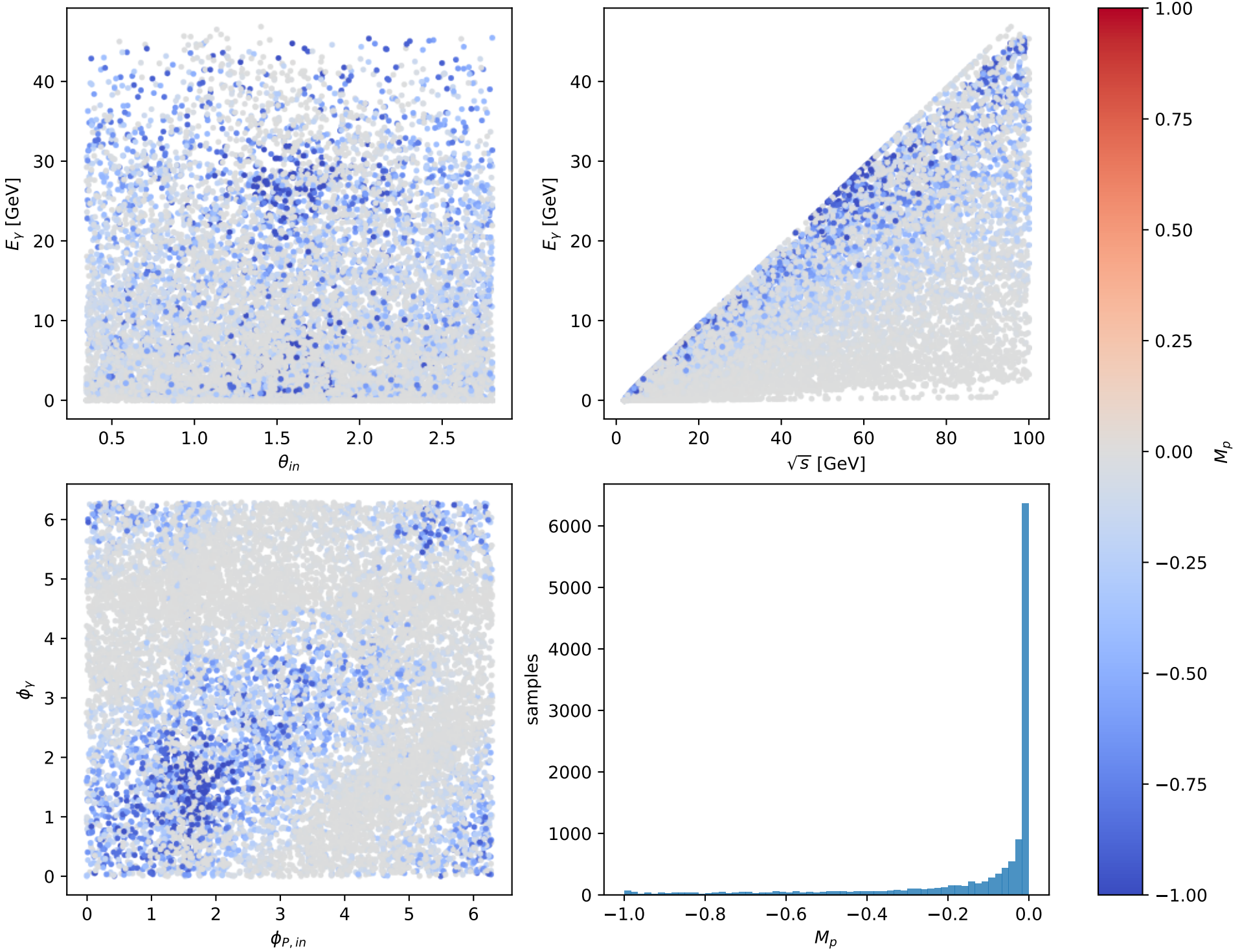
Phase-space scan: Ty proton [Ty_proton], max M_p=-0
