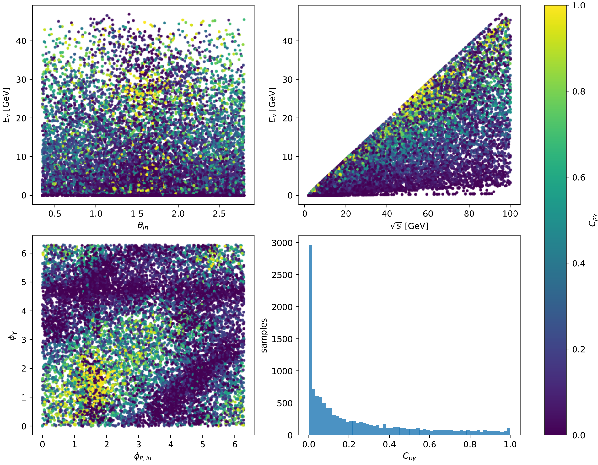
Phase-space scan: Ty proton [Ty_proton], max C_{p\gamma}=0.99998
