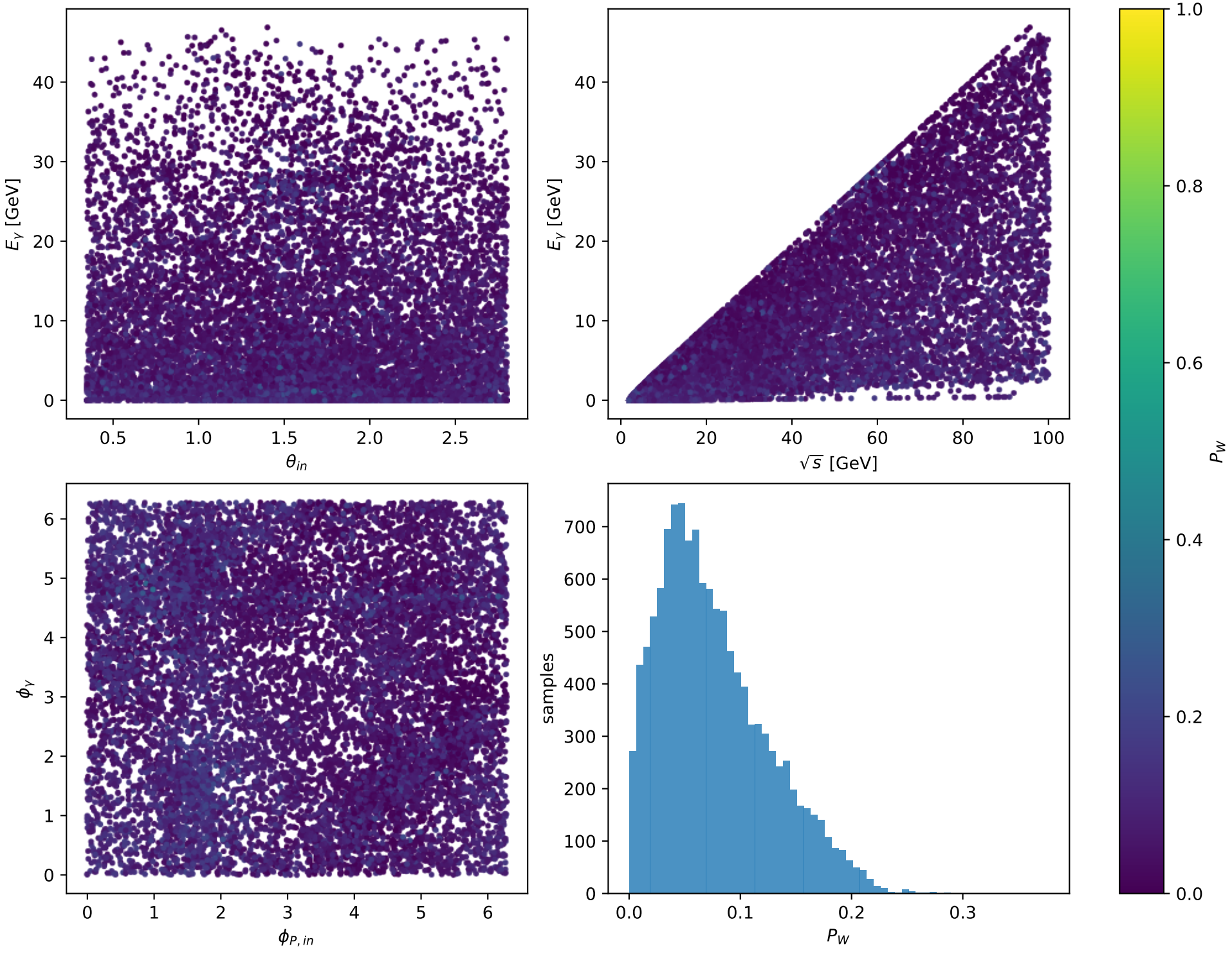
Phase-space scan: Ty proton [Ty_proton], max P_W=0.37703
