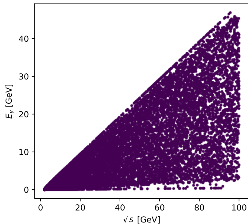
Phase-space scan: Ty proton [Ty_proton], max C_{\ell|p\gamma}=0
