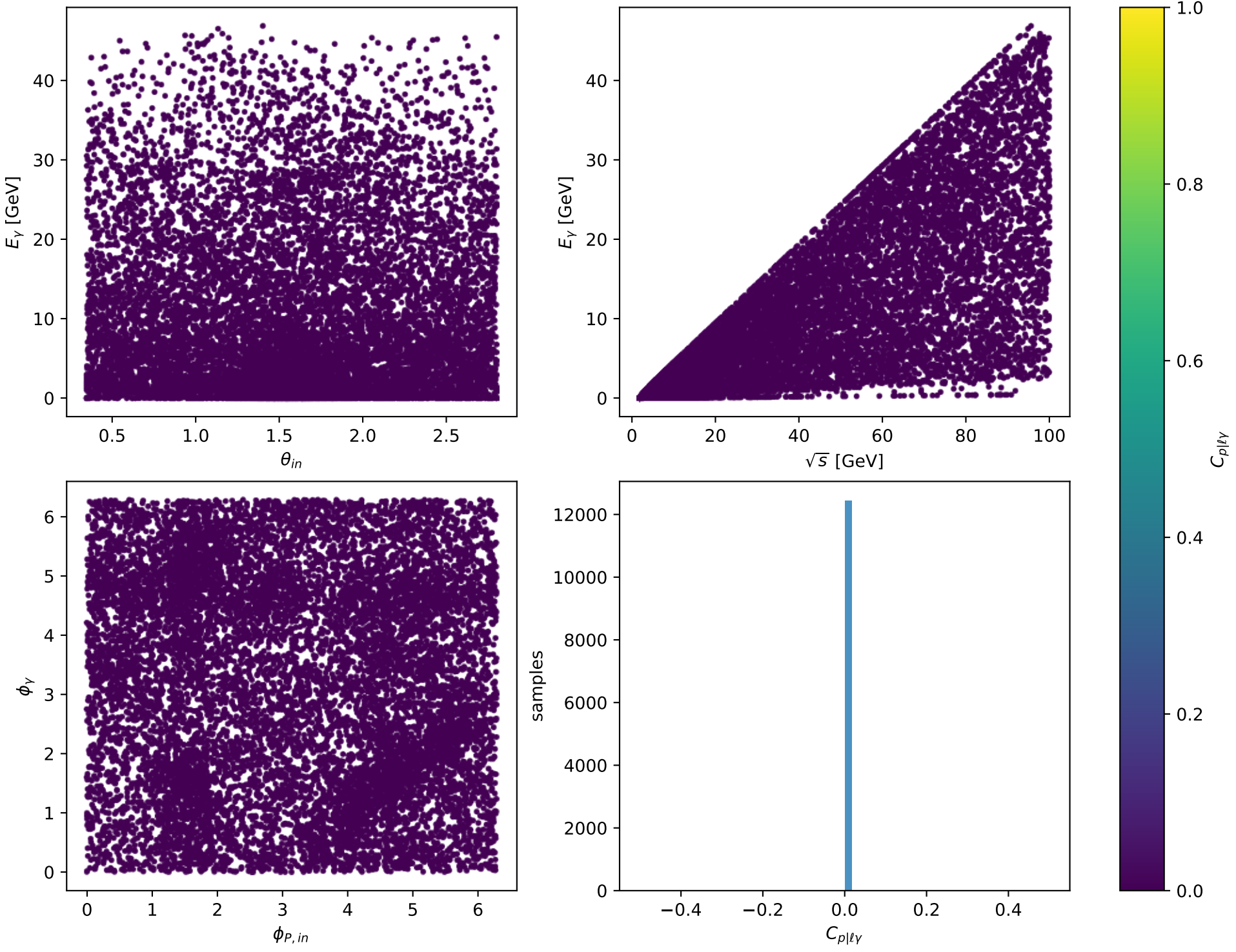
Phase-space scan: Ty proton [Ty_proton], max C_{p|l\gamma}=0
