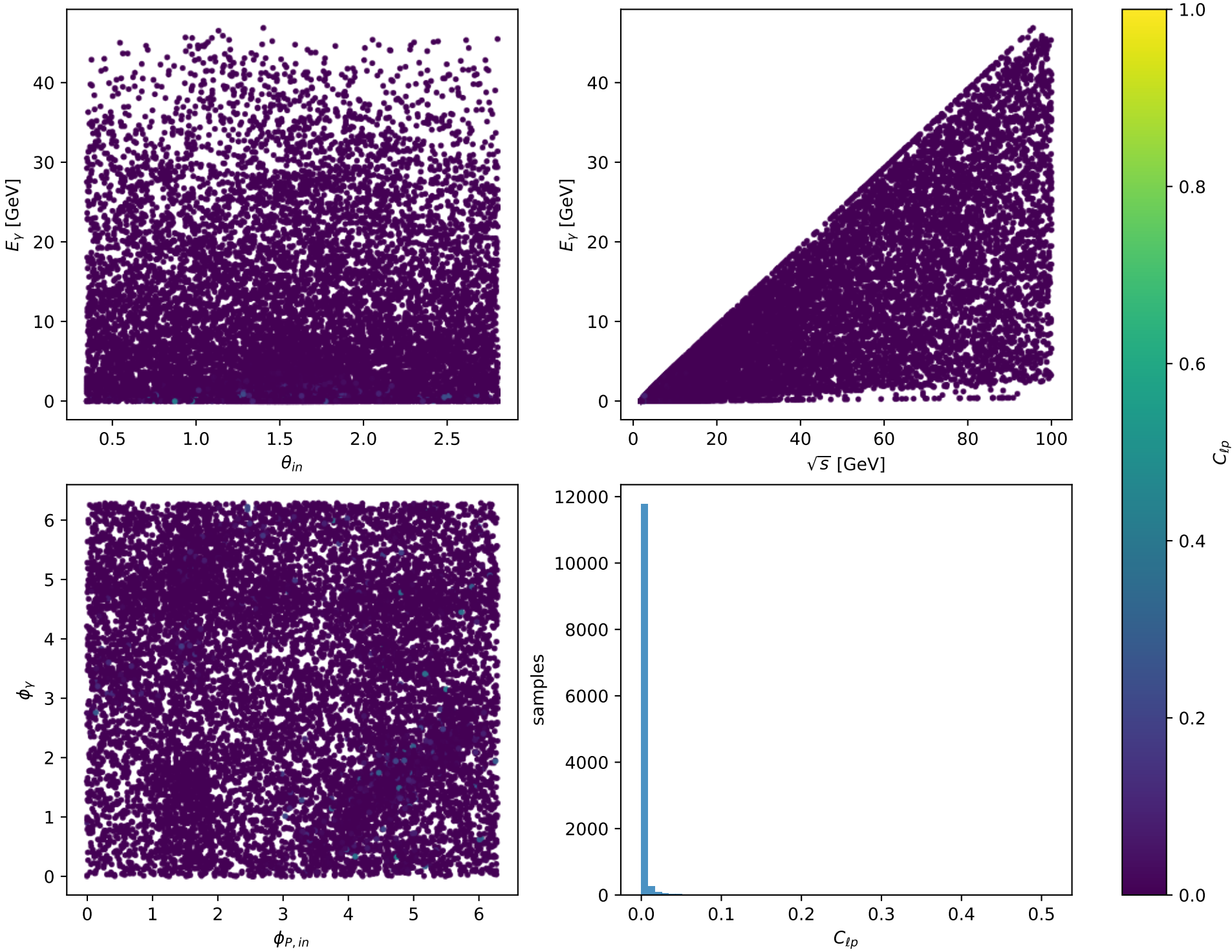
Phase-space scan: Ty proton [Ty_proton], max C_{lp}=0.51238
