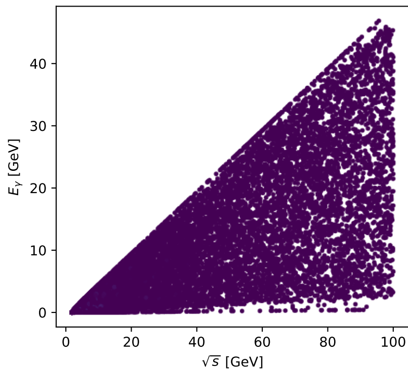
Phase-space scan: Ty proton [Ty_proton], max C_{\ell\gamma}=0.20796
