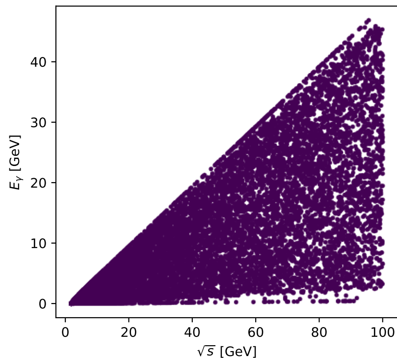
Phase-space scan: Unpolarized [unpolarized], max C_{p\gamma}=1.5829\text{e-}11
