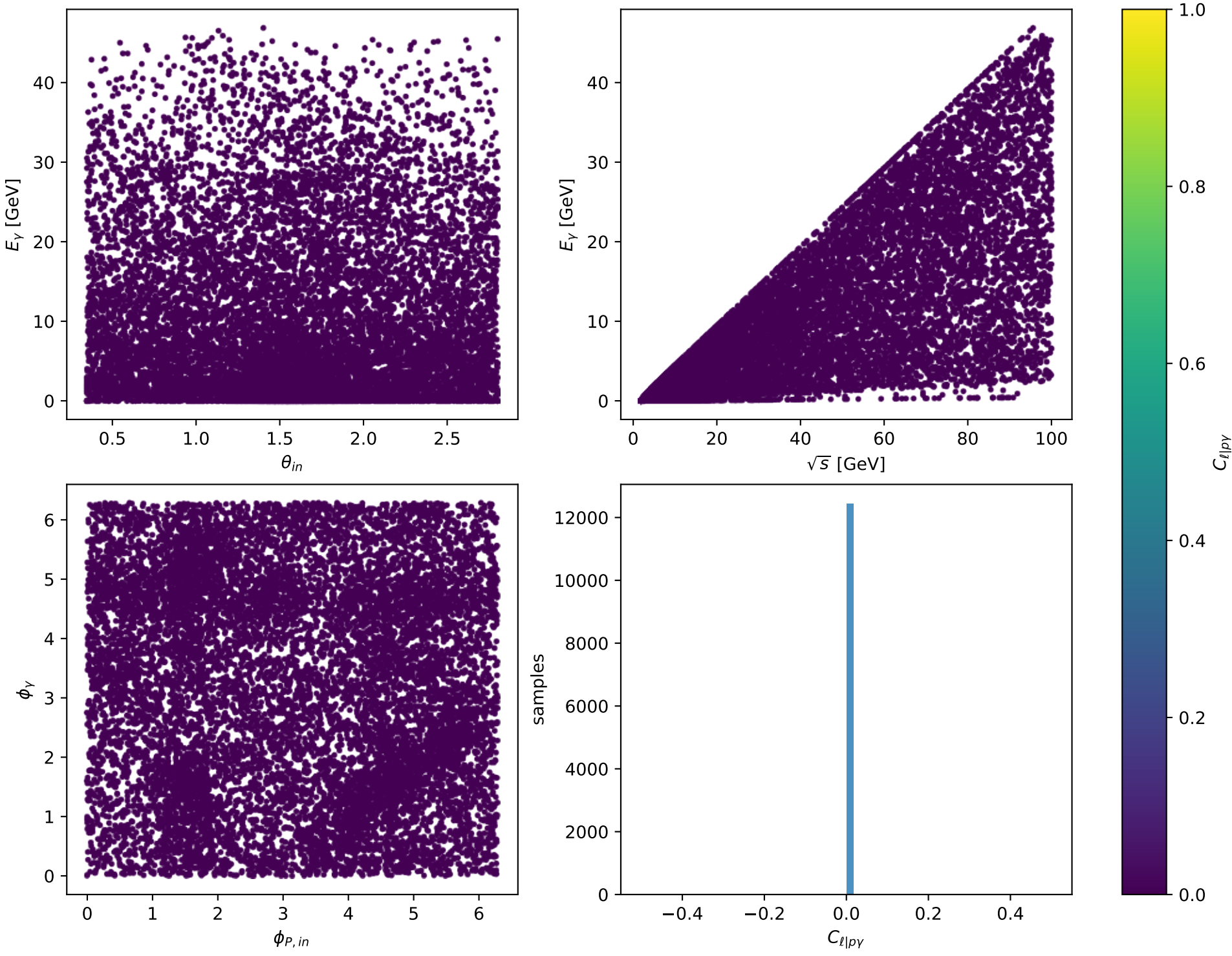
Phase-space scan: Unpolarized [unpolarized], max C_{\ell|p\gamma}=0
