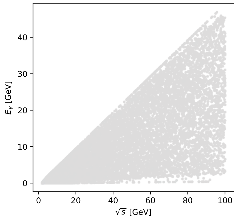
Phase-space scan: Unpolarized [unpolarized], max M_p=-0
