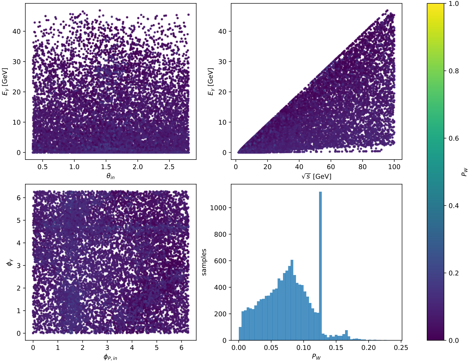
Phase-space scan: Unpolarized [unpolarized], max P_W=0.23954
