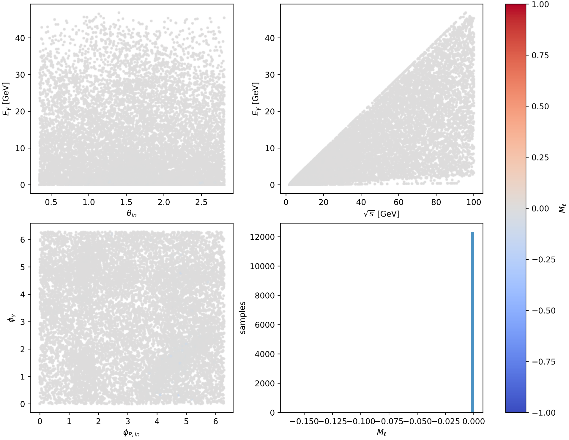
Phase-space scan: Unpolarized [unpolarized], max M_\ell=-0
