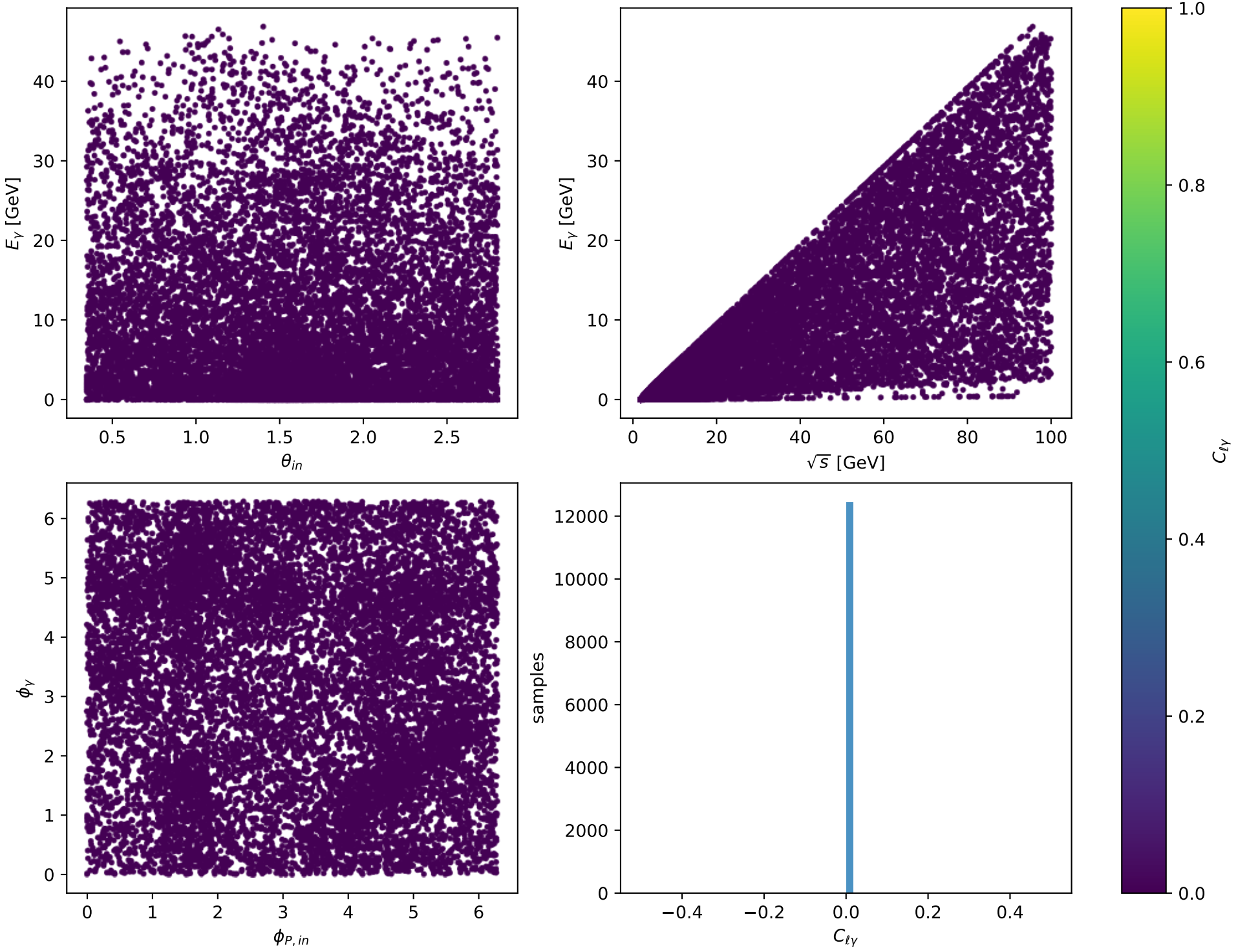
Phase-space scan: Unpolarized [unpolarized], max C_{\ell\gamma}=0
