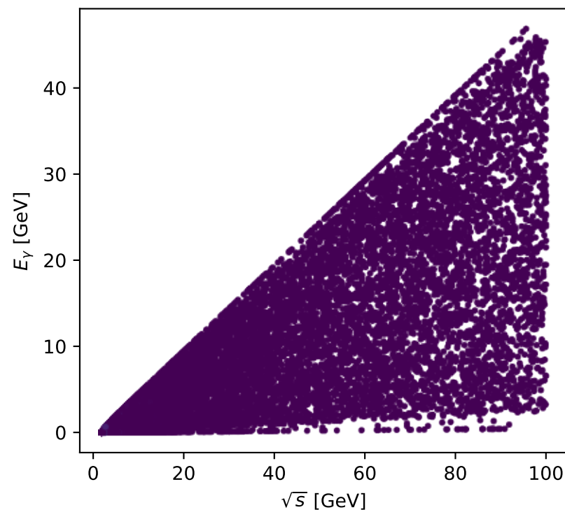
Phase-space scan: Unpolarized [unpolarized], max C_{lp}=0.40357
