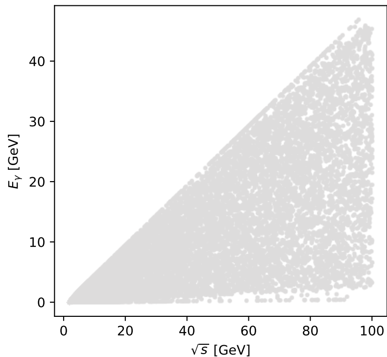
Phase-space scan: Unpolarized [unpolarized], max M_\gamma = -0
