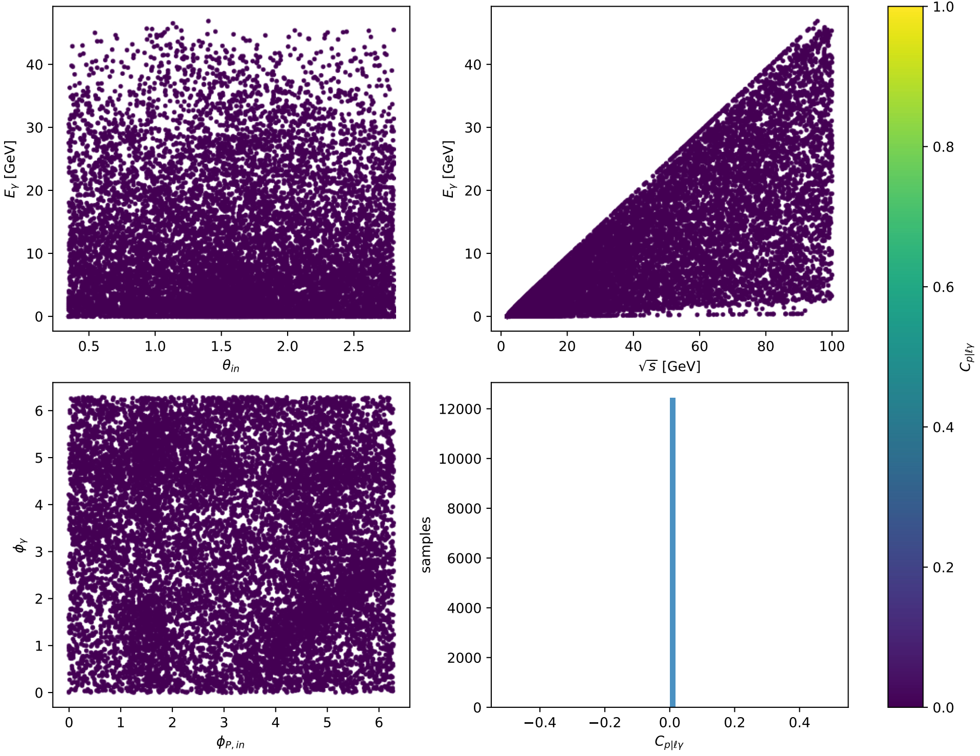
Phase-space scan: Unpolarized [unpolarized], max C_{p|l\gamma}=0
