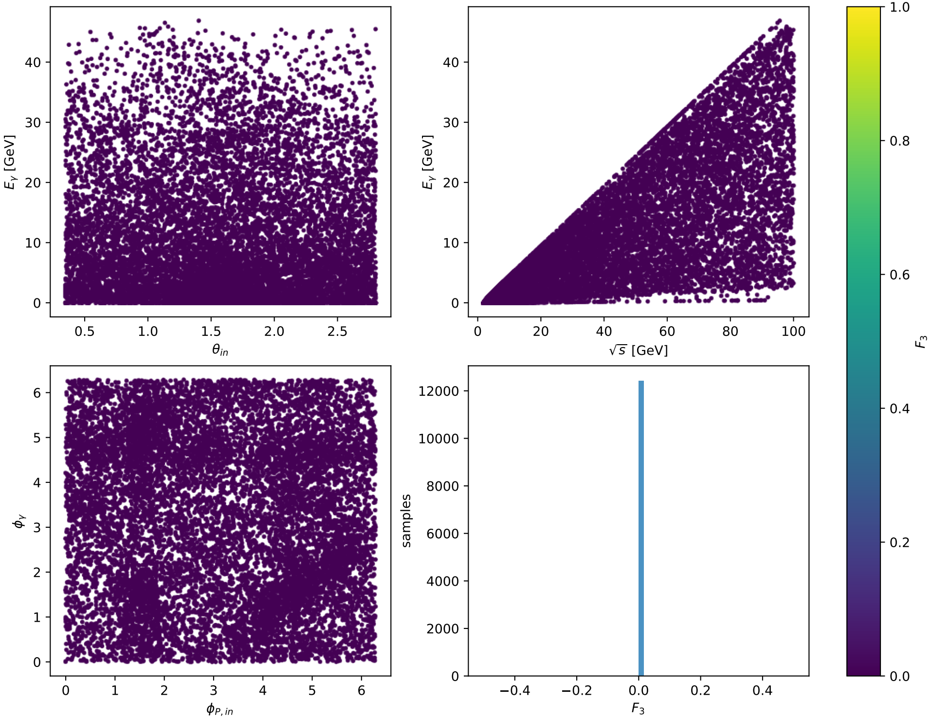
Phase-space scan: Unpolarized [unpolarized], max F_3=0
