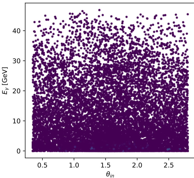
Phase-space scan: Unpolarized [unpolarized], max C_{lp}=0.40357
