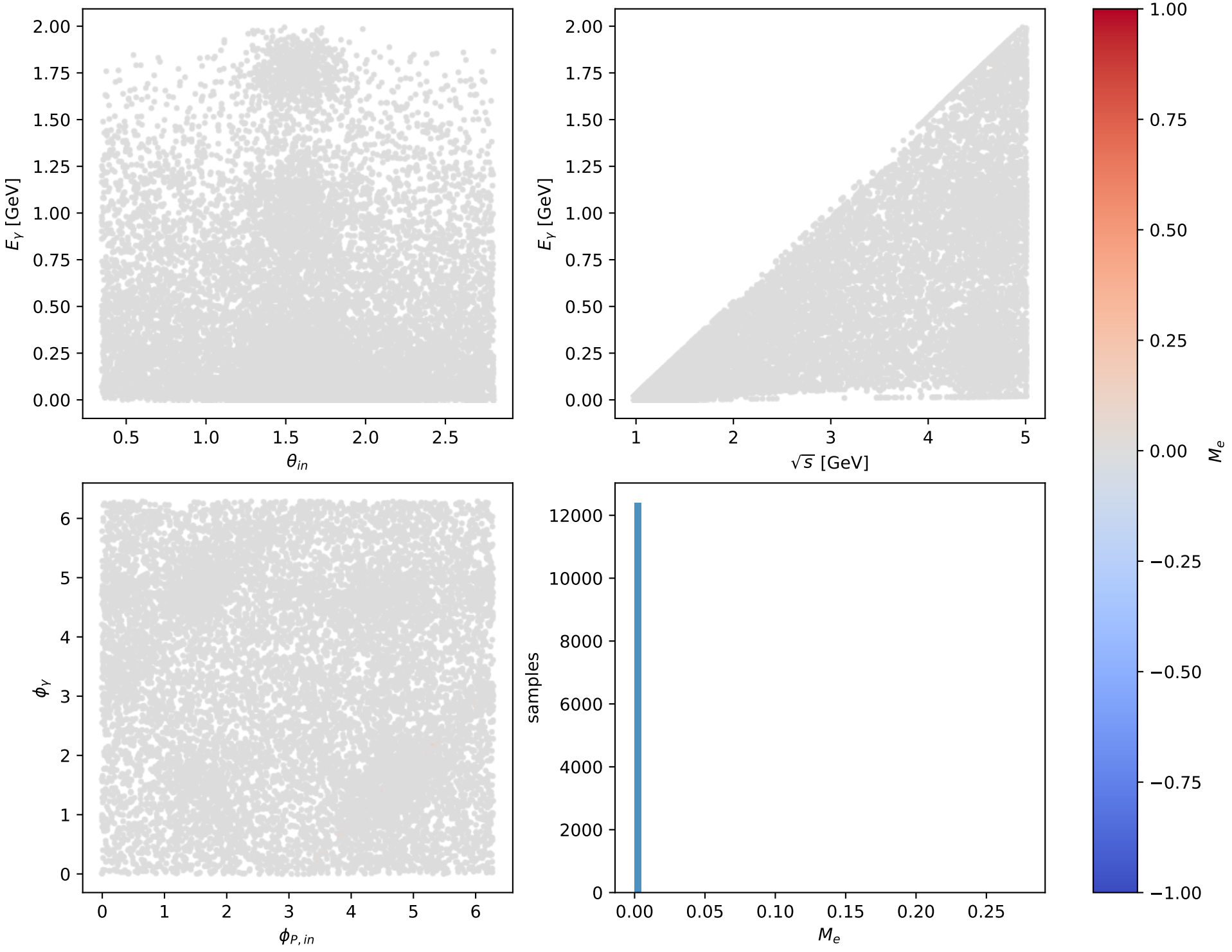
Phase-space scan: L electron + L proton [LL], max M_e=0.27785
