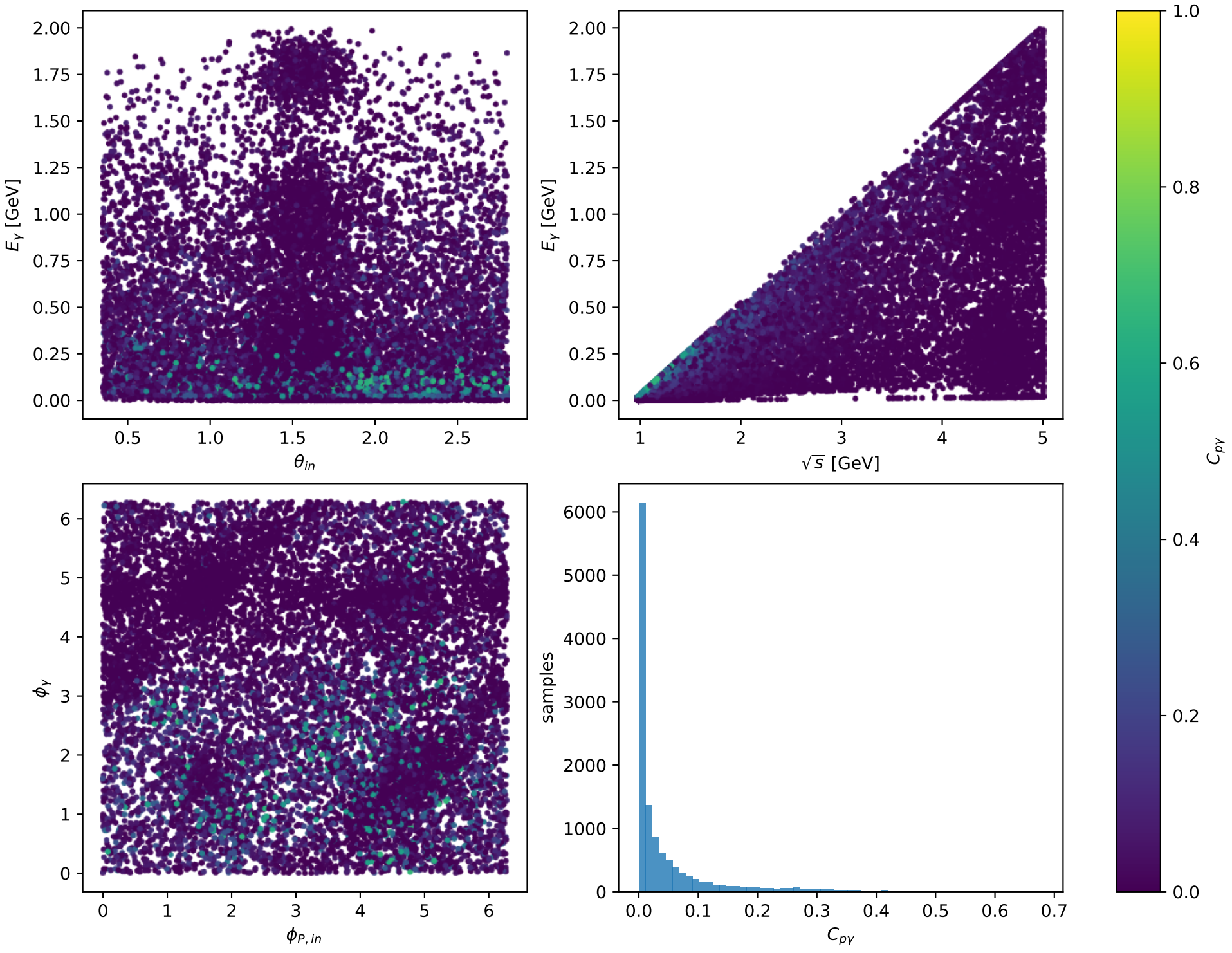
Phase-space scan: L electron [ L_{\text{electron}} ], max C_{p\gamma}=0.68067
