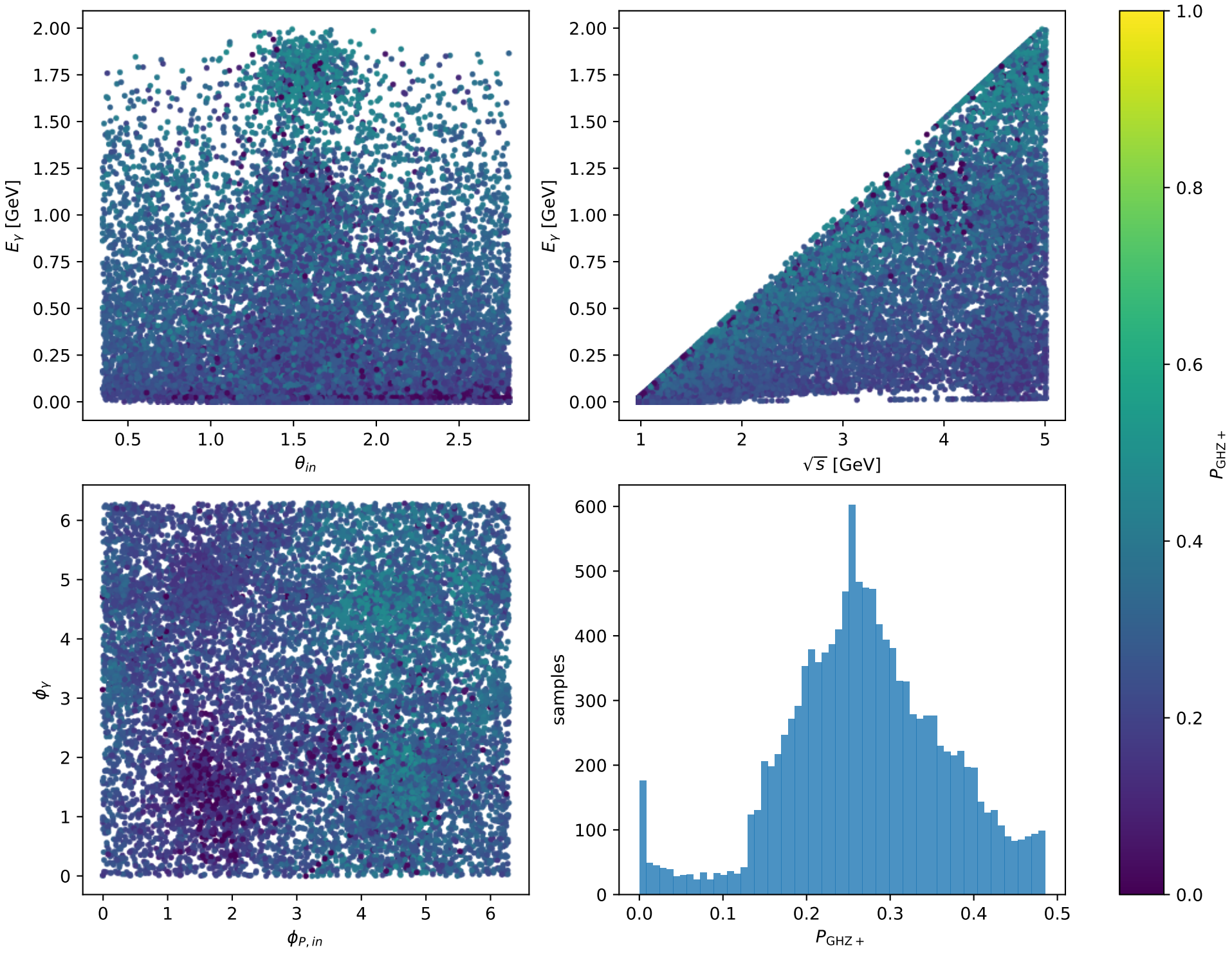
Phase-space scan: L electron [L_electron], max P_{\text{GHZ}+}=0.48525
