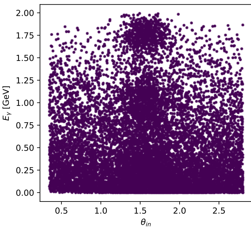
Phase-space scan: L electron [ L_{\text{electron}} ], max C_{\gamma|ep}=1.3657\text{e-}07
