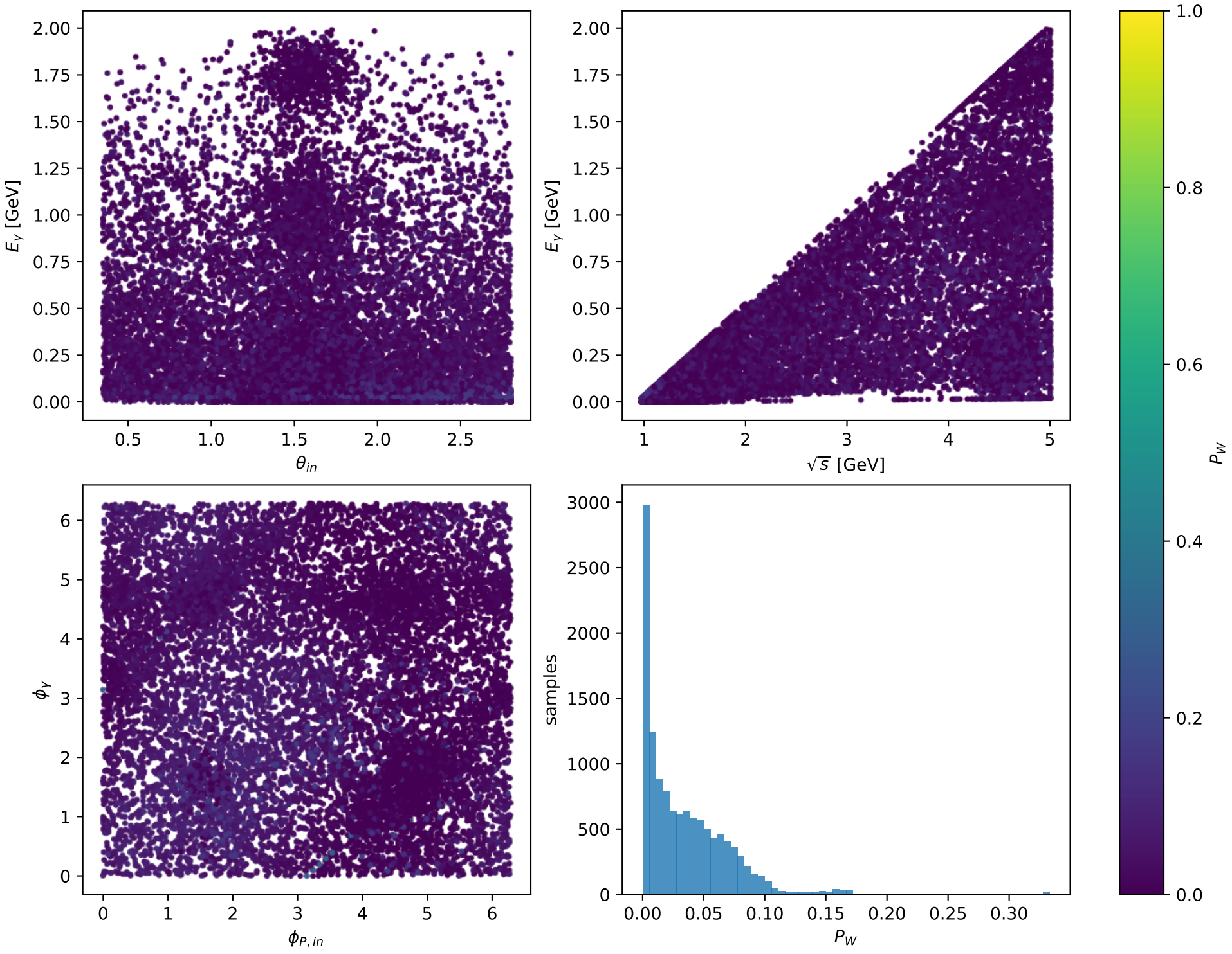
Phase-space scan: L electron [L_electron], max P_W=0.33332
