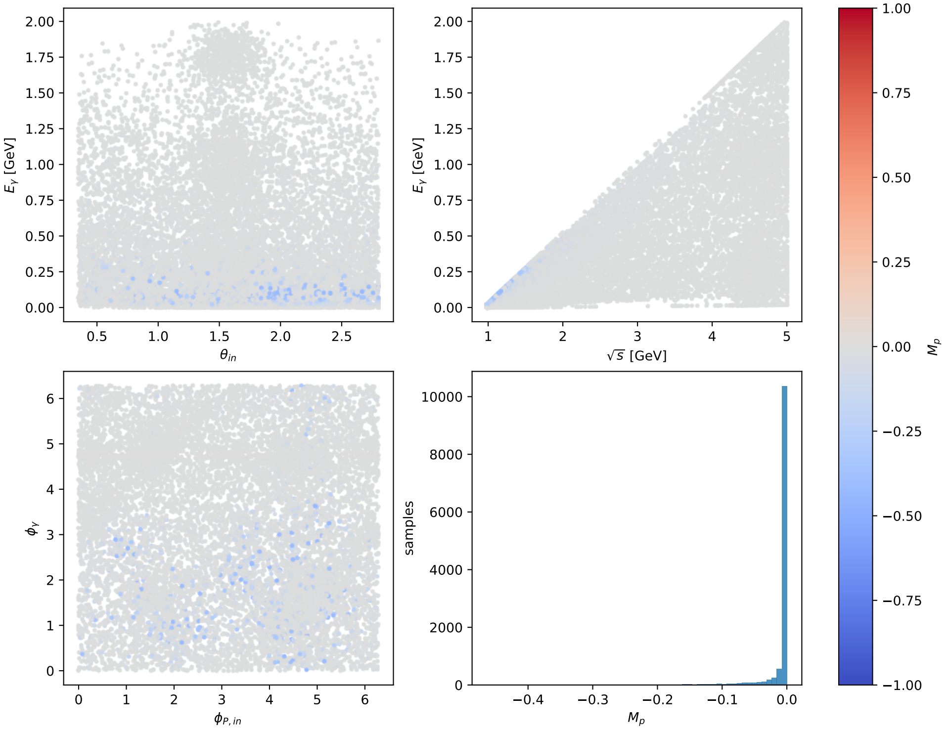
Phase-space scan: L electron [L_electron], max M_p=1.954\text{e-14}
