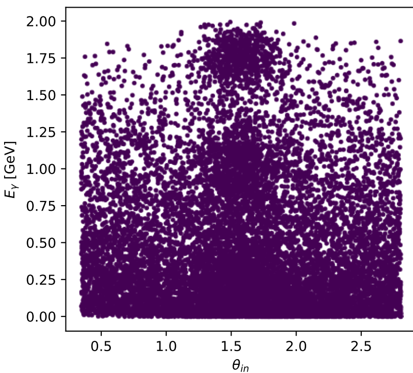
Phase-space scan: L electron [L_electron], max C_{p|ey}=1.3979\text{e-}07
