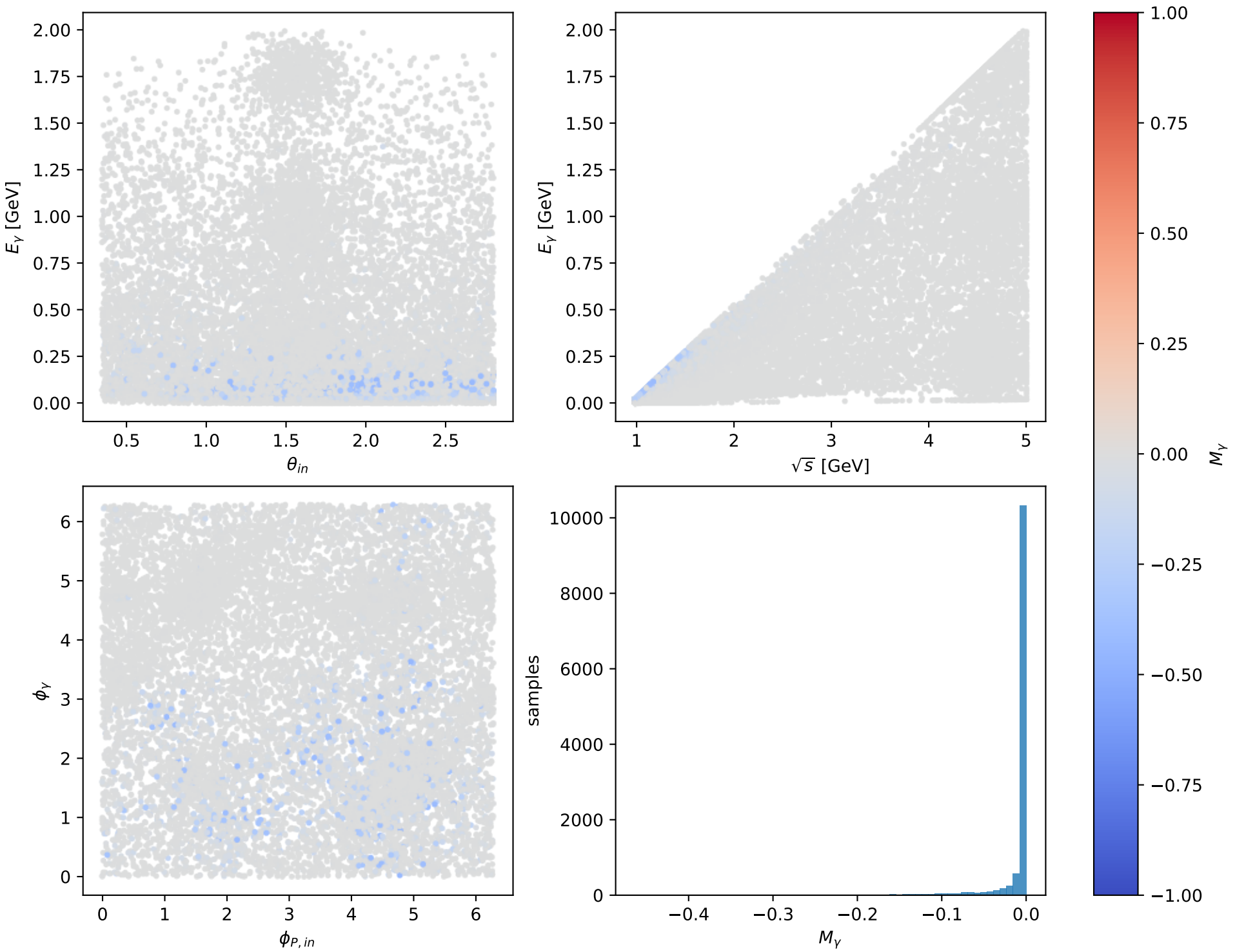
Phase-space scan: L electron [L_electron], max M_\gamma=1.8652\text{e-14}
