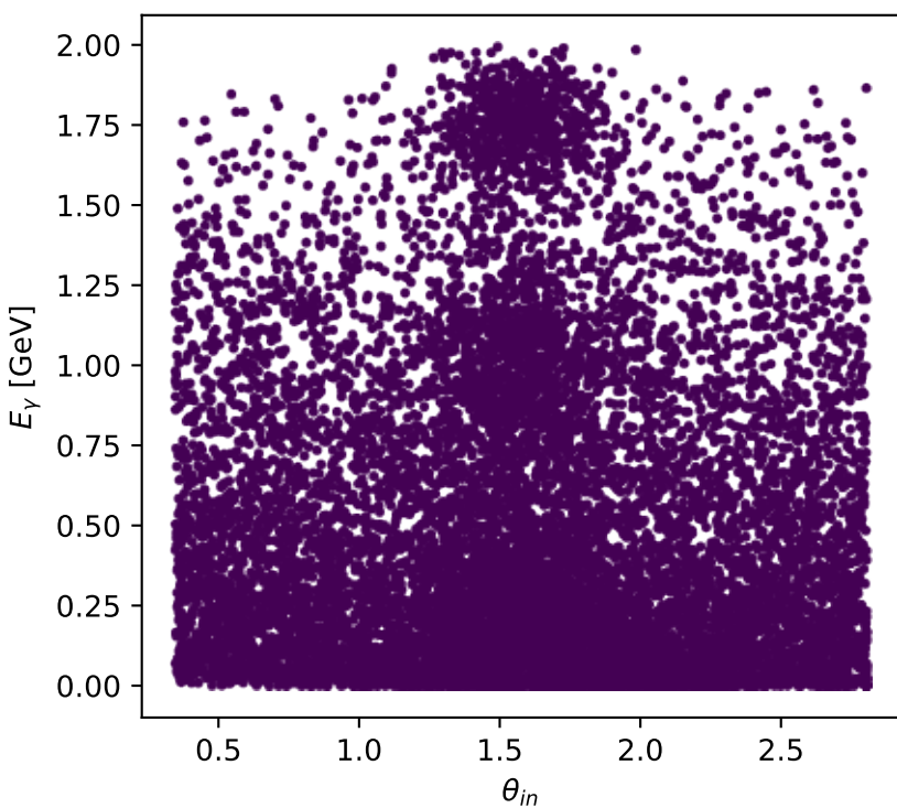
Phase-space scan: L electron [L_electron], max F_3=1.8939\text{e-14}
