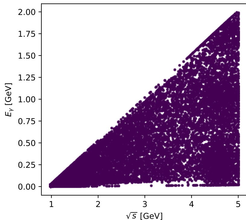
Phase-space scan: L electron [L_electron], max C_{e|p\gamma}=1.3657\text{e-}07
