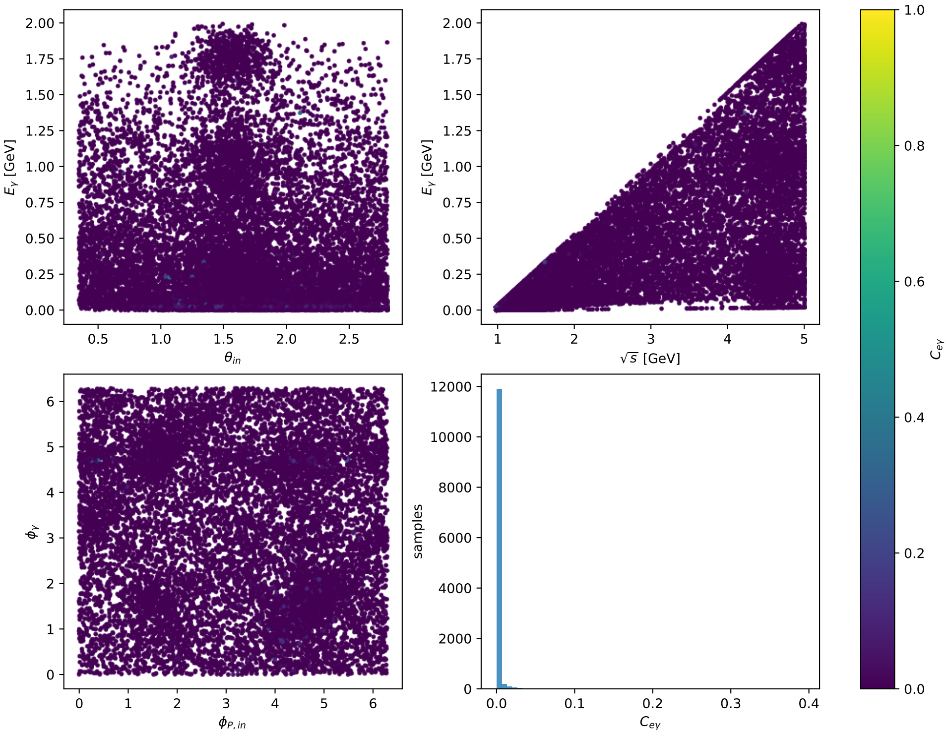
Phase-space scan: L electron [L_electron], max C_{ey}=0.39394
