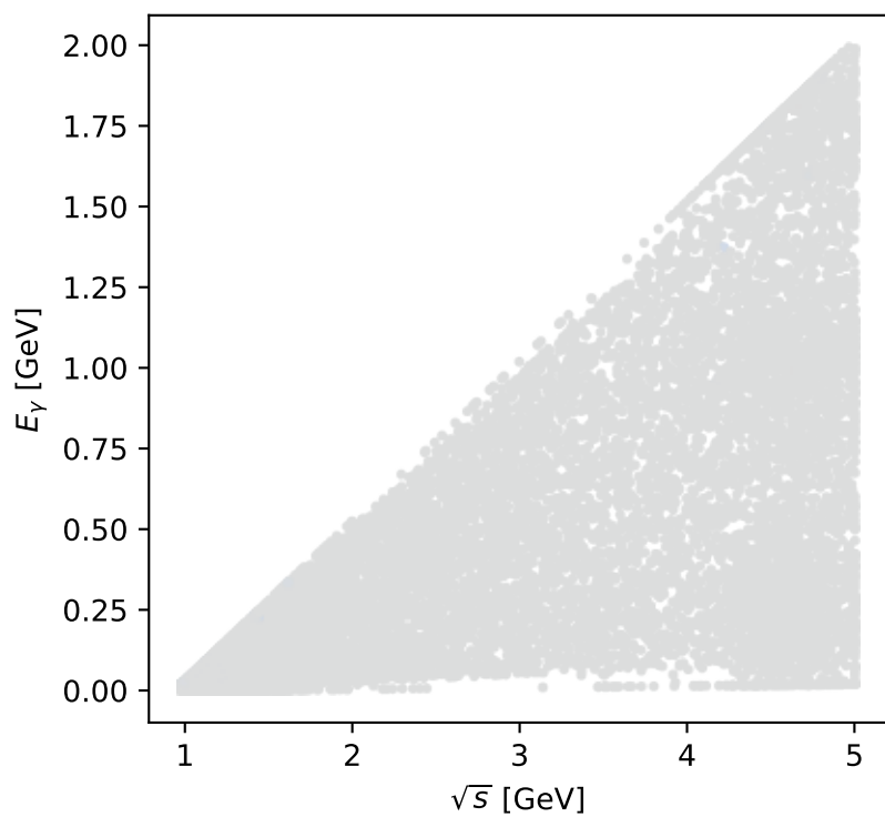
Phase-space scan: L electron [L_electron], max M_e=1.8652\text{e-14}
