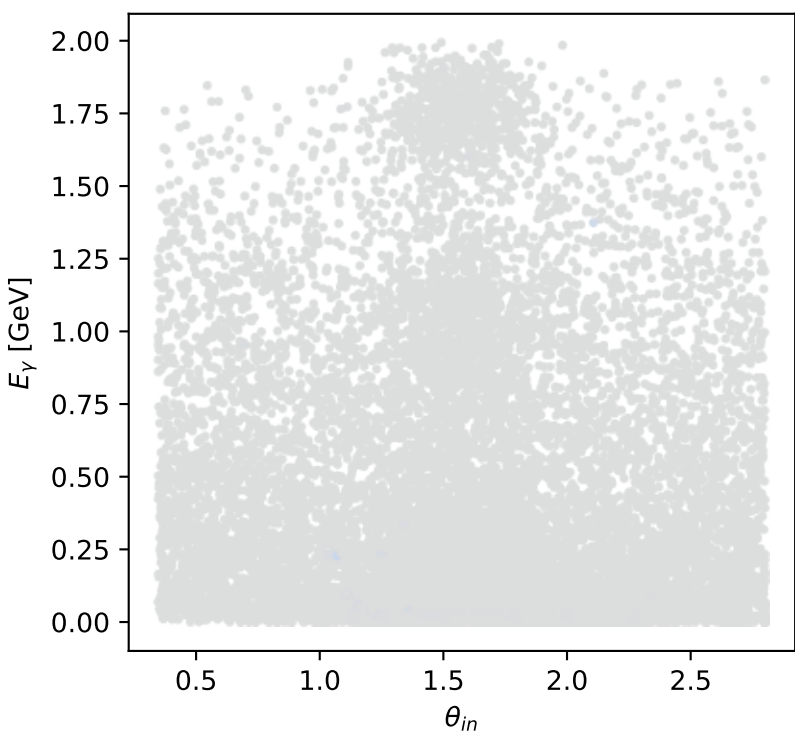
Phase-space scan: L electron [L_electron], max M_e=1.8652\text{e-14}
