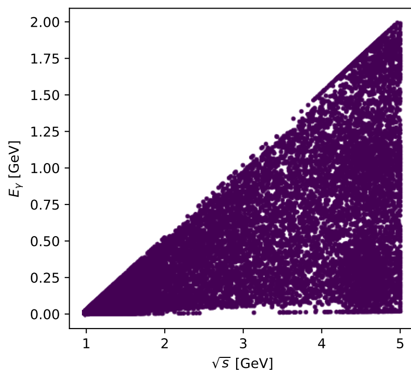
Phase-space scan: L proton [L_proton], max C_{e|p\gamma}=3.1399\text{e-}07
