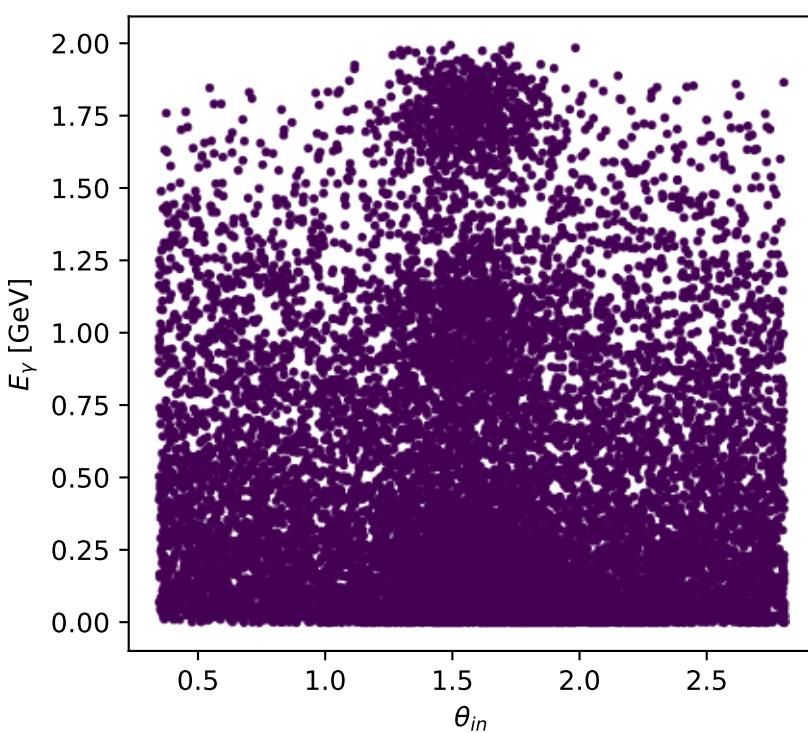
Phase-space scan: L proton [L_proton], max C_{e|p\gamma}=3.1399\text{e-}07
