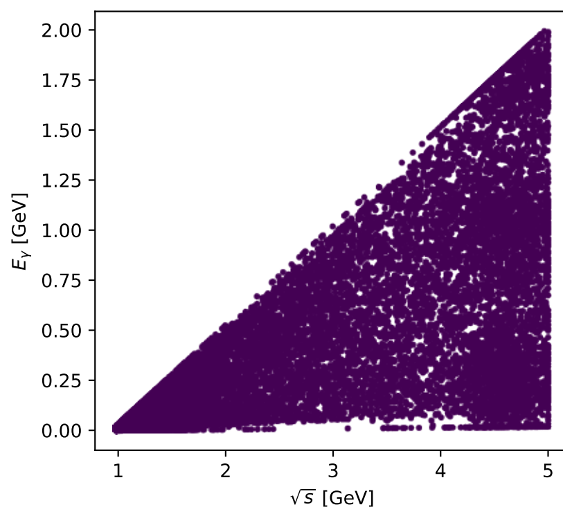
Phase-space scan: L proton [ L_{\text{proton}} ], max C_{p|e\gamma}=3.437\text{e-}07
