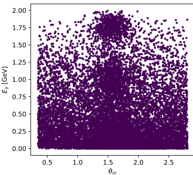
Phase-space scan: L proton [ L_{\text{proton}} ], max C_{p|e\gamma}=3.437\text{e-}07
