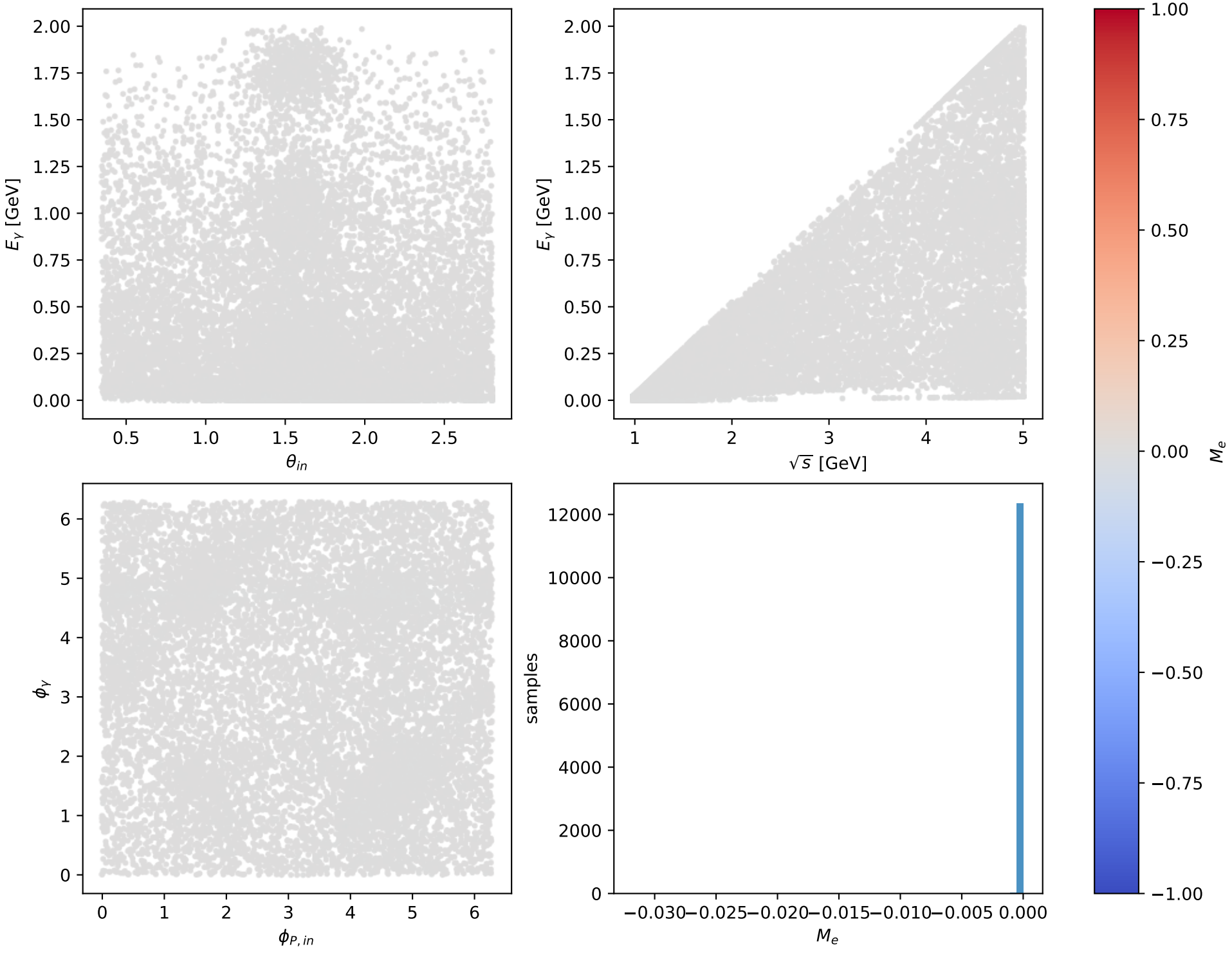
Phase-space scan: Tx proton [Tx_proton], max M_e = -0
