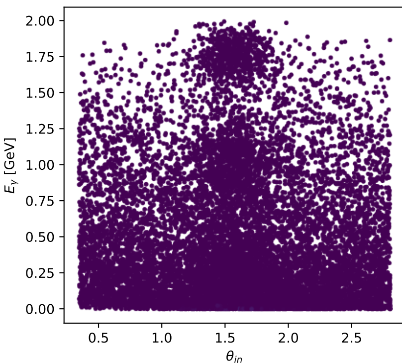
Phase-space scan: Tx proton [Tx_proton], max C_{ep}=0.17813
