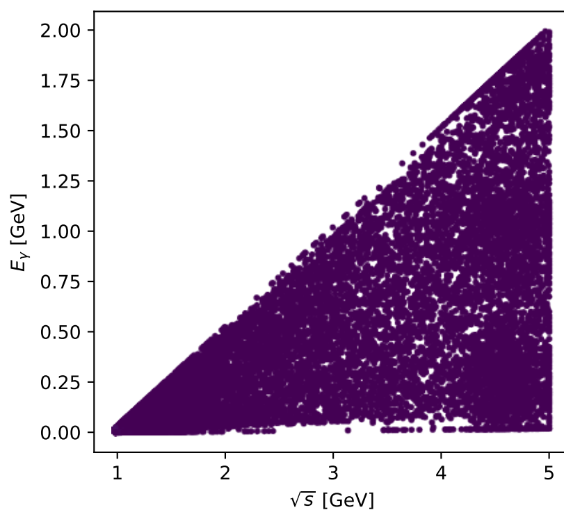
Phase-space scan: Ty electron [Ty_electron], max C_{ep}=0.18592
