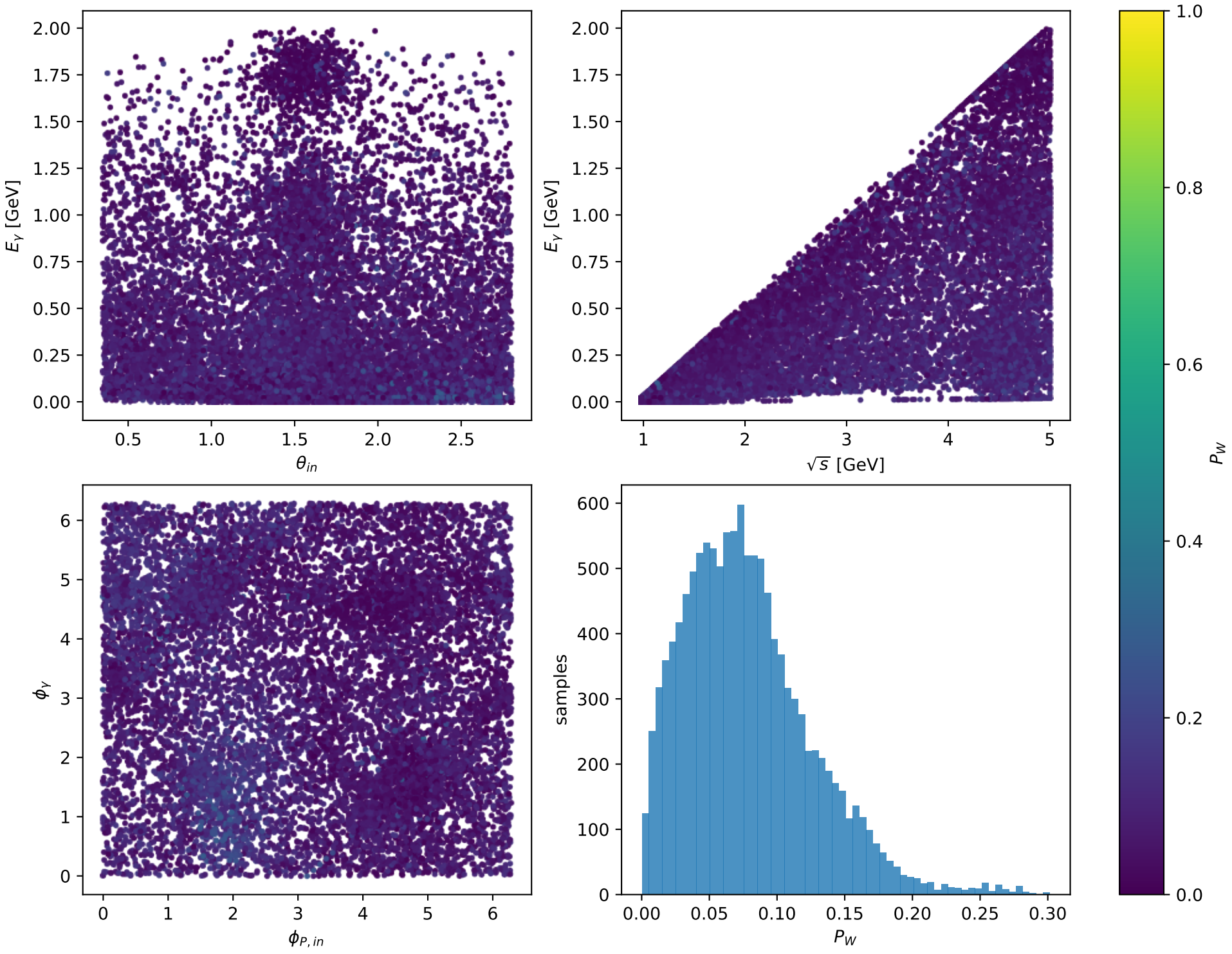
Phase-space scan: Ty proton [Ty_proton], max P_W=0.30152
