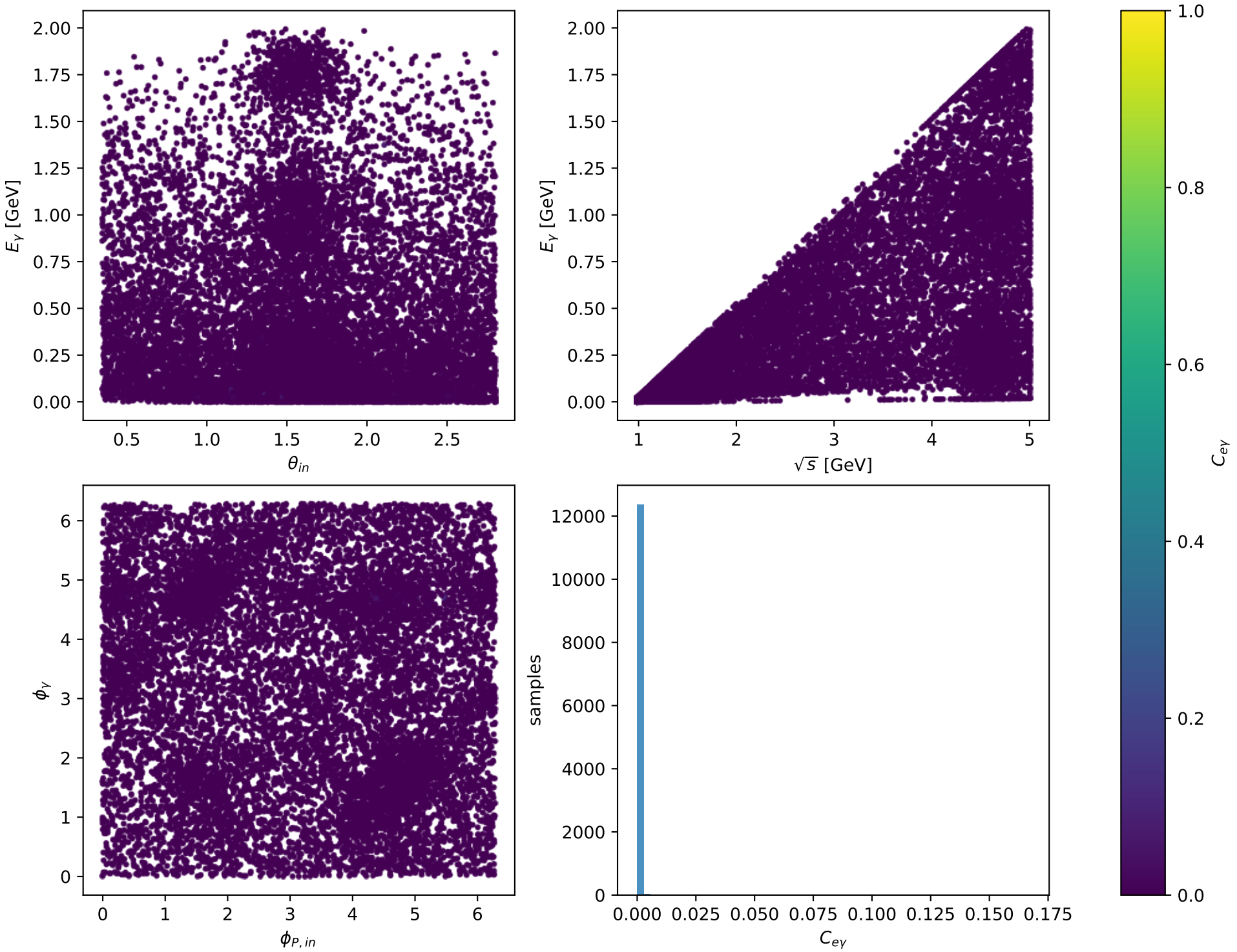
Phase-space scan: Ty proton [Ty_proton], max C_{e\gamma}=0.16712
