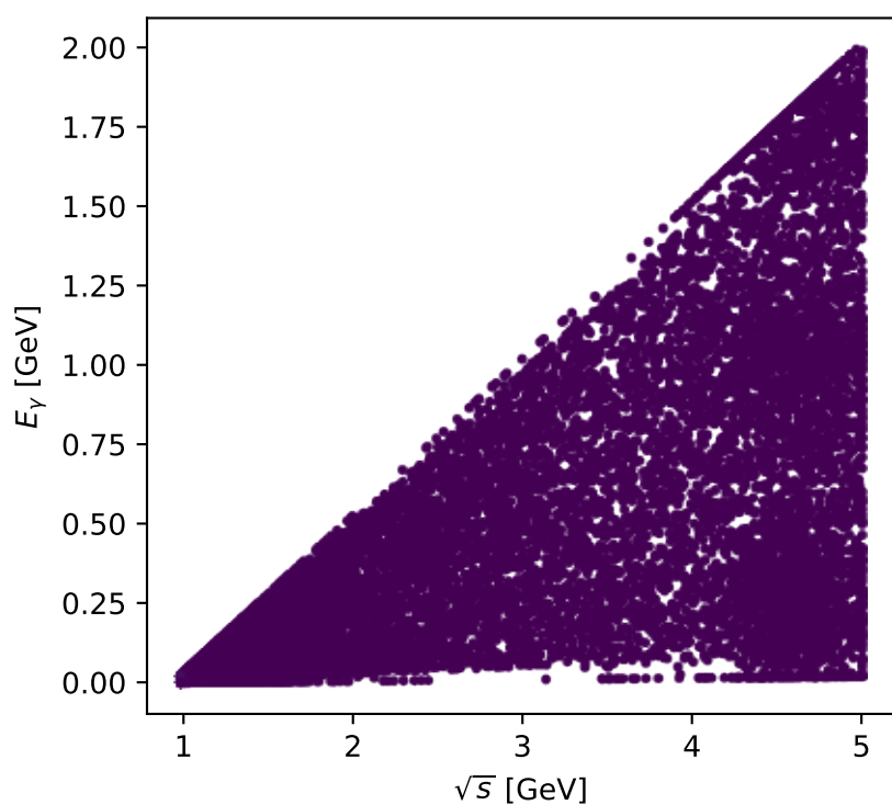
Phase-space scan: Ty proton [Ty_proton], max C_{ep}=0.1745
