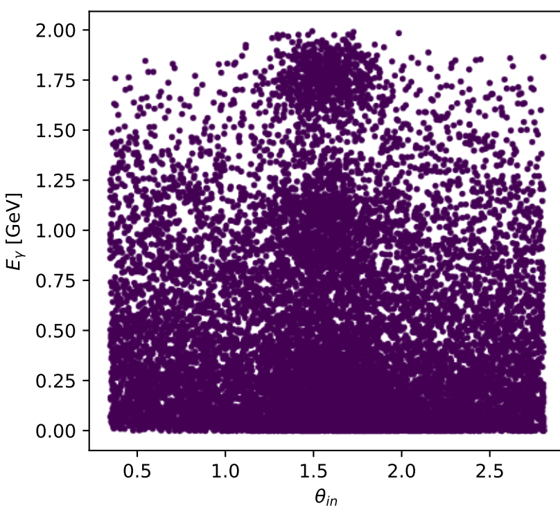
Phase-space scan: Ty proton [Ty_proton], max C_{e|p\gamma}=0
