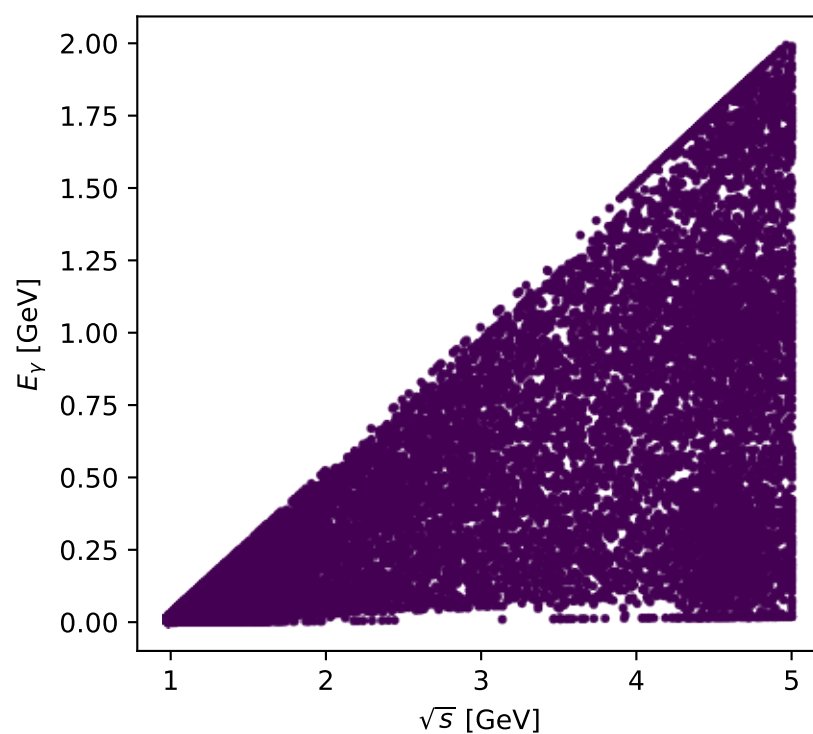
Phase-space scan: Ty proton [Ty_proton], max C_{e|p\gamma}=0
