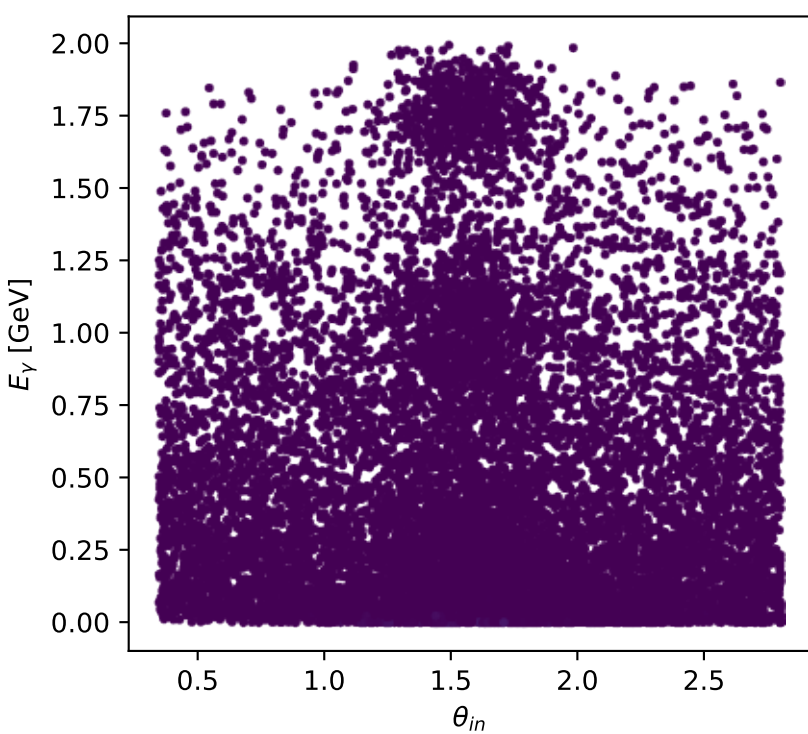
Phase-space scan: Ty proton [Ty_proton], max C_{ep}=0.1745
