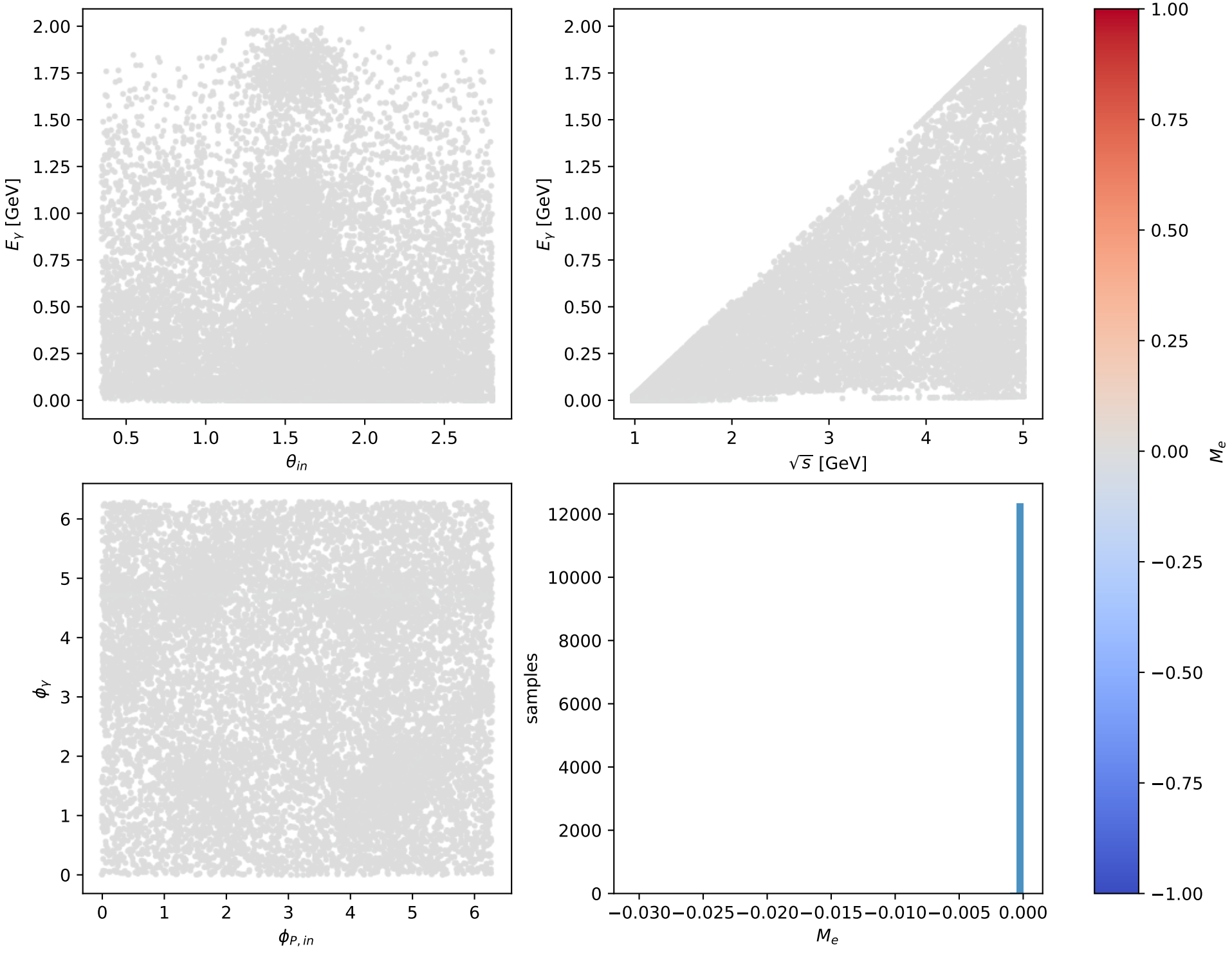
Phase-space scan: Ty proton [Ty_proton], max M_e=-0
