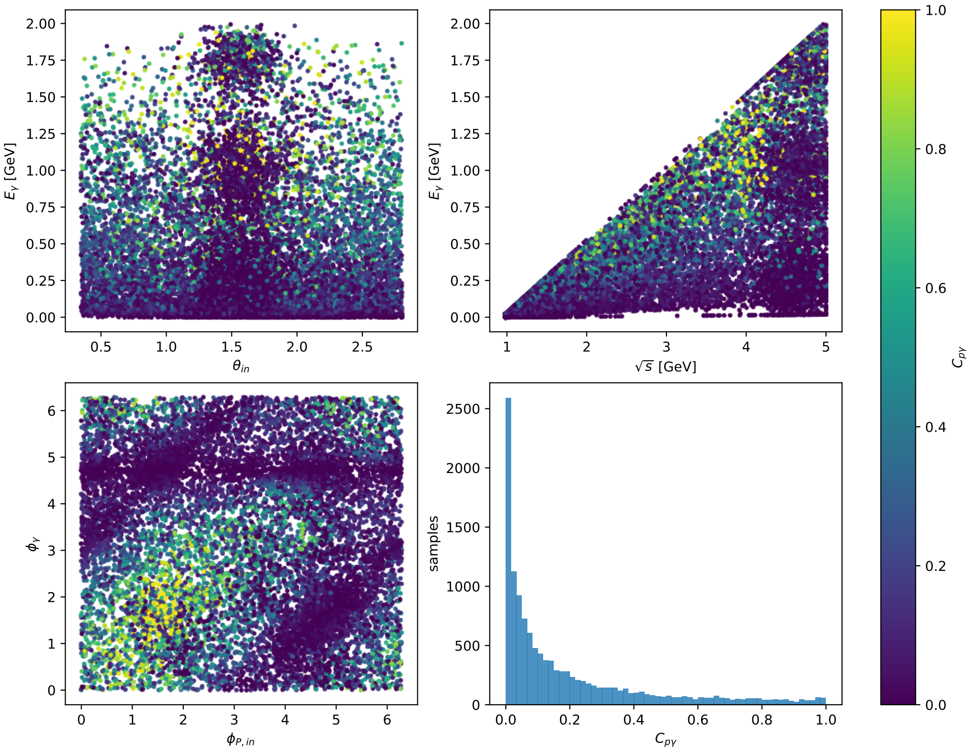
Phase-space scan: T_y proton [ T_y proton], max C_{p\gamma}=0.99999
