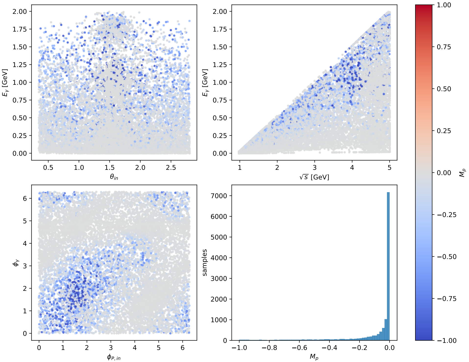
Phase-space scan: Ty proton [Ty_proton], max M_p=-0
