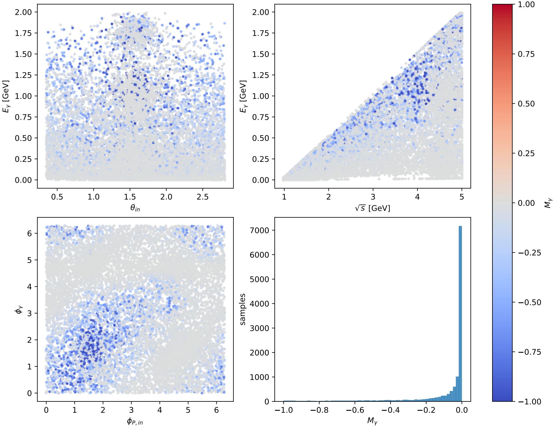
Phase-space scan: Ty proton [Ty_proton], max M_Y=-0
