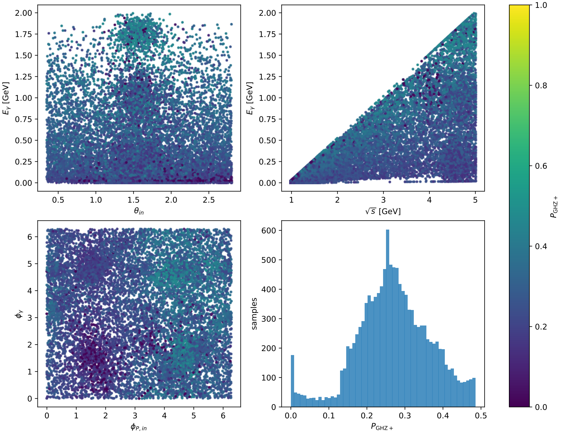
Phase-space scan: Ty proton [Ty_proton], max P_{\text{GHZ}+}=0.48525
