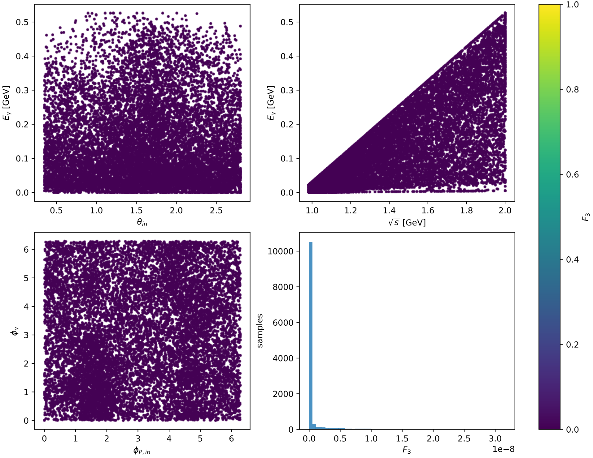
Phase-space scan: L massless lepton + L proton [LL], max F_3=3.1589\text{e-}08
