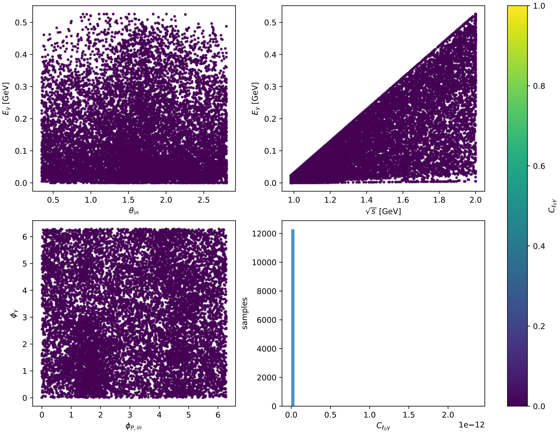
Phase-space scan: L massless lepton + L proton [LL], max C_{\ell_0\gamma}=2.3516\text{e-}12
