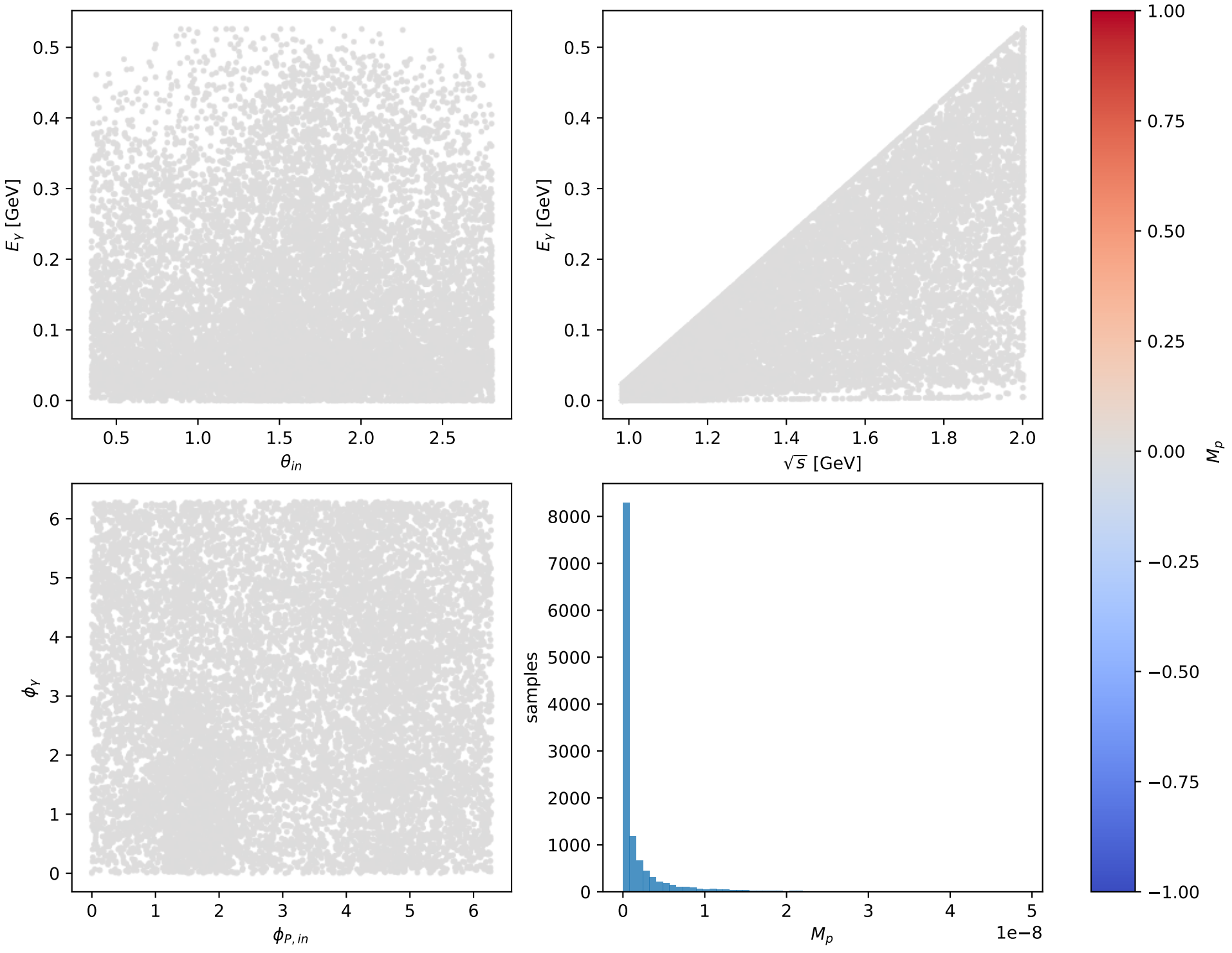
Phase-space scan: L massless lepton + L proton [LL], max M_p=4.8853\text{e-}08
