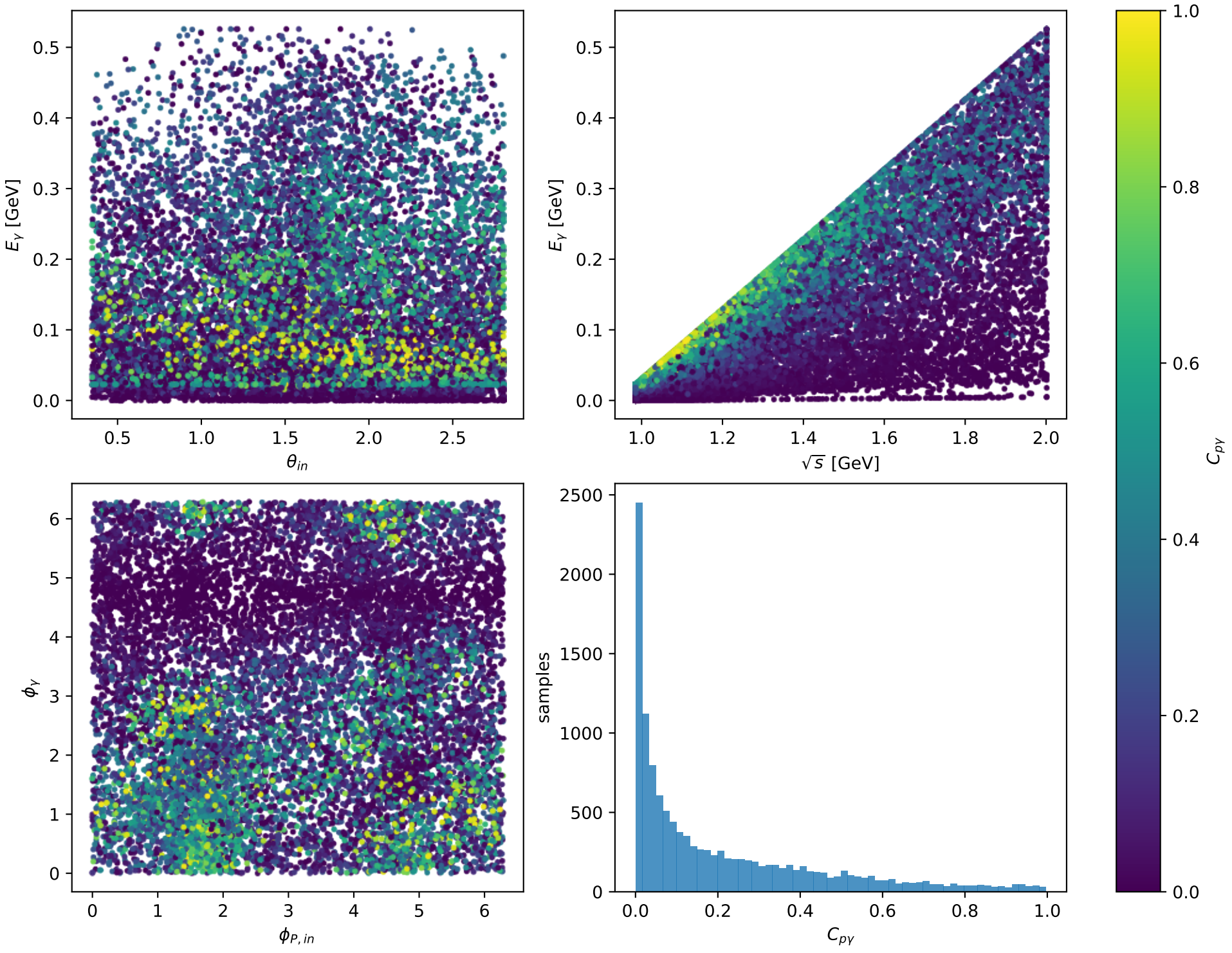
Phase-space scan: L massless lepton + L proton [LL], max C_{p\gamma}=0.99704
