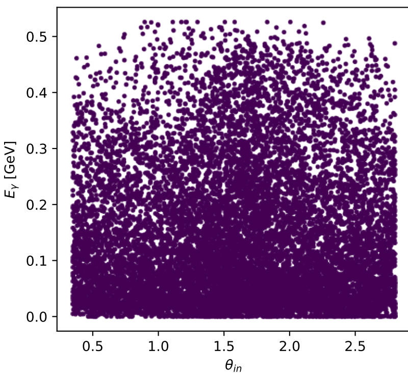
Phase-space scan: L massless lepton + L proton [LL], max C_{\ell_0|p\gamma}=3.65\text{e-}08
