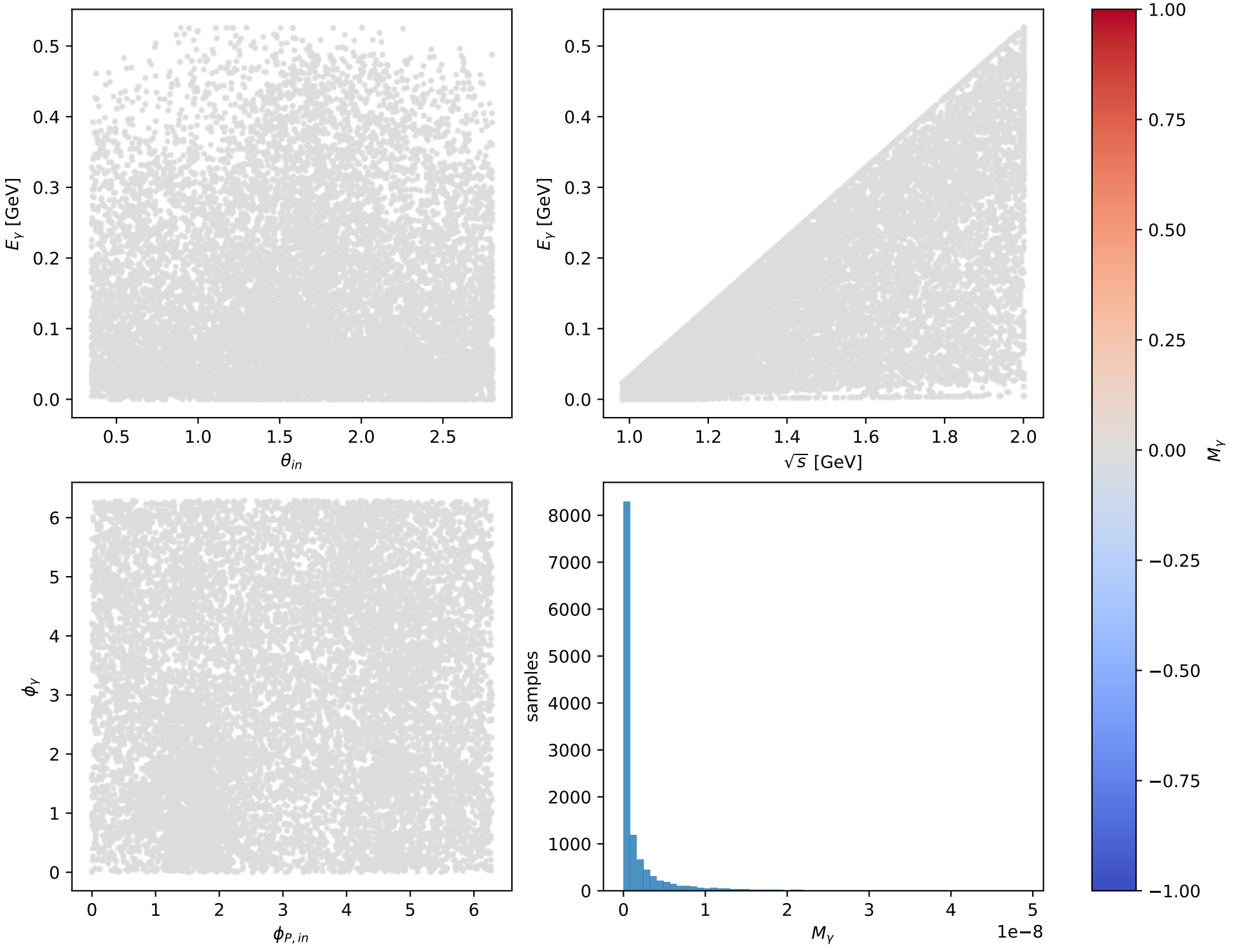
Phase-space scan: L massless lepton + L proton [LL], max M_\gamma=4.8853\text{e-}08
