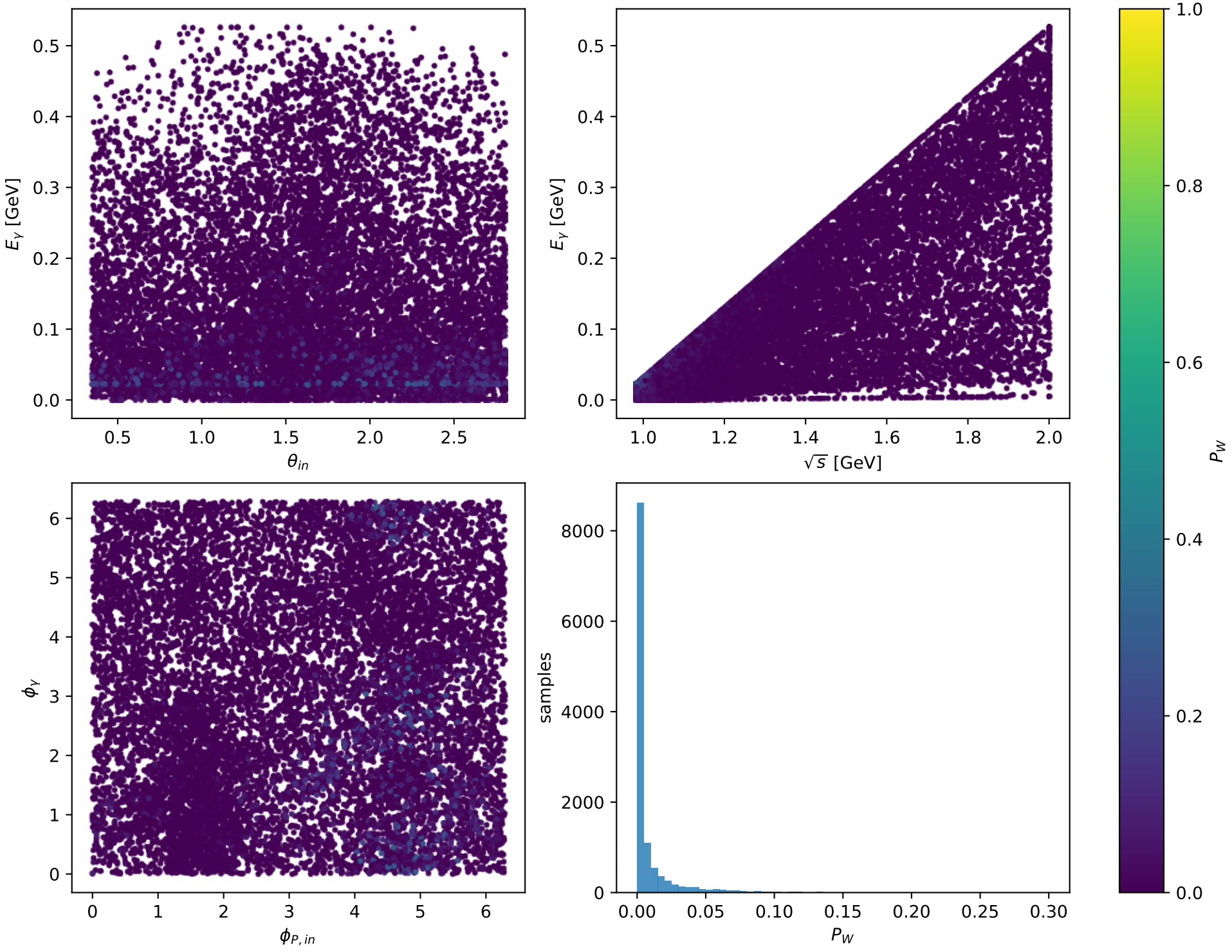
Phase-space scan: L massless lepton+ L proton [LL], max P_W=0.30024
