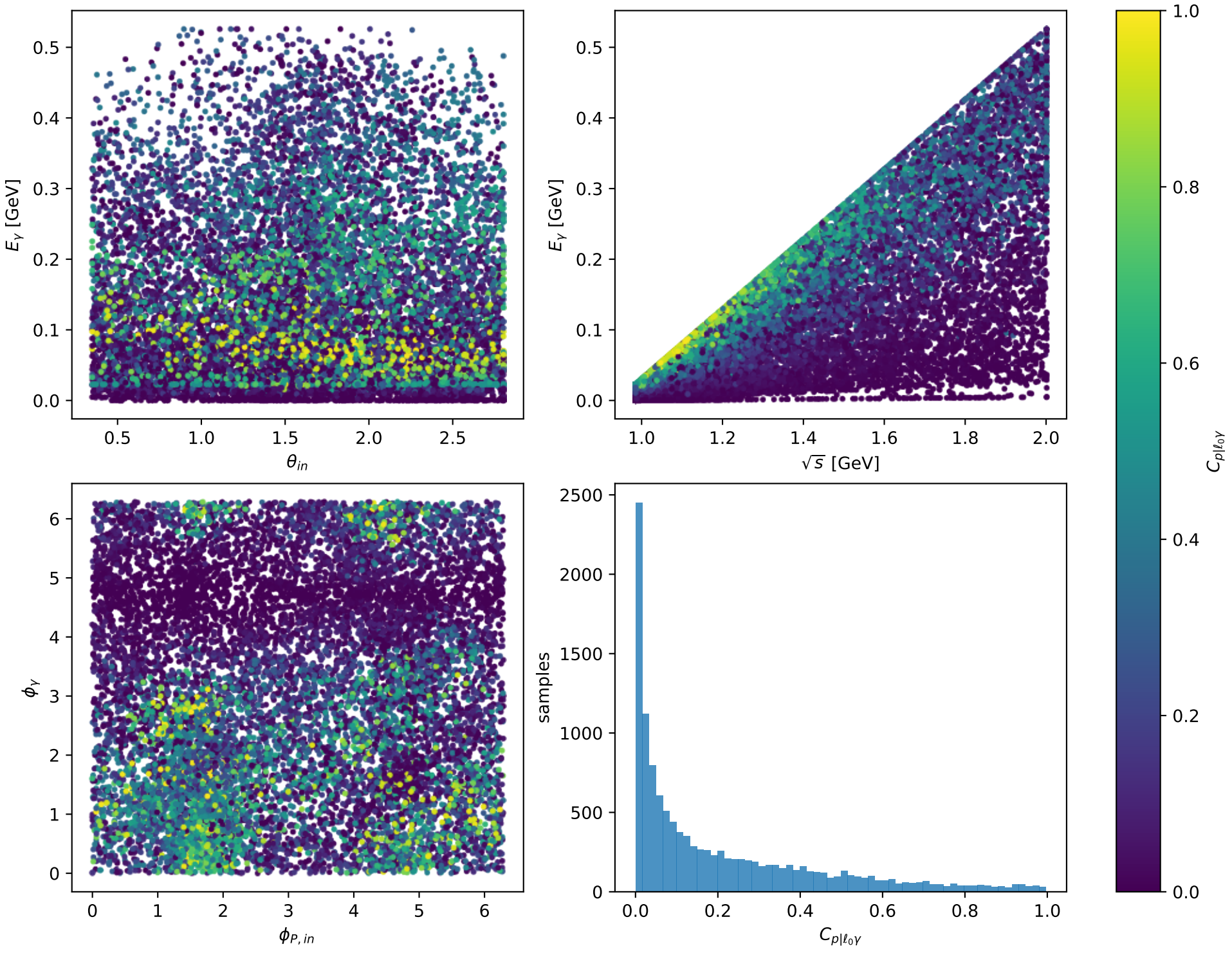
Phase-space scan: L massless lepton + L proton [LL], max C_{p|\ell_0\gamma}=0.99704
