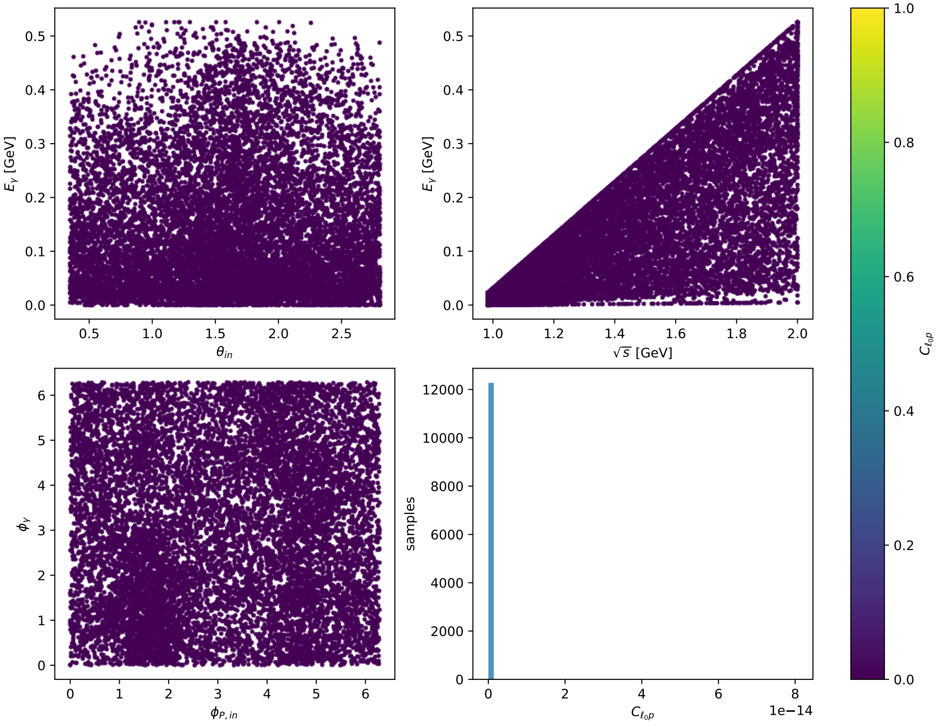
Phase-space scan: L massless lepton + L proton [LL], max C_{\ell_0 p}=8.0604\text{e-}14
