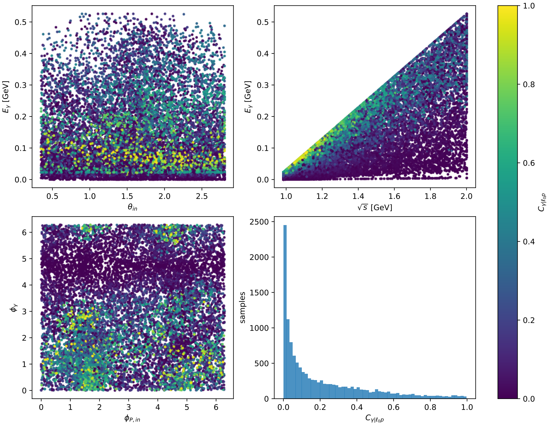
Phase-space scan: L massless lepton + L proton [LL], max C_{\gamma|\ell_0 p}=0.99704
