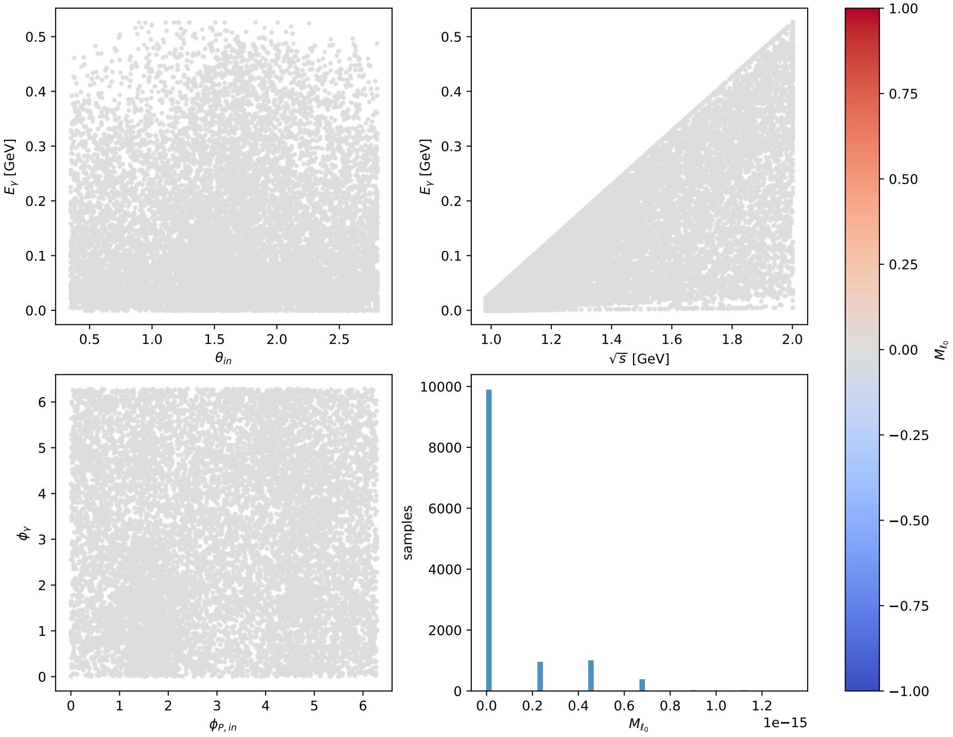
Phase-space scan: L massless lepton + L proton [LL], max M_{\ell_0}=1.3323\text{e-15}
