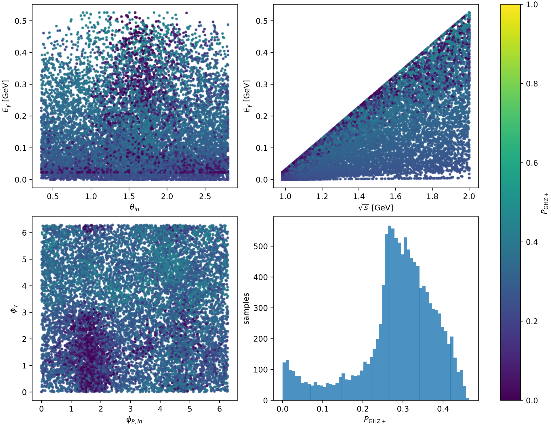
Phase-space scan: L massless lepton + L proton [LL], max P_{\text{GHZ}+}=0.4648
