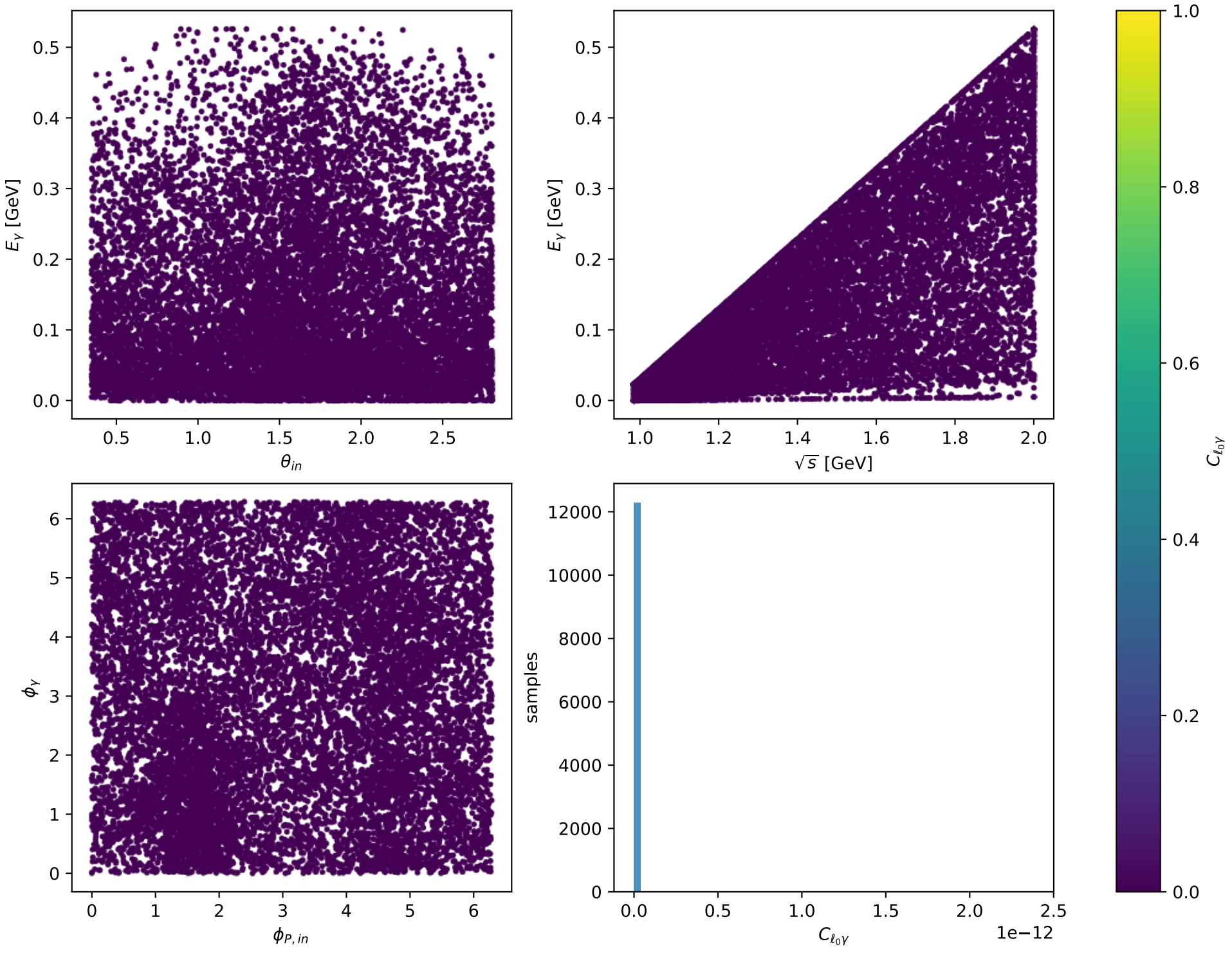
Phase-space scan: L massless lepton + Tx proton [LTx], max C_{\ell_0\gamma}=2.3817\text{e-12}
