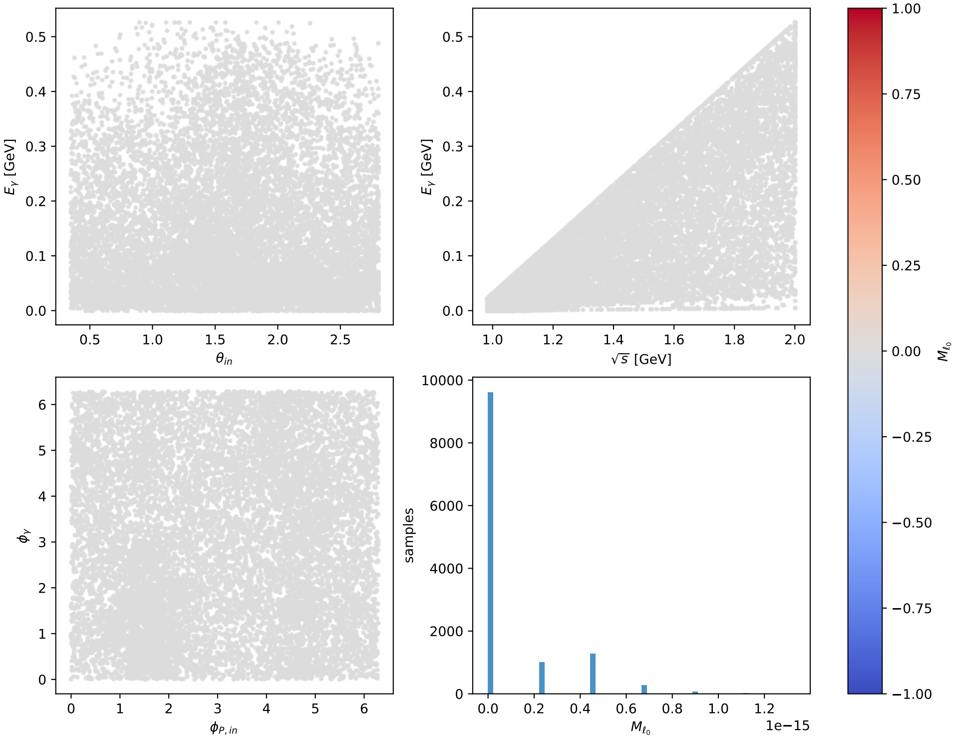
Phase-space scan: L massless lepton + Tx proton [LTx], max M_{\ell_0}=1.3323\text{e-15}
