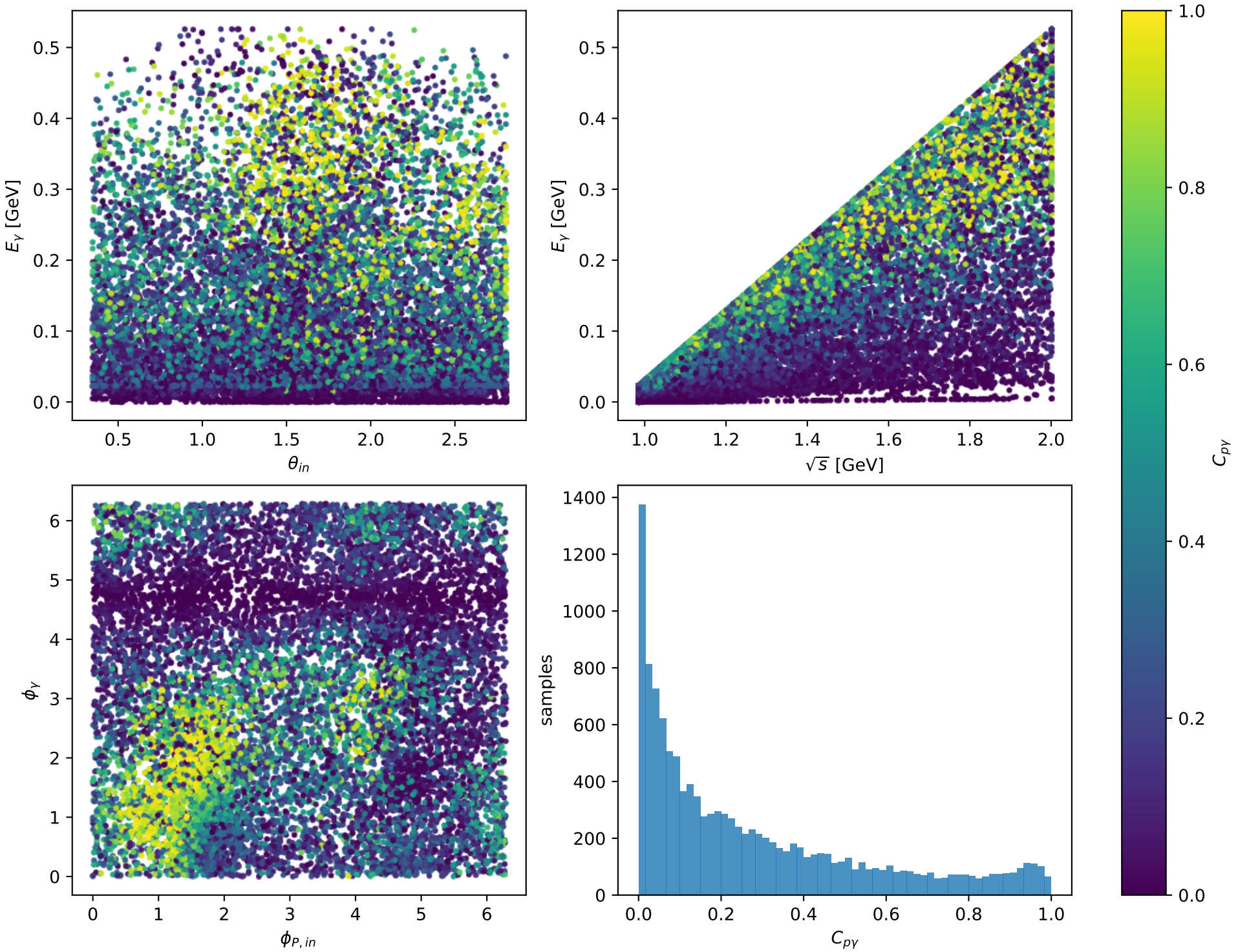
Phase-space scan: L massless lepton + Tx proton [LTx], max C_{p\gamma}=0.9998
