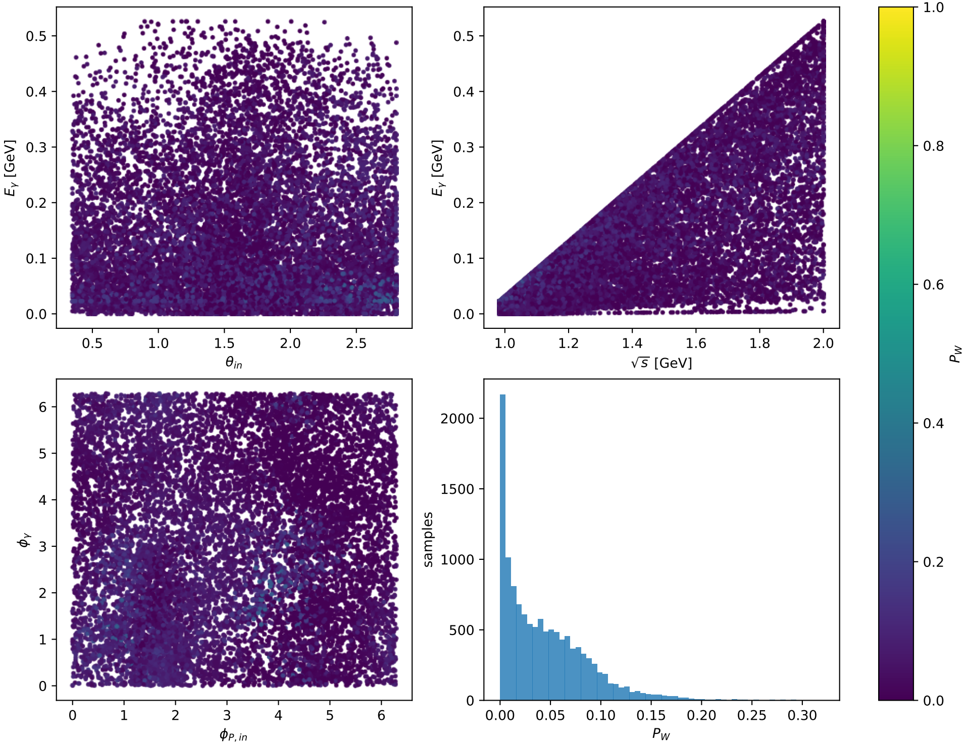
Phase-space scan: L massless lepton + Tx proton [LTx], max P_W=0.32095
