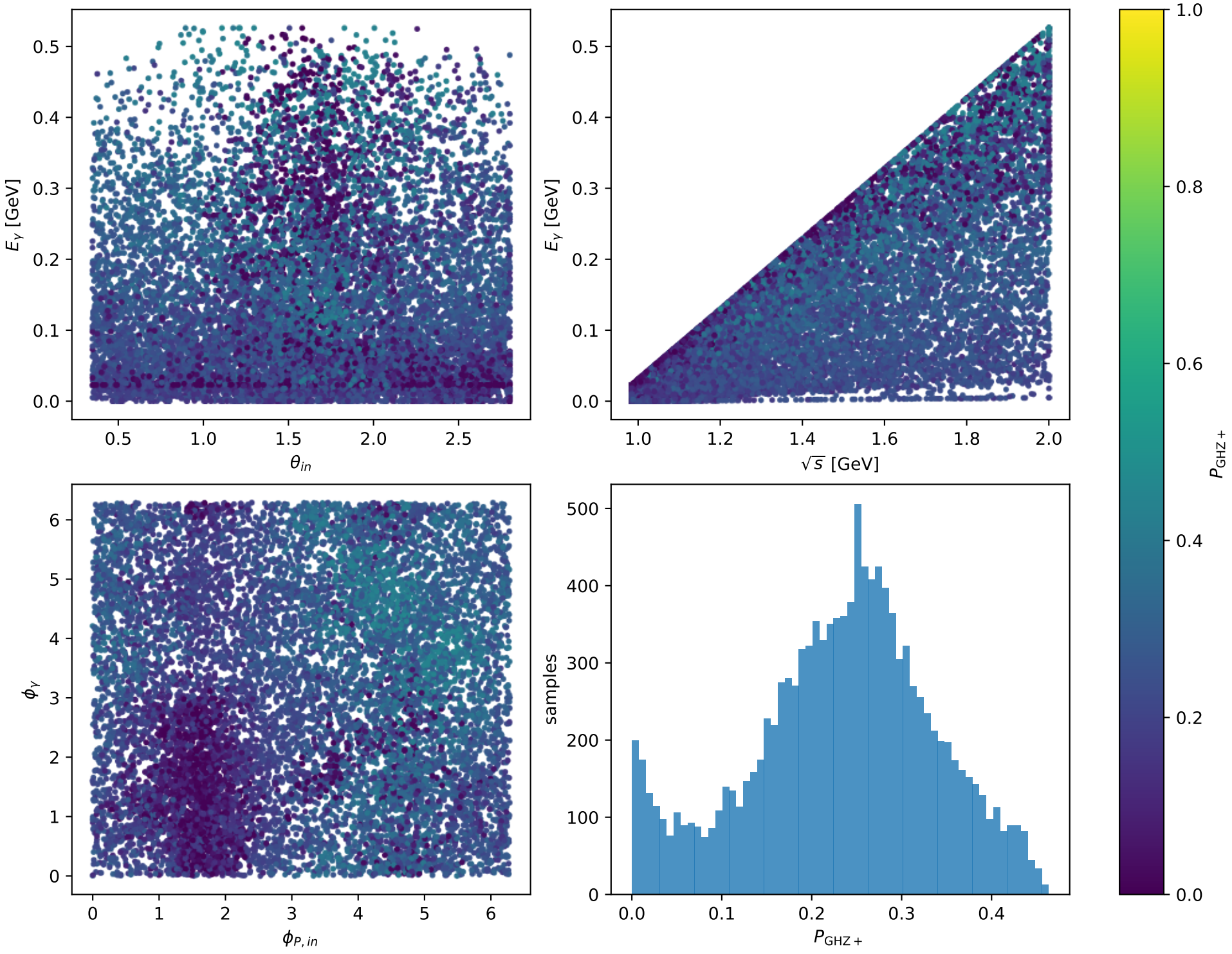
Phase-space scan: L massless lepton + Tx proton [LTx], max P_{\text{GHZ}+}=0.46368
