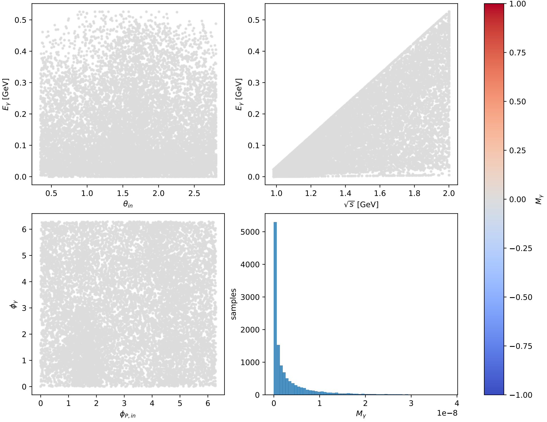
Phase-space scan: L massless lepton + Tx proton [LTx], max M_\gamma=3.8235\text{e-}08
