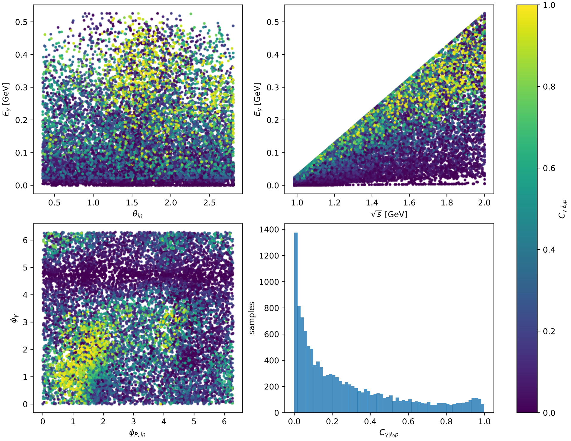
Phase-space scan: L massless lepton + Tx proton [LTx], max C_{\gamma|\ell_0 p}=0.9998
