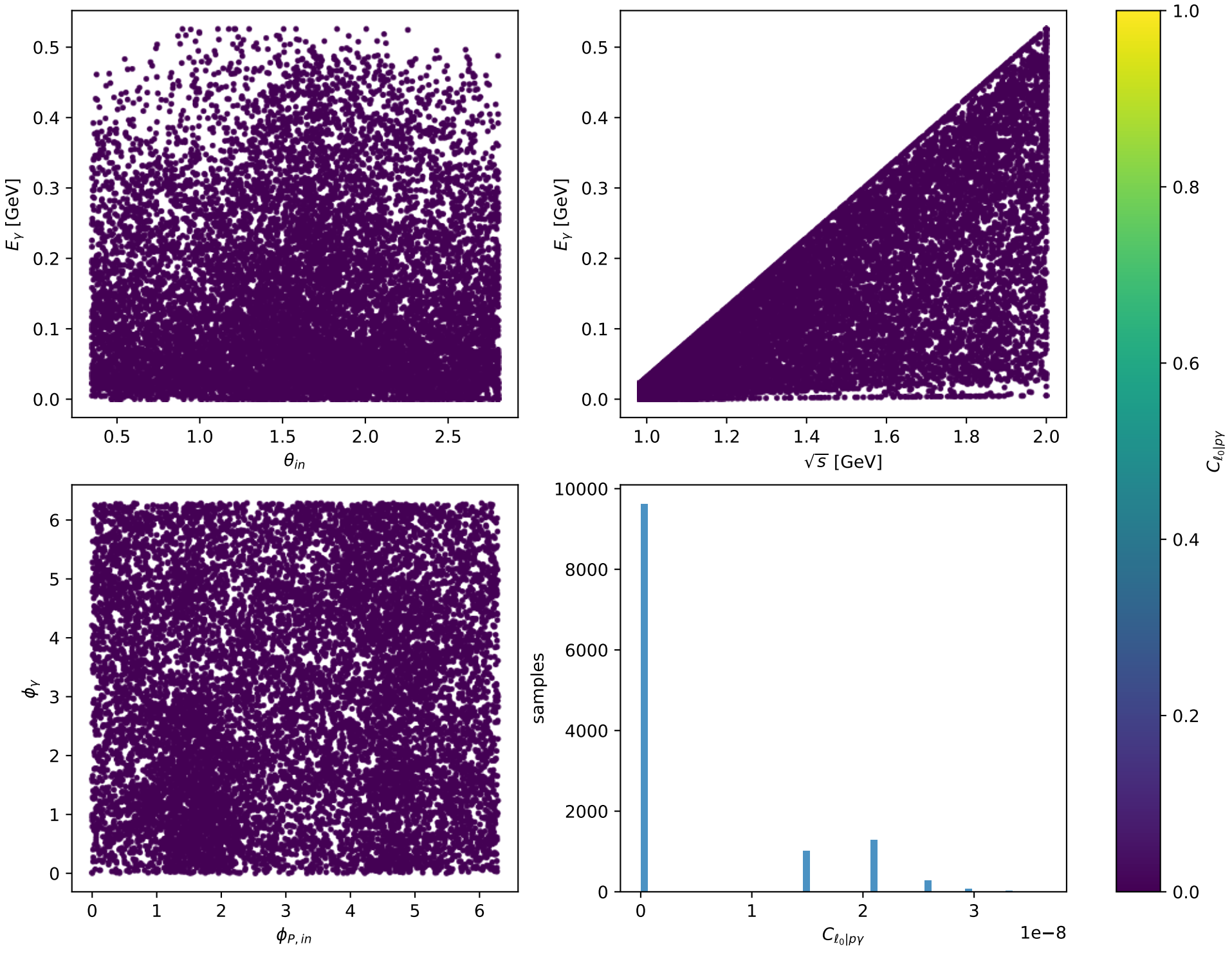
Phase-space scan: L massless lepton + Tx proton [LTx], max C_{\ell_0|p\gamma}=3.65\text{e-}08
