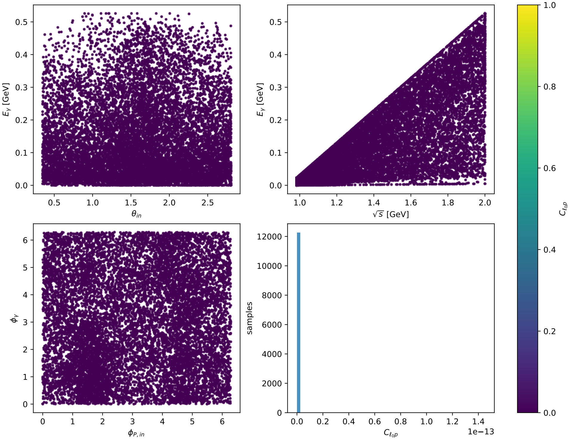
Phase-space scan: L massless lepton + Tx proton [LTx], max C_{\ell_0 p} = 1.4506\text{e-}13
