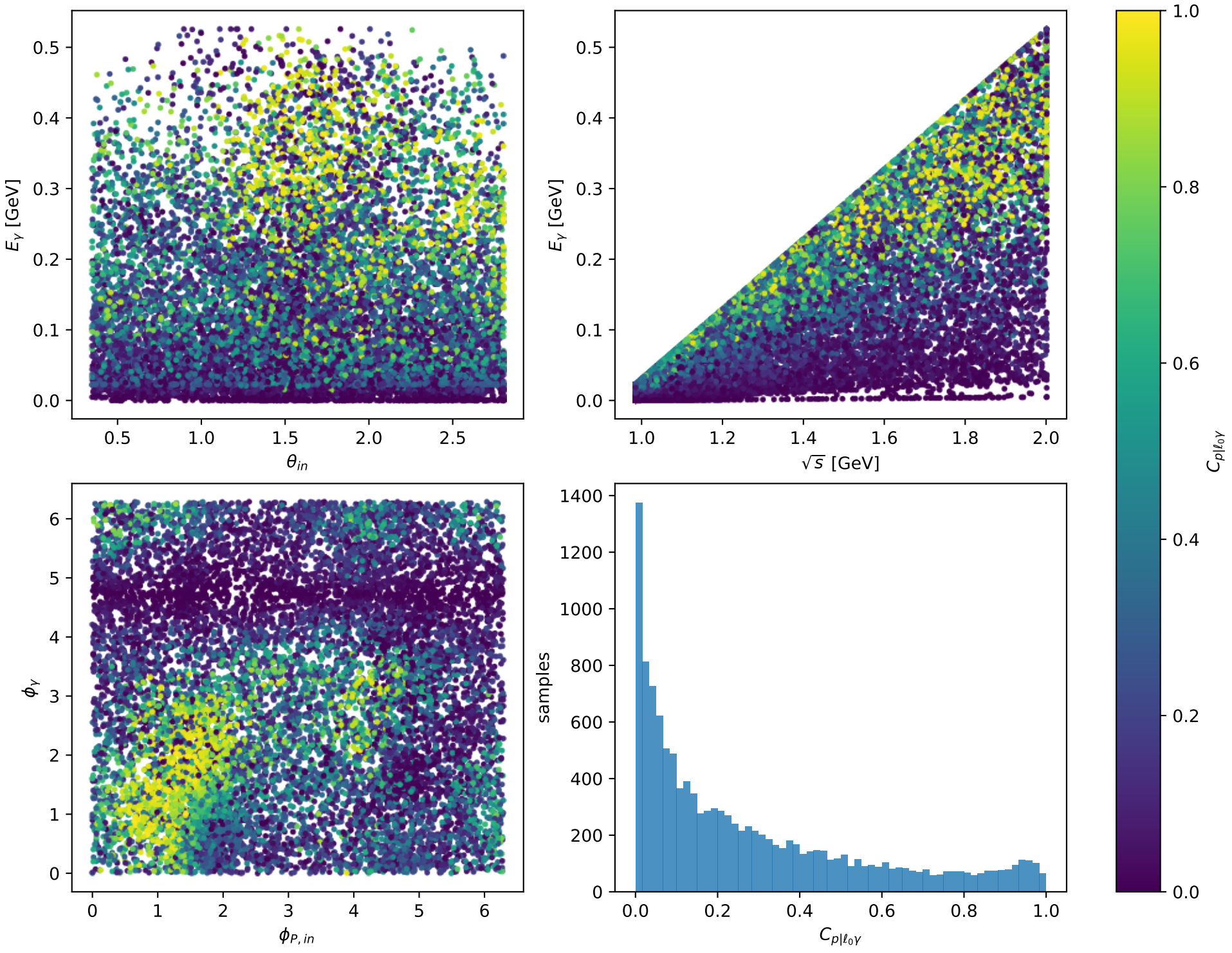
Phase-space scan: L massless lepton + Tx proton [LTx], max C_{p|\ell_0\gamma}=0.9998
