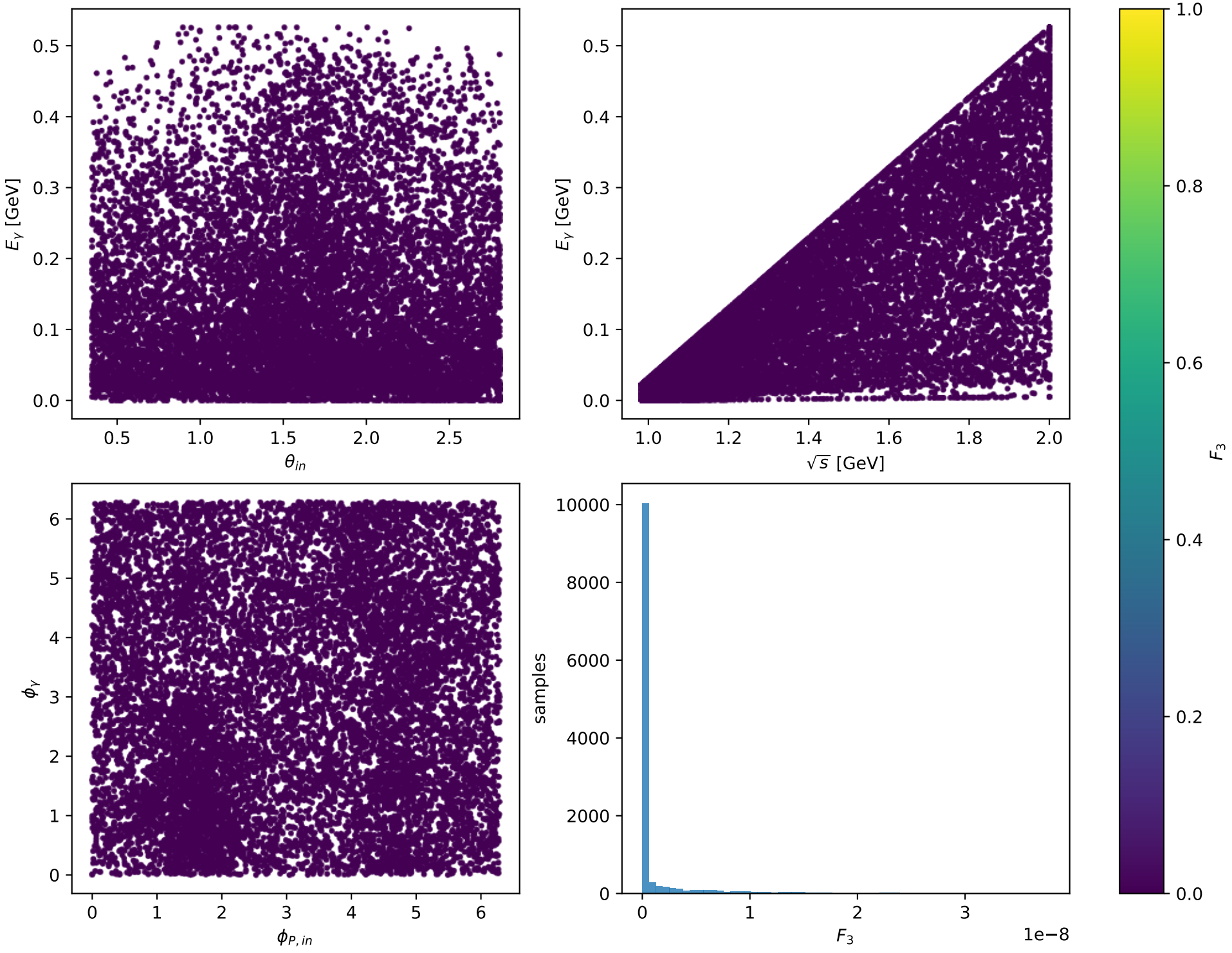
Phase-space scan: L massless lepton + Tx proton [LTx], max F_3=3.7831\text{e-}08
