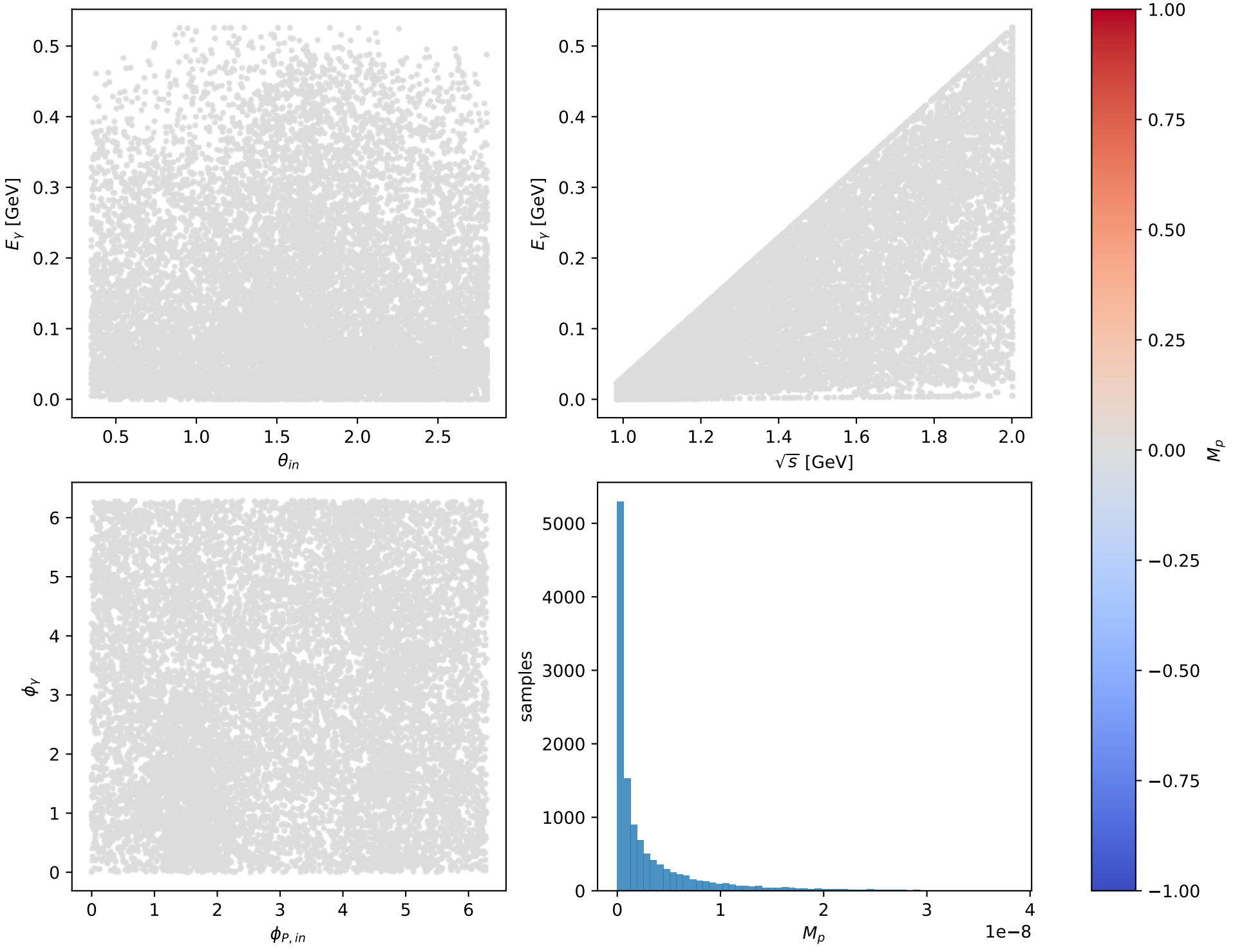
Phase-space scan: L massless lepton + Tx proton [LTx], max M_p=3.8235\text{e-}08
