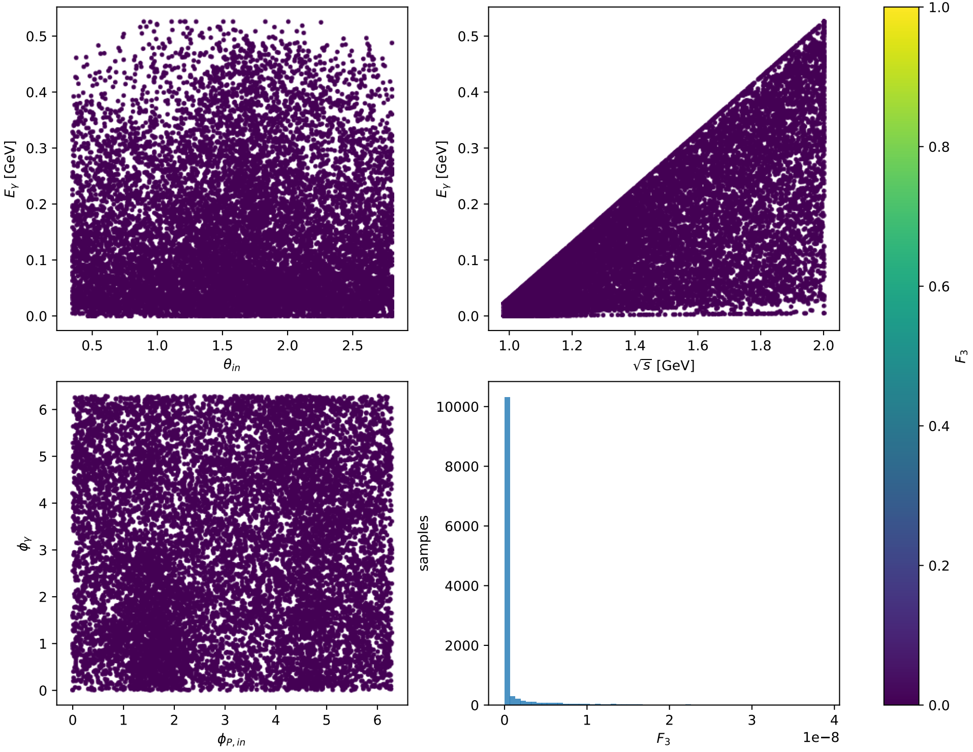
Phase-space scan: L massless lepton + Ty proton [LTy], max F_3=3.8688\text{e-}08
