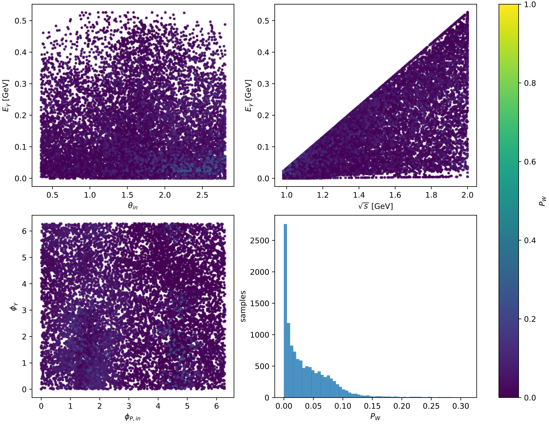
Phase-space scan: L massless lepton + Ty proton [LTy], max P_W=0.31143
