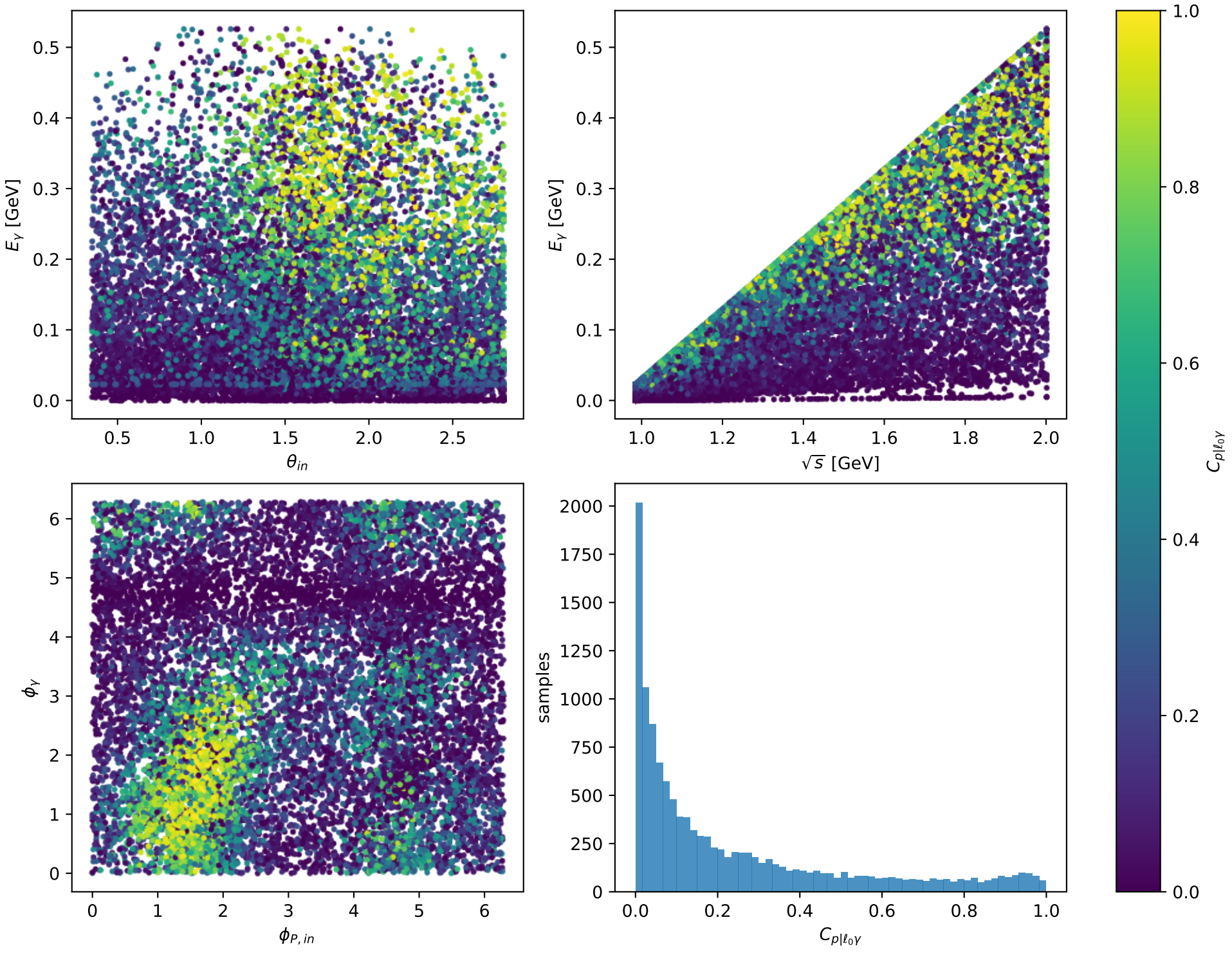
Phase-space scan: L massless lepton + Ty proton [LTy], max C_{p|\ell_0\gamma}=0.99934
