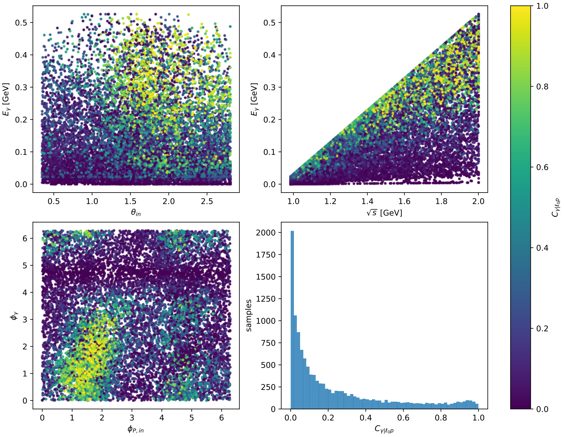
Phase-space scan: L massless lepton + Ty proton [LTy], max C_{\gamma|\ell_0 p}=0.99934
