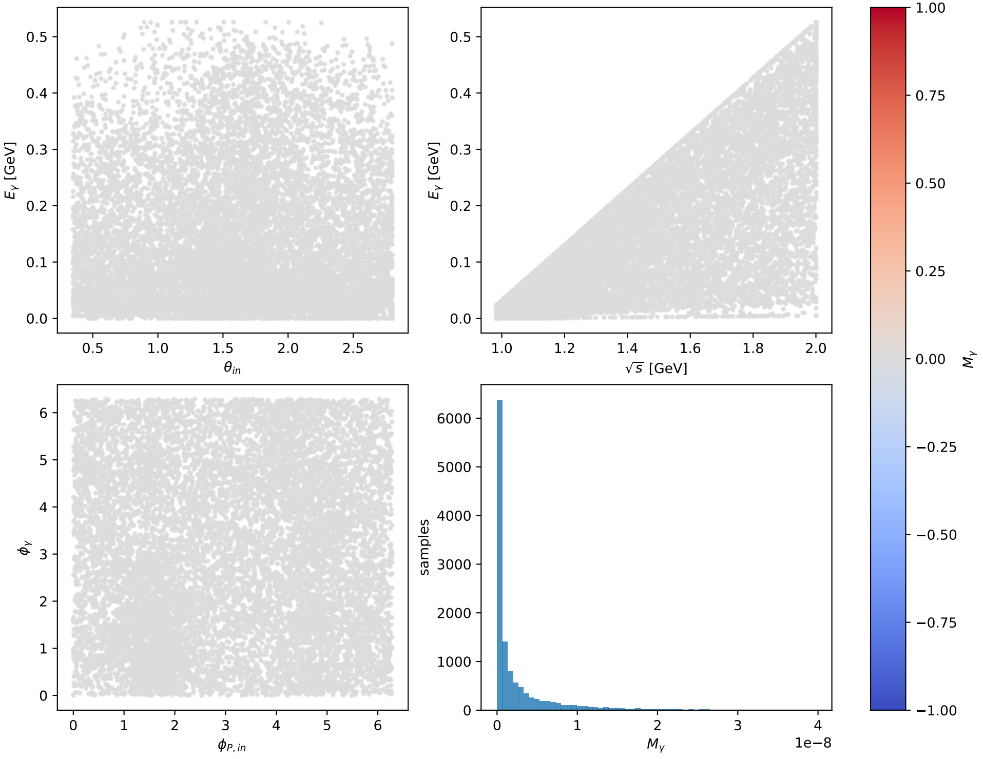
Phase-space scan: L massless lepton + Ty proton [LTy], max M_\gamma=3.9737\text{e-}08
