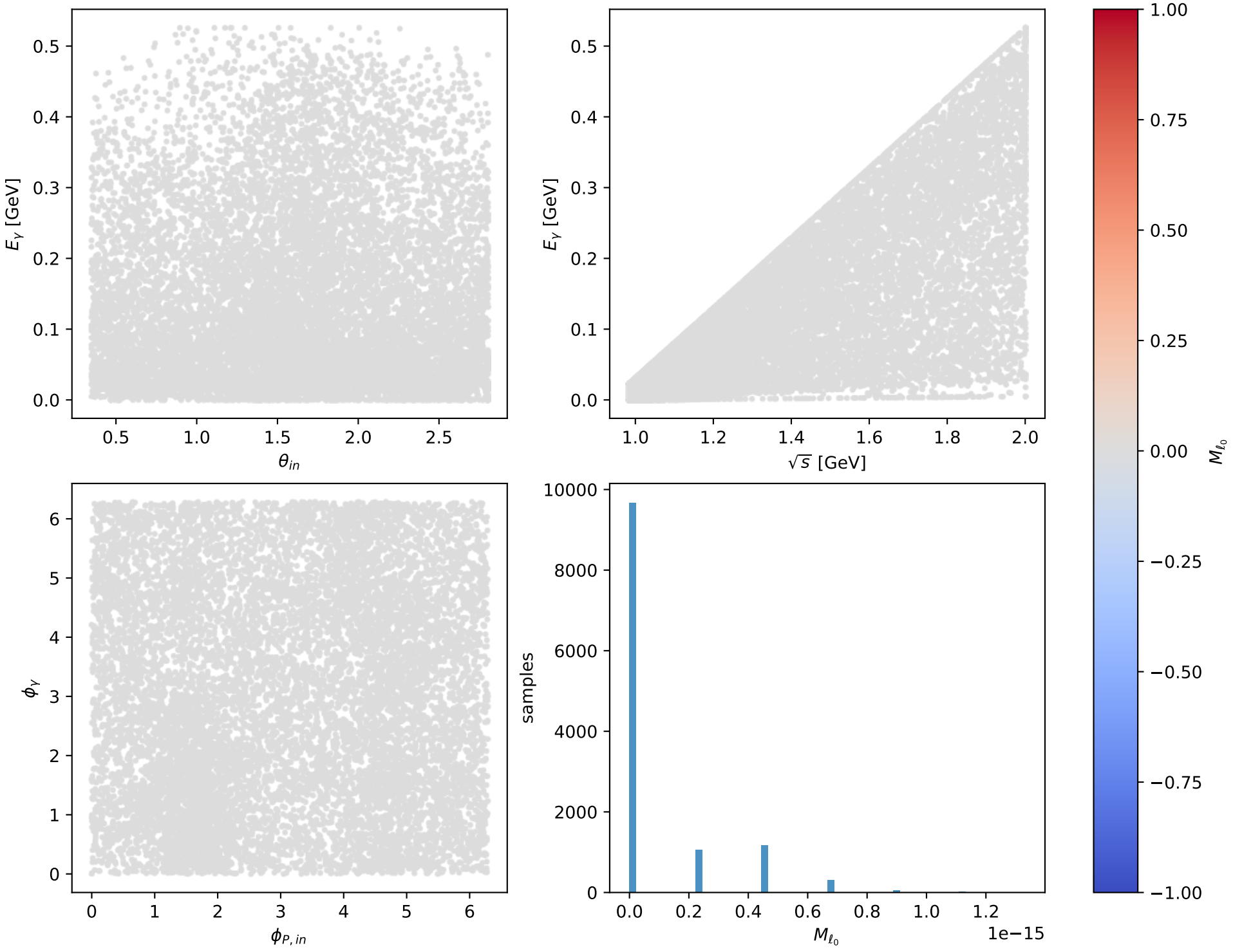
Phase-space scan: L massless lepton + Ty proton [LTy], max M_{\ell_0}=1.3323\text{e-15}
