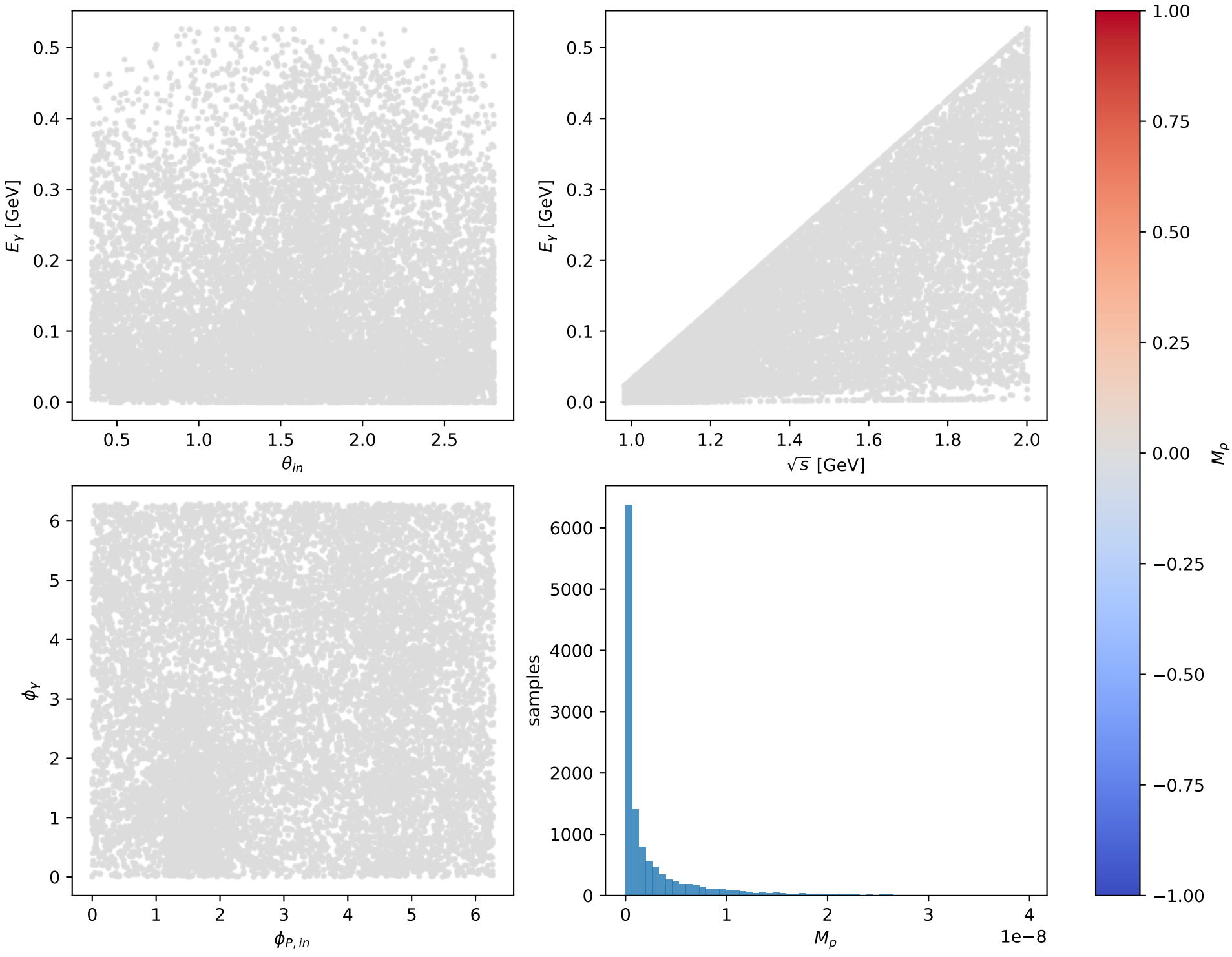
Phase-space scan: L massless lepton + Ty proton [LTy], max M_p=3.9737\text{e-}08
