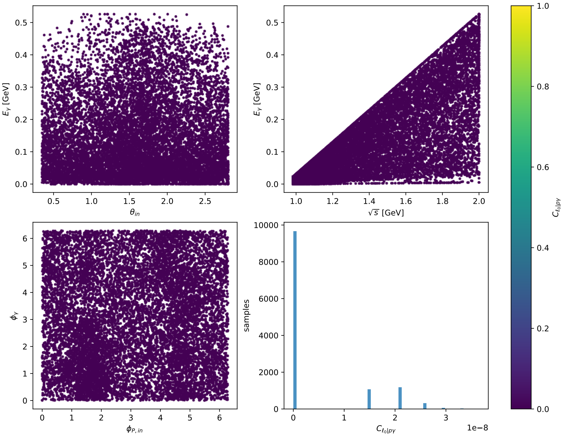
Phase-space scan: L massless lepton + Ty proton [LTy], max C_{\ell_0|p\gamma}=3.65\text{e-}08
