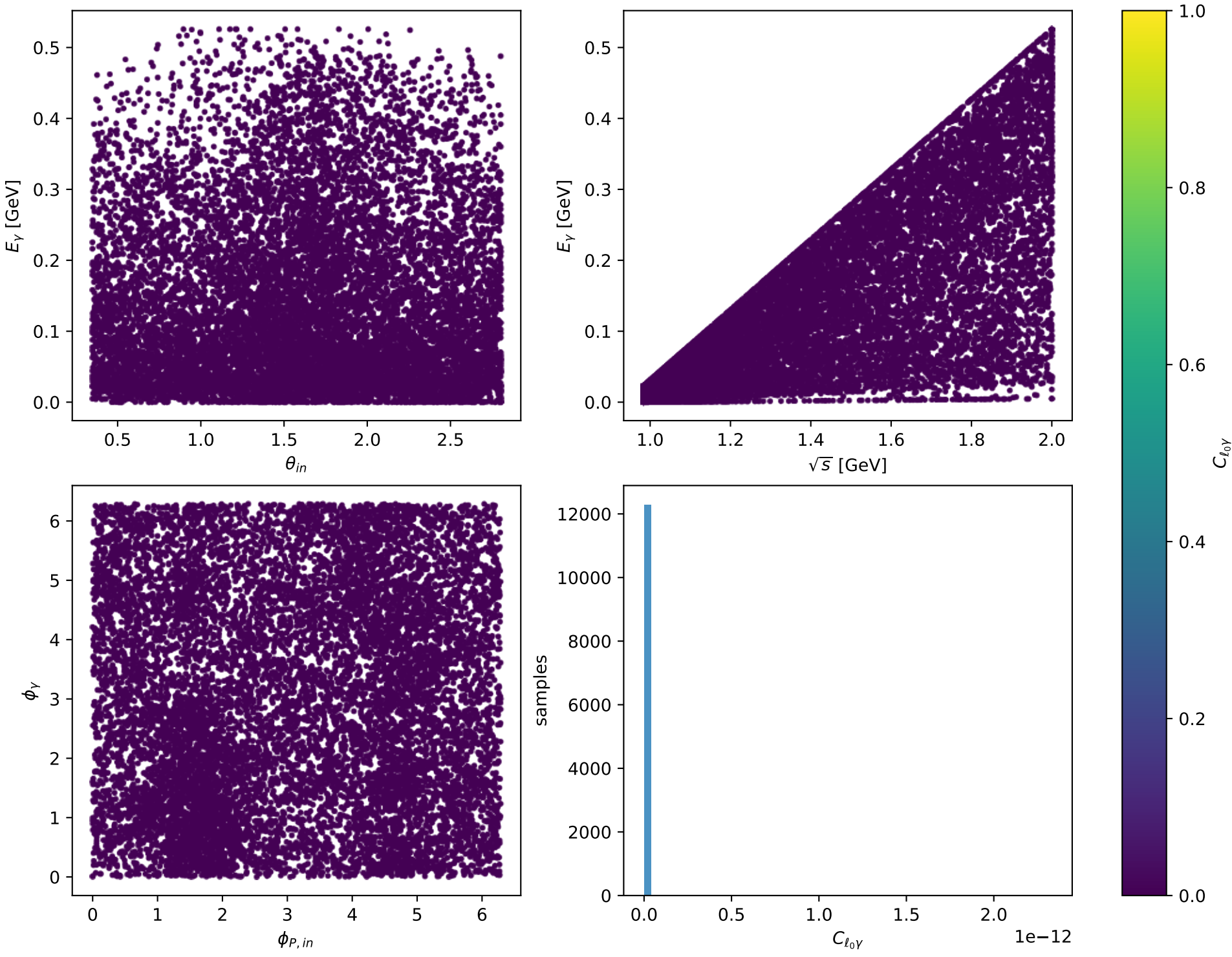
Phase-space scan: L massless lepton + Ty proton [LTy], max C_{\ell_0\gamma}=2.3317\text{e-}12
