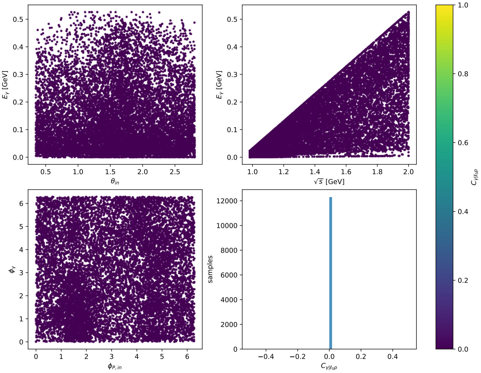
Phase-space scan: L proton[L_proton], max C_{\gamma|\ell_0 p}=0
