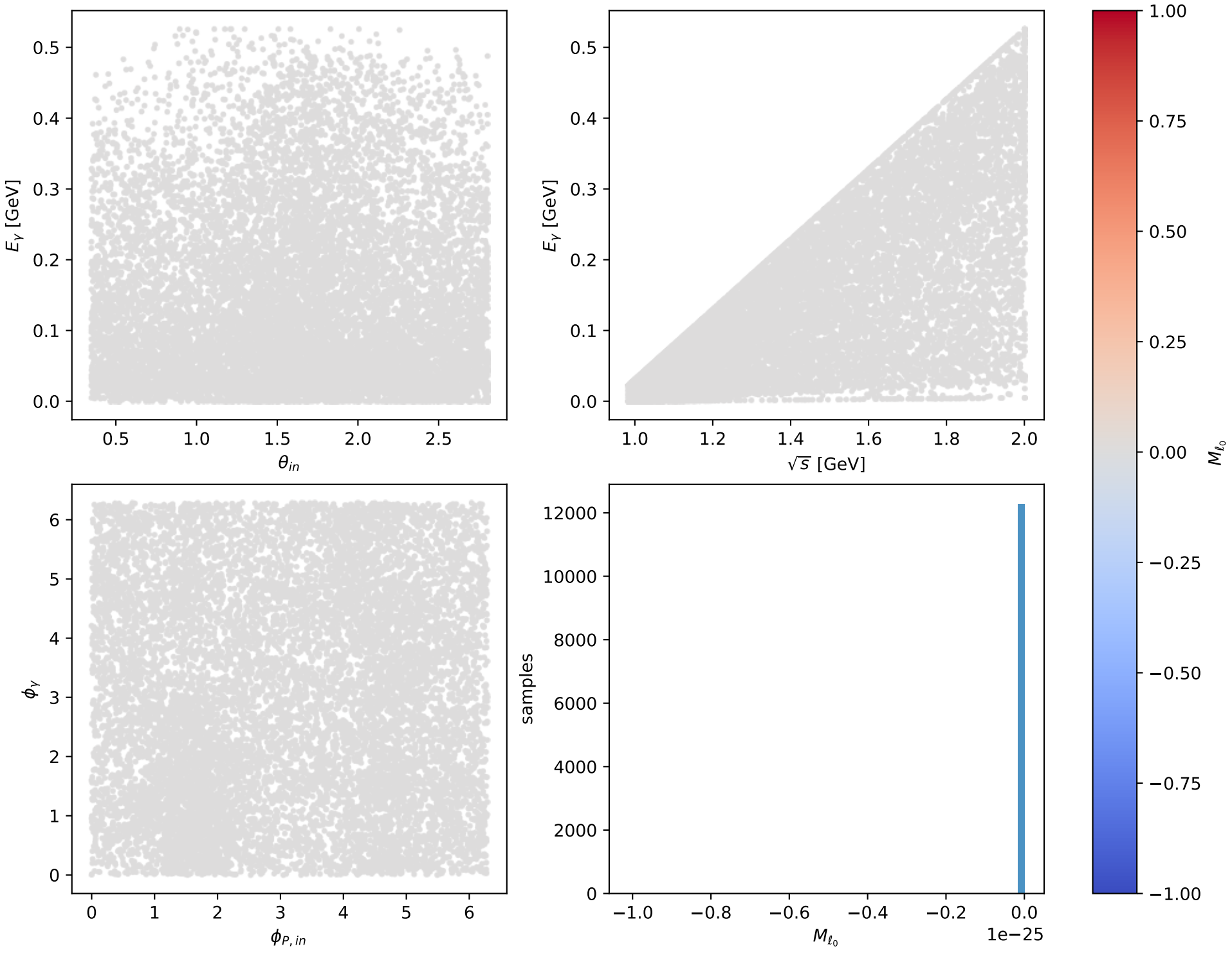
Phase-space scan: L proton [L_proton], max M_{\ell_0} = -0
