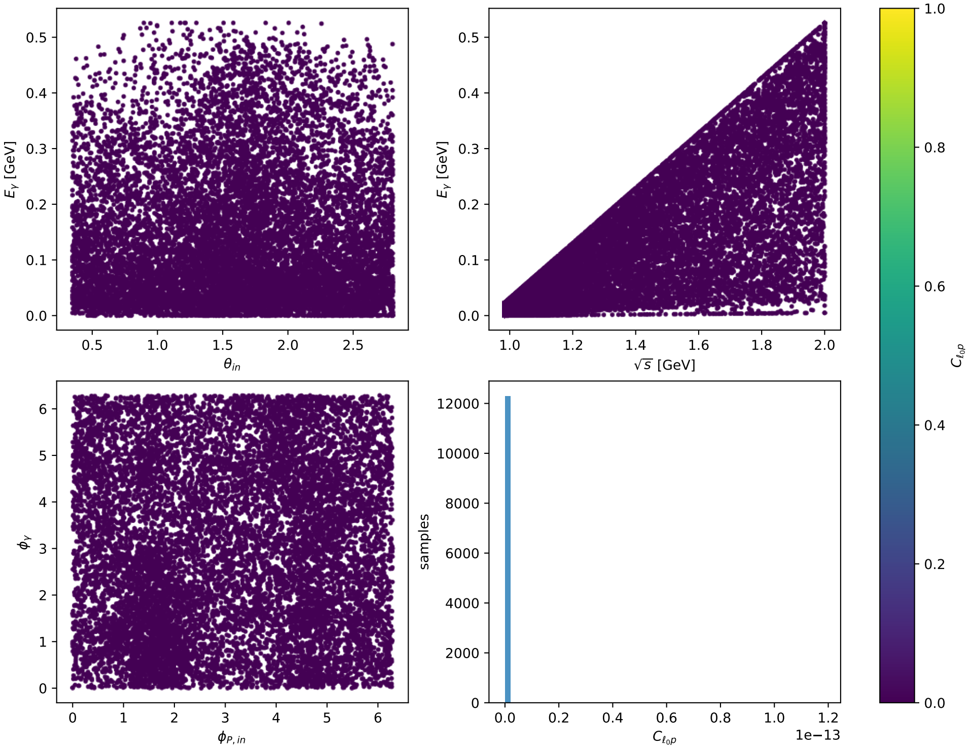
Phase-space scan: L proton [ L_{\text{proton}} ], max C_{\ell_0 p} = 1.1867\text{e-}13
