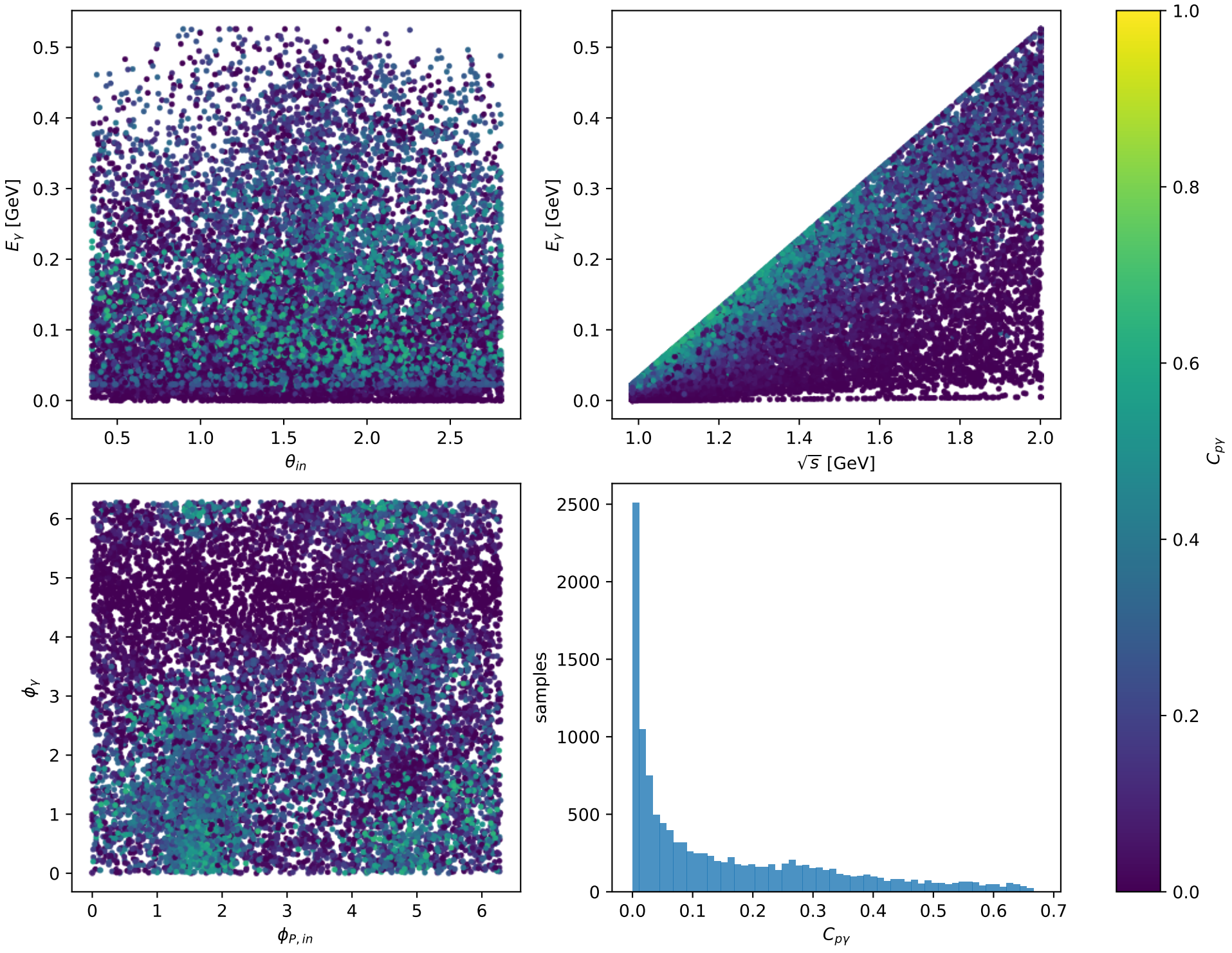
Phase-space scan: L proton [L_proton], max C_{p\gamma} =0.67783
