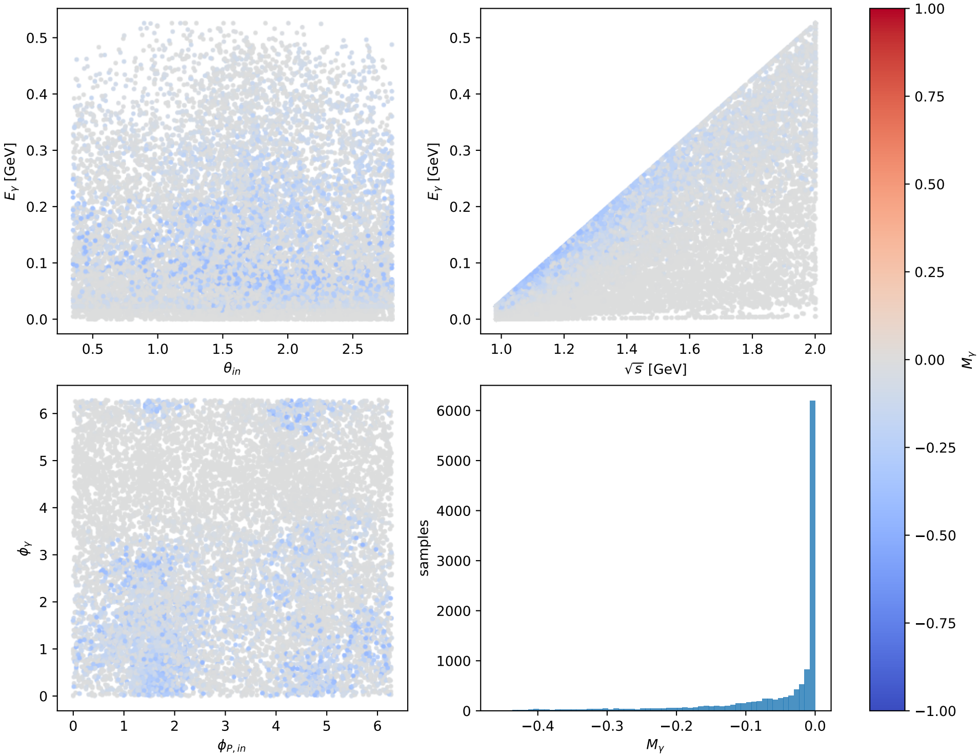
Phase-space scan: L proton [L_proton], max M_Y = -3.035\text{e-}13
