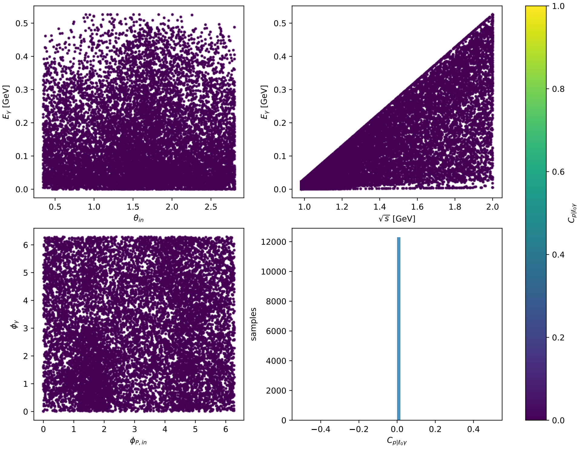
Phase-space scan: L proton[L_proton], max C_{p|\ell_0\gamma}=0
