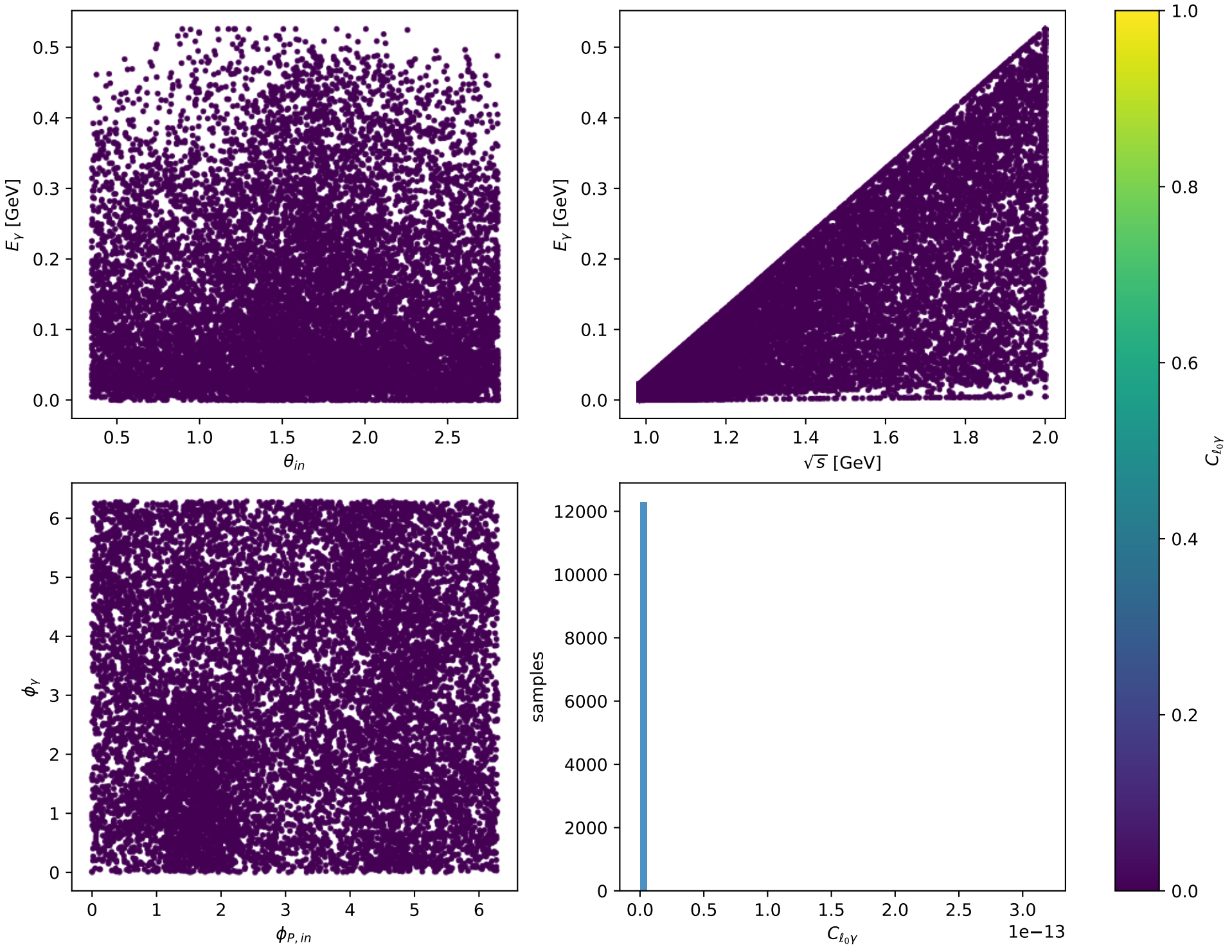
Phase-space scan: L proton [ L_{\text{proton}} ], max C_{\ell_0\gamma}=3.1767\text{e-13}
