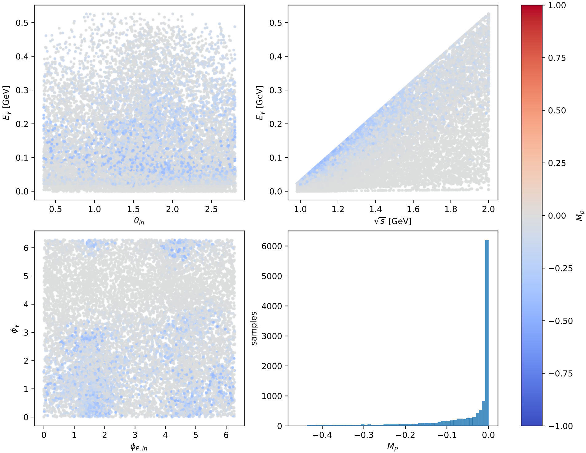
Phase-space scan: L proton [L_proton], max M_p = -3.035 \times 10^{-13}
