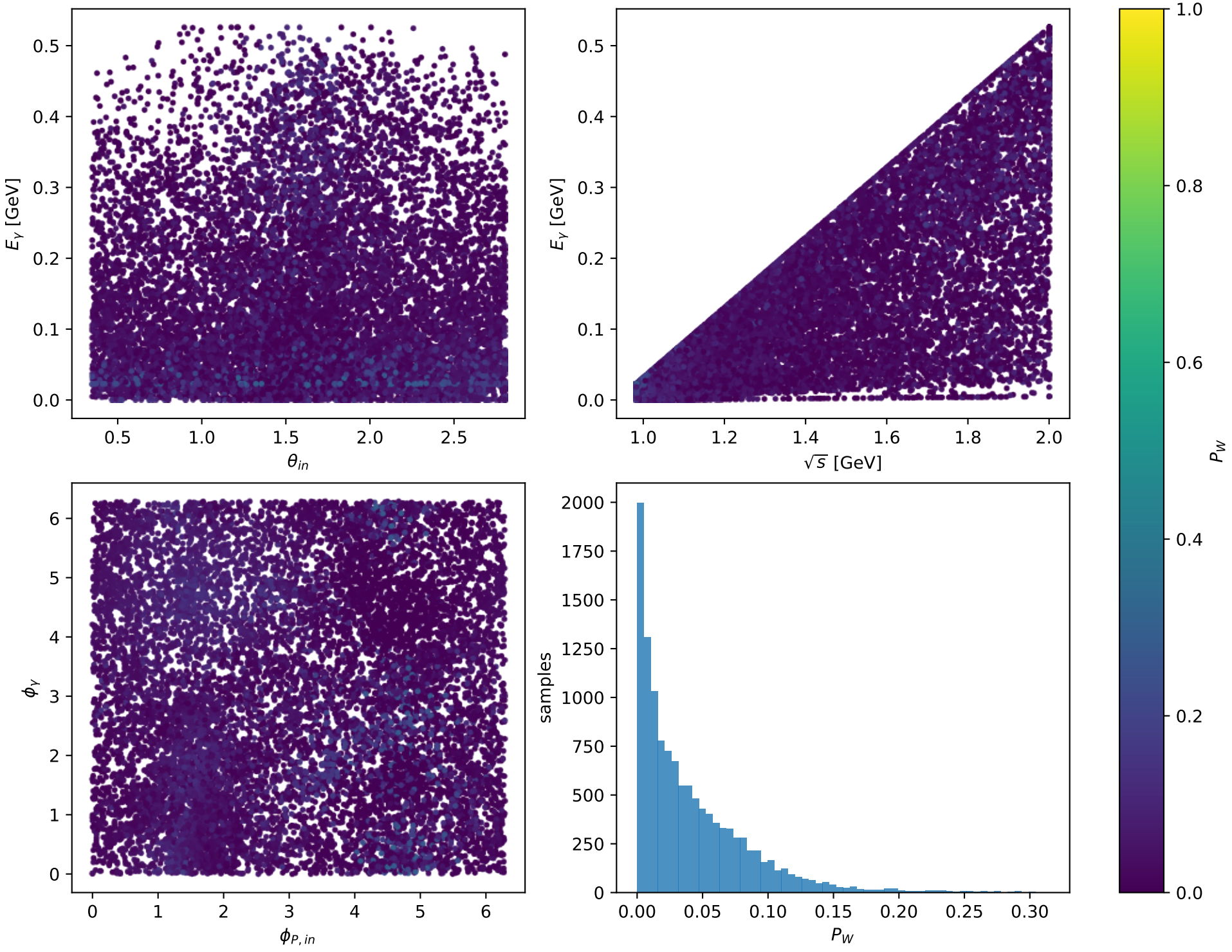
Phase-space scan: L proton [L_proton], max P_W=0.31469
