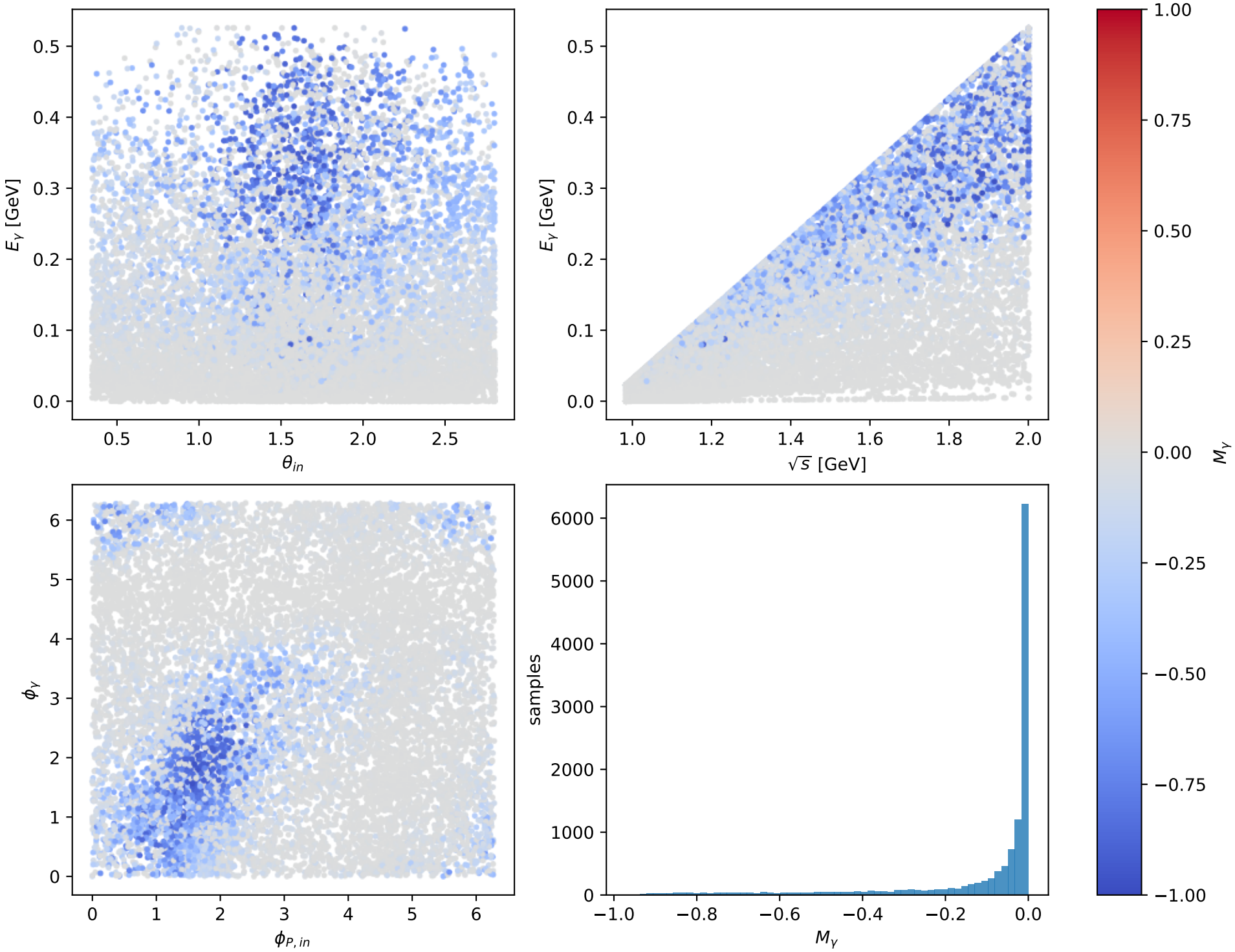
Phase-space scan: Tx proton [Tx_proton], max M_\gamma = -4.105\text{e-}11
