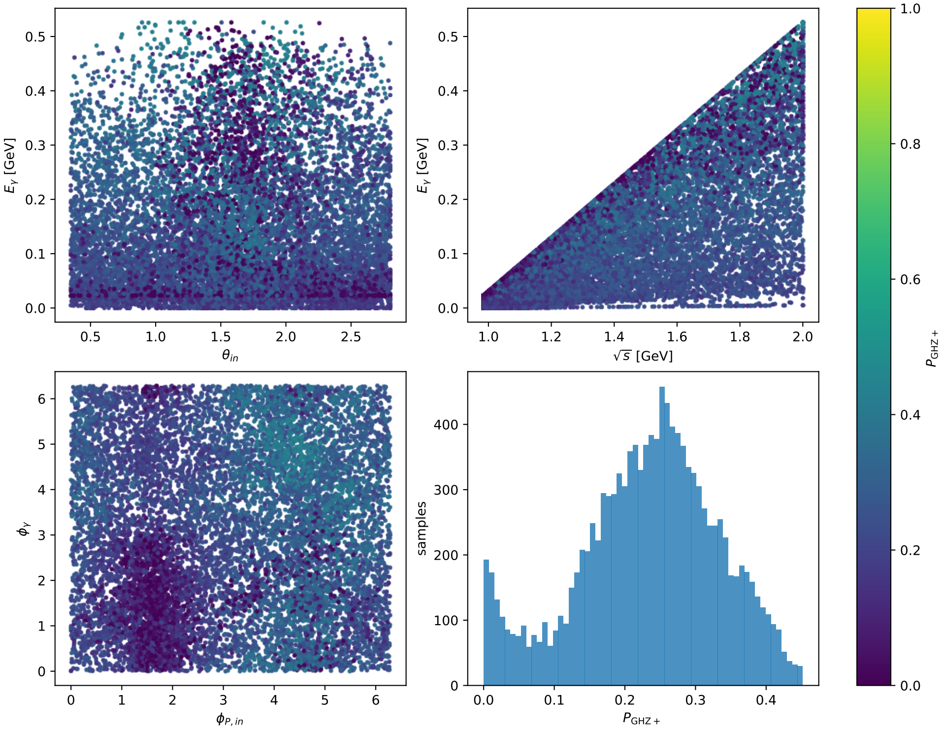
Phase-space scan: Tx proton [Tx_proton], max P_{\text{GHZ}+}=0.45193
