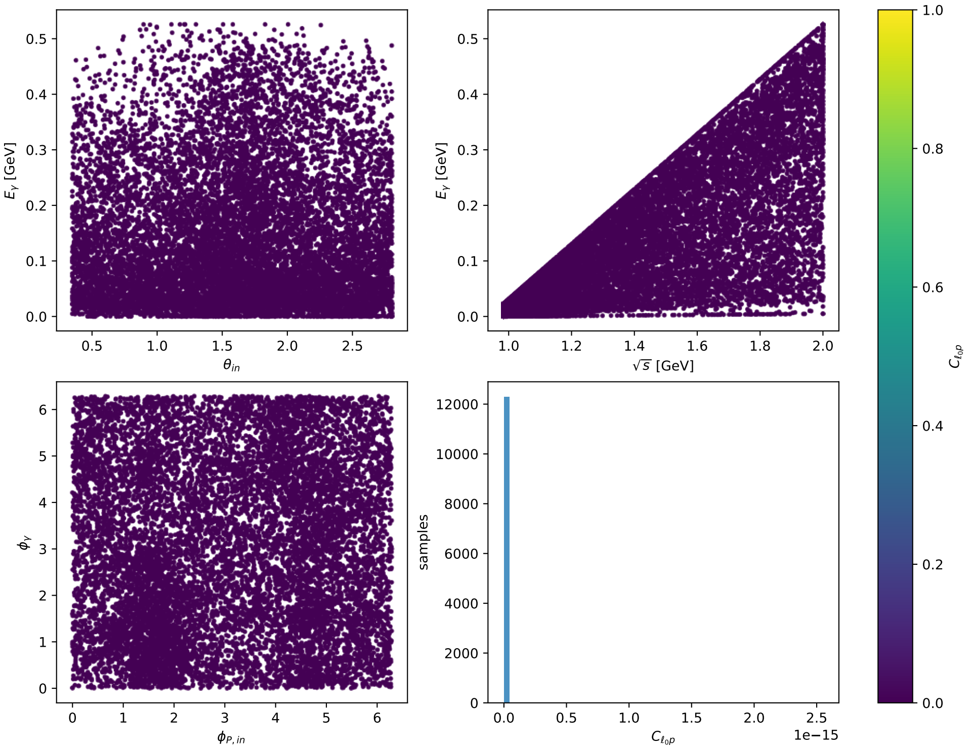
Phase-space scan: Tx proton [Tx_proton], max C_{\ell_0 p} = 2.55\text{e-15}
