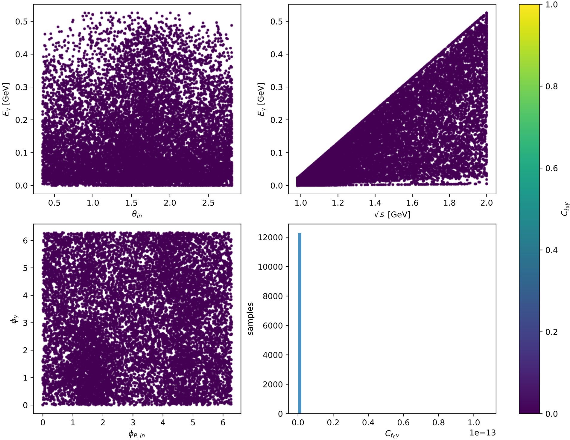
Phase-space scan: Tx proton [Tx_proton], max C_{\ell_0\gamma}=1.0731\text{e-}13
