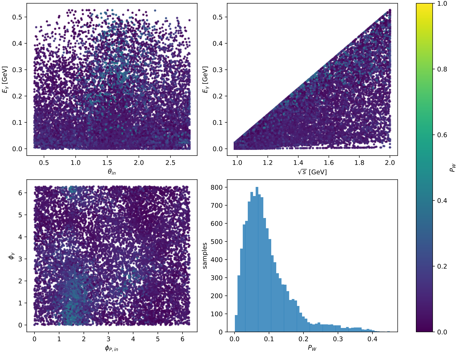
Phase-space scan: Tx proton [Tx_proton], max P_W=0.45064
