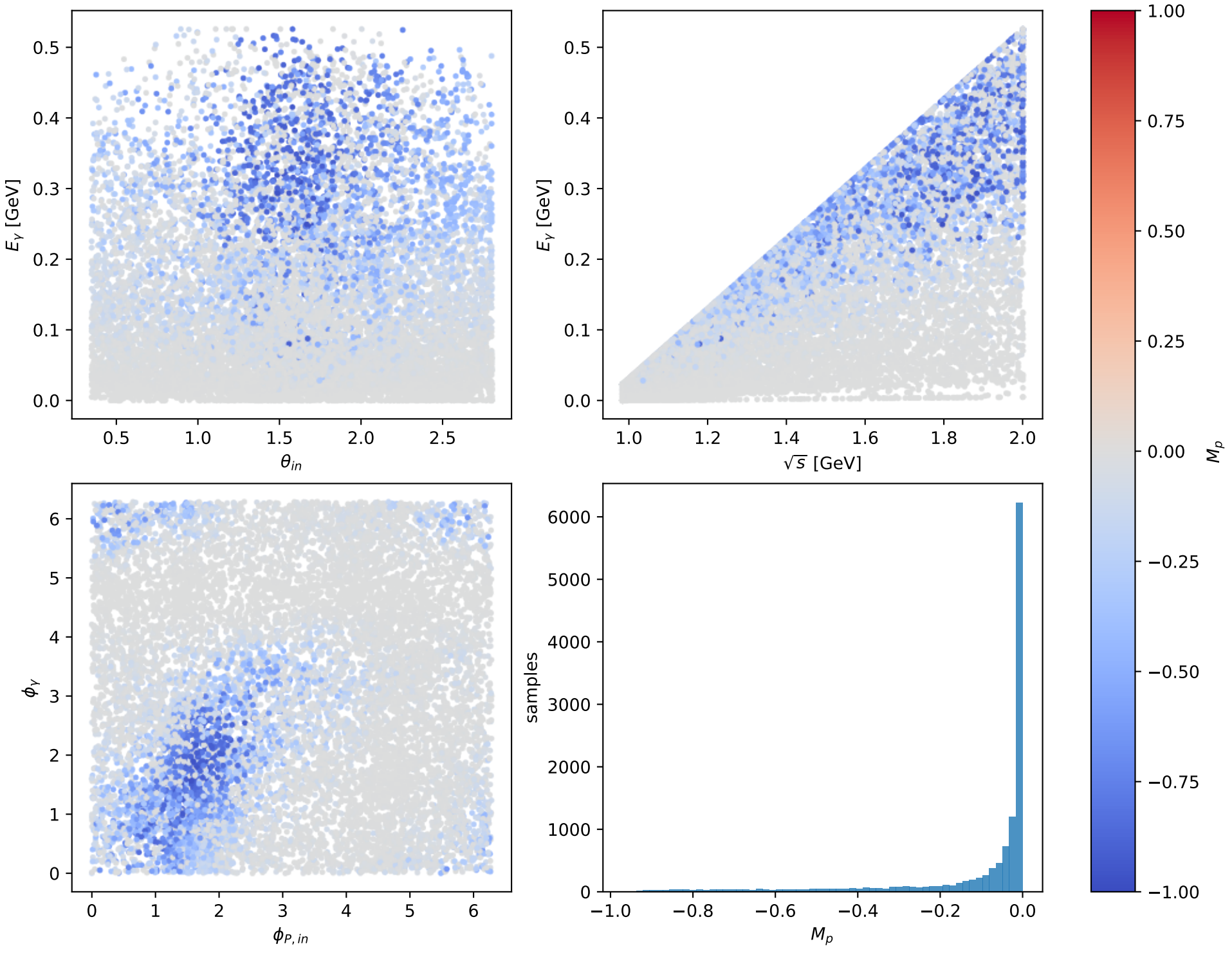
Phase-space scan: Tx proton [Tx_proton], max M_p = -4.105\text{e-}11
