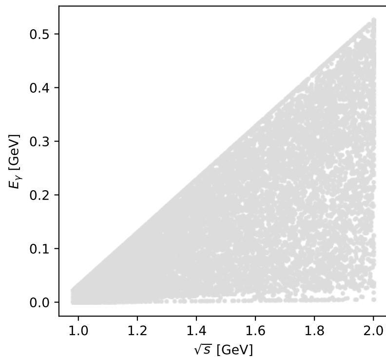
Phase-space scan: Tx proton [Tx_proton], max M_{\ell_0} = -0
