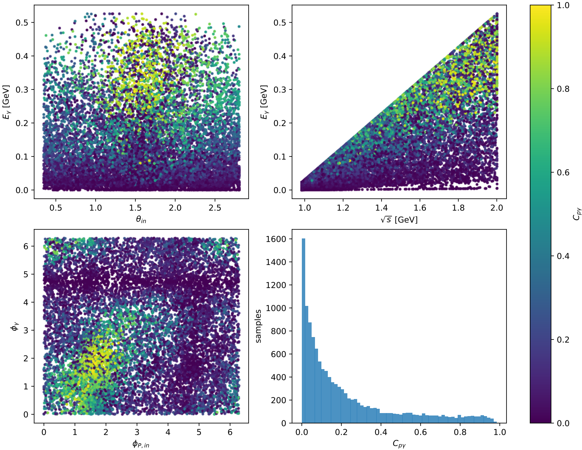
Phase-space scan: Tx proton [Tx_proton], max C_{p\gamma}=0.98479
