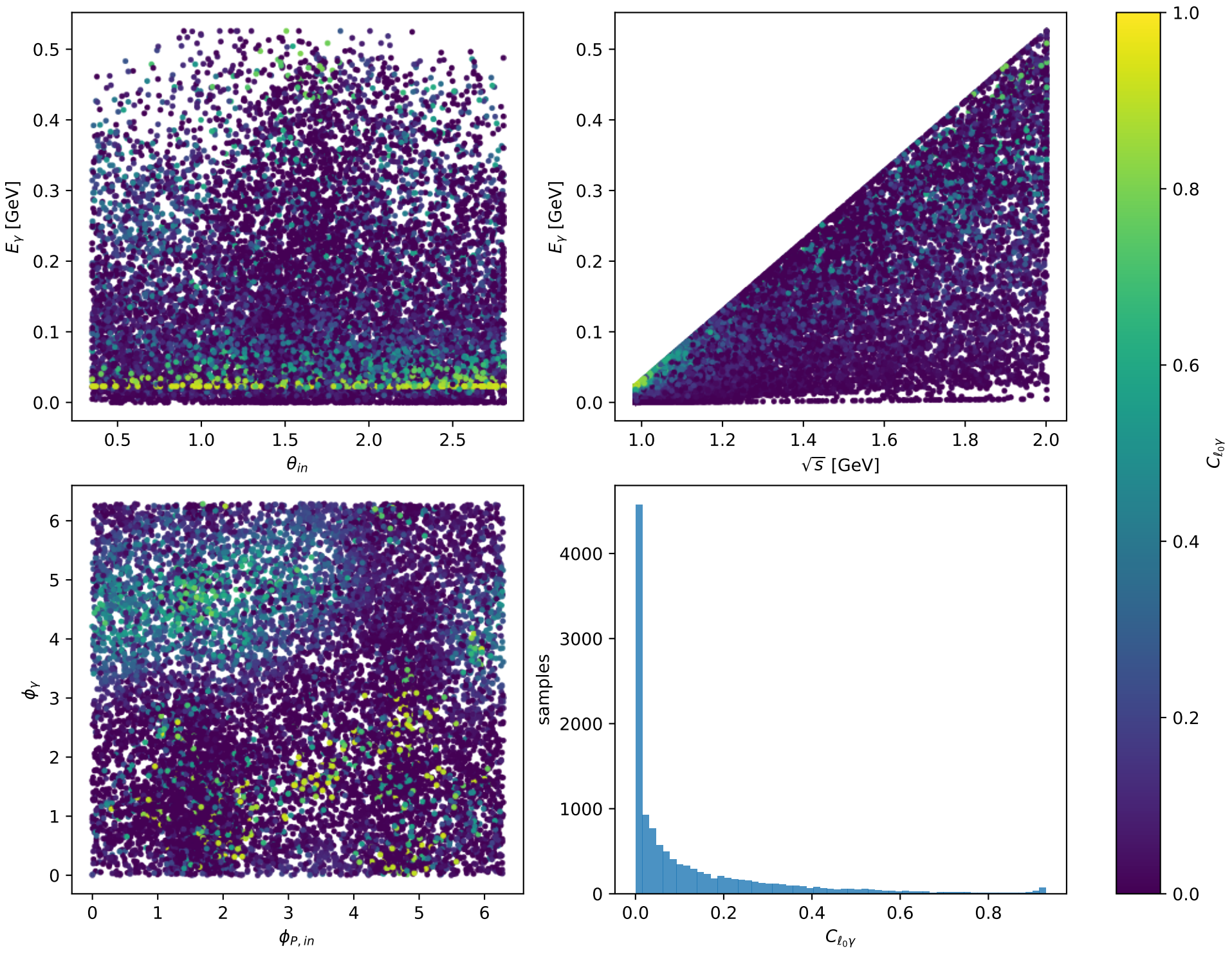
Phase-space scan: Ty massless lepton [Ty_electron], max C_{\ell_0\gamma}=0.93071
