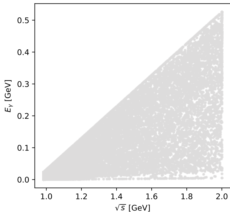
Phase-space scan: Ty massless lepton [Ty_electron], max M_p=-0
