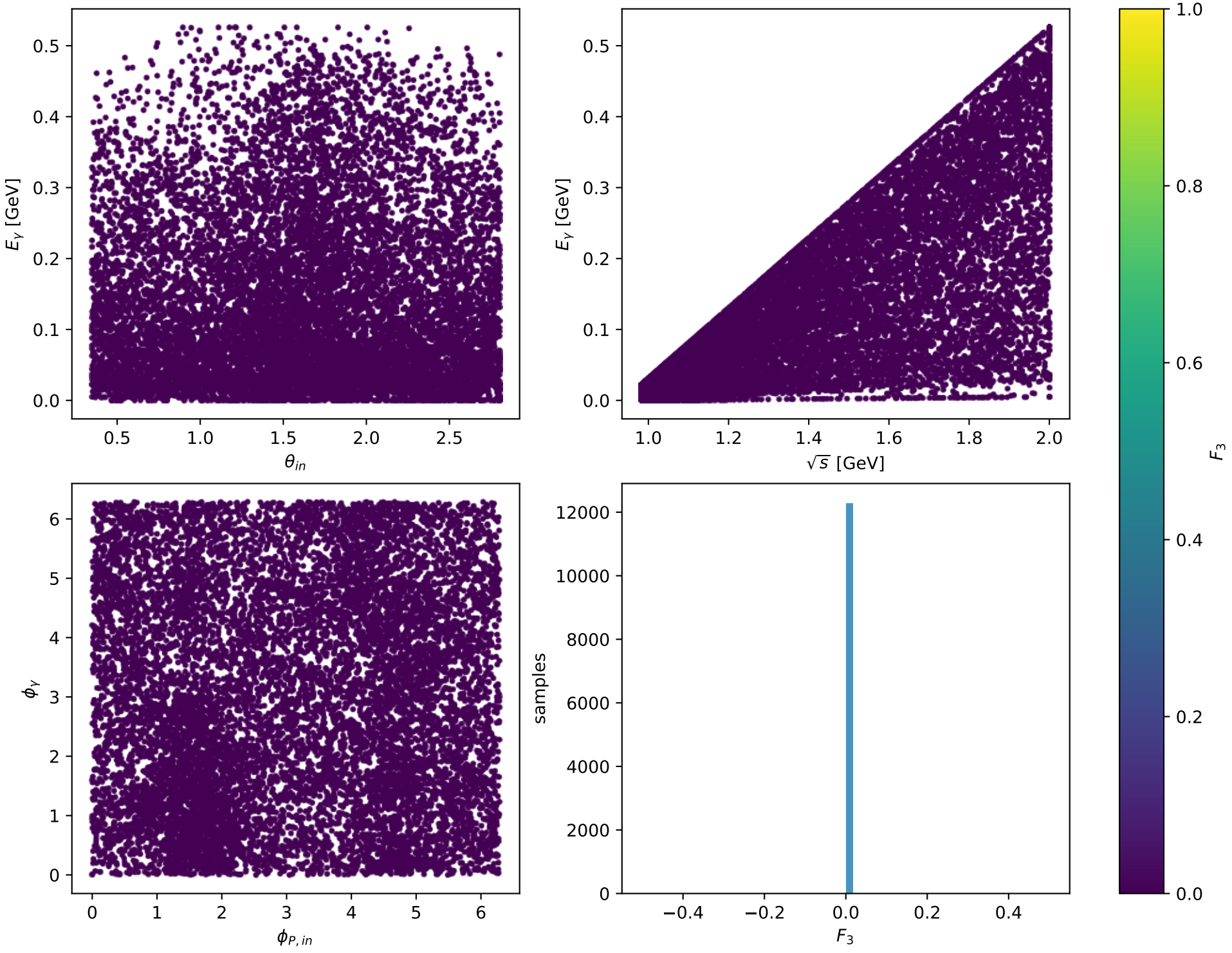
Phase-space scan: Ty massless lepton [Ty_electron], max F_3=0
