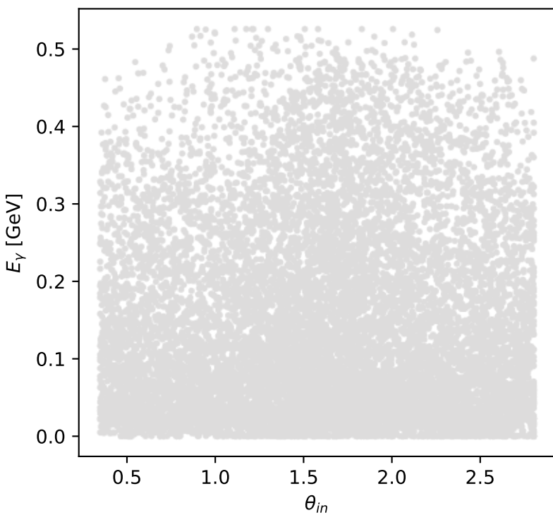
Phase-space scan: Ty massless lepton [Ty_electron], max M_p=-0
