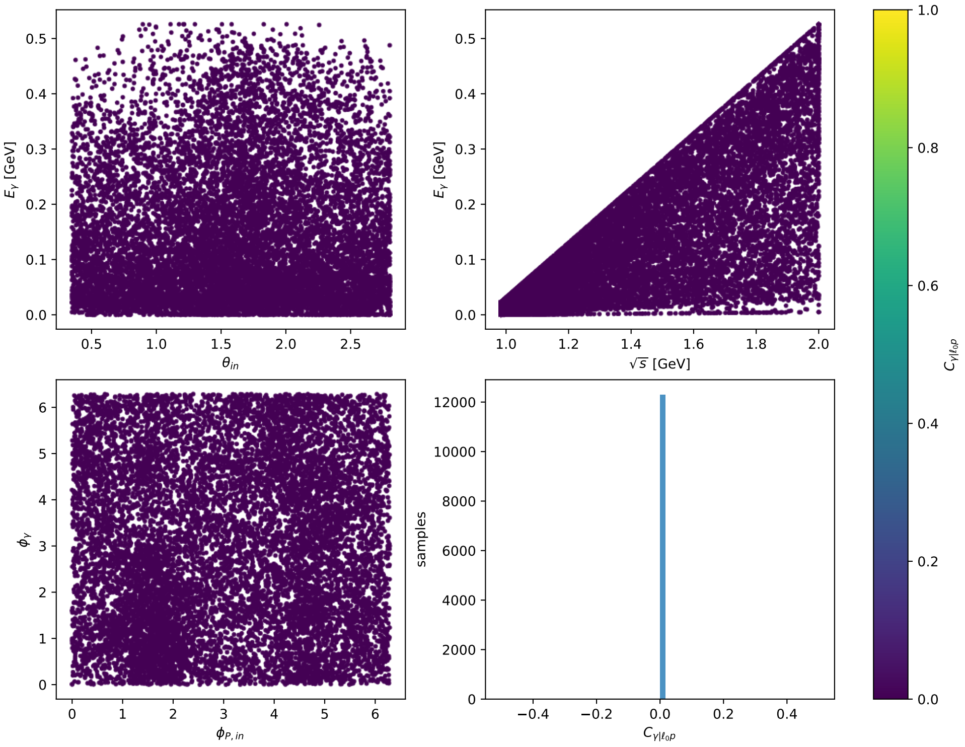
Phase-space scan: Ty massless lepton [Ty_electron], max C_{\gamma|\ell op}=0
