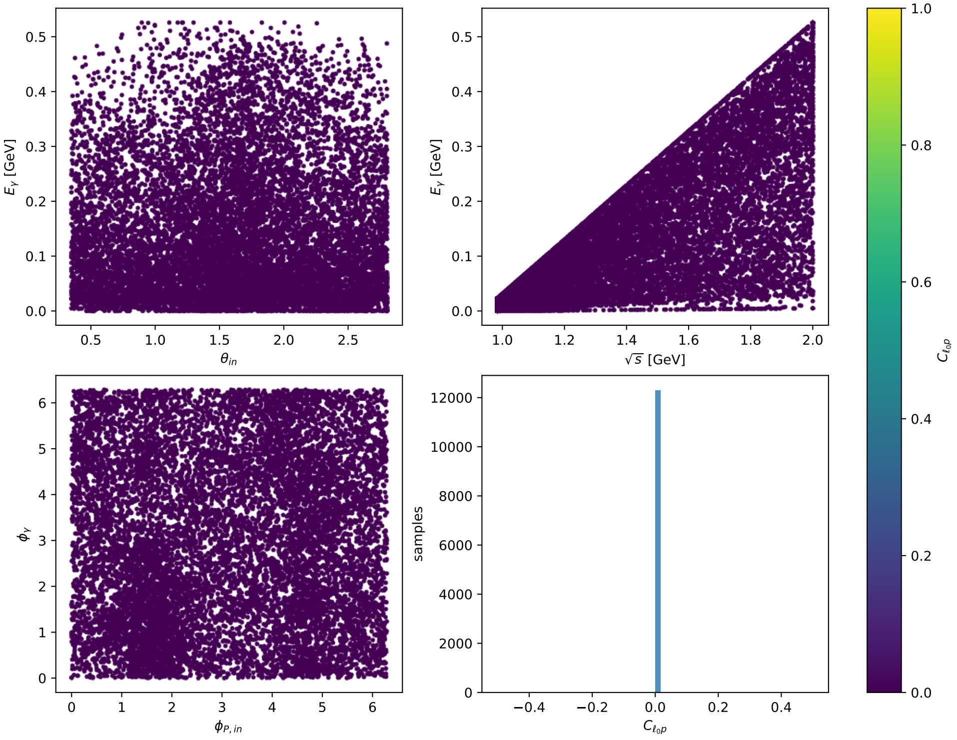
Phase-space scan: Ty massless lepton [Ty_electron], max C_{\ell_0 p}=0
