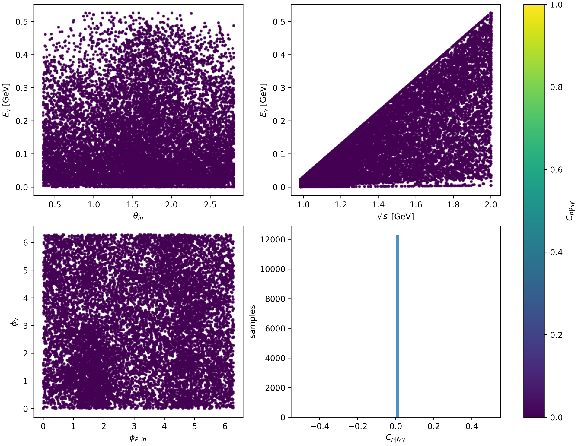
Phase-space scan: Ty massless lepton [Ty_electron], max C_{p|\ell_0\gamma}=0
