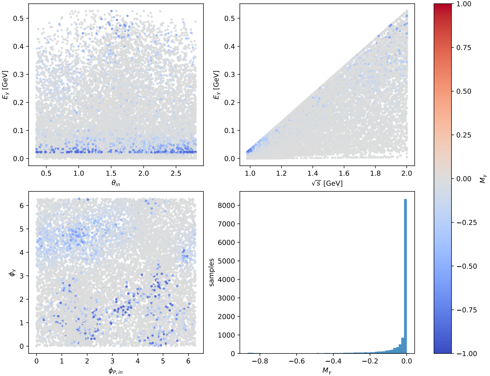
Phase-space scan: Ty massless lepton [Ty_electron], max M_\gamma = -0
