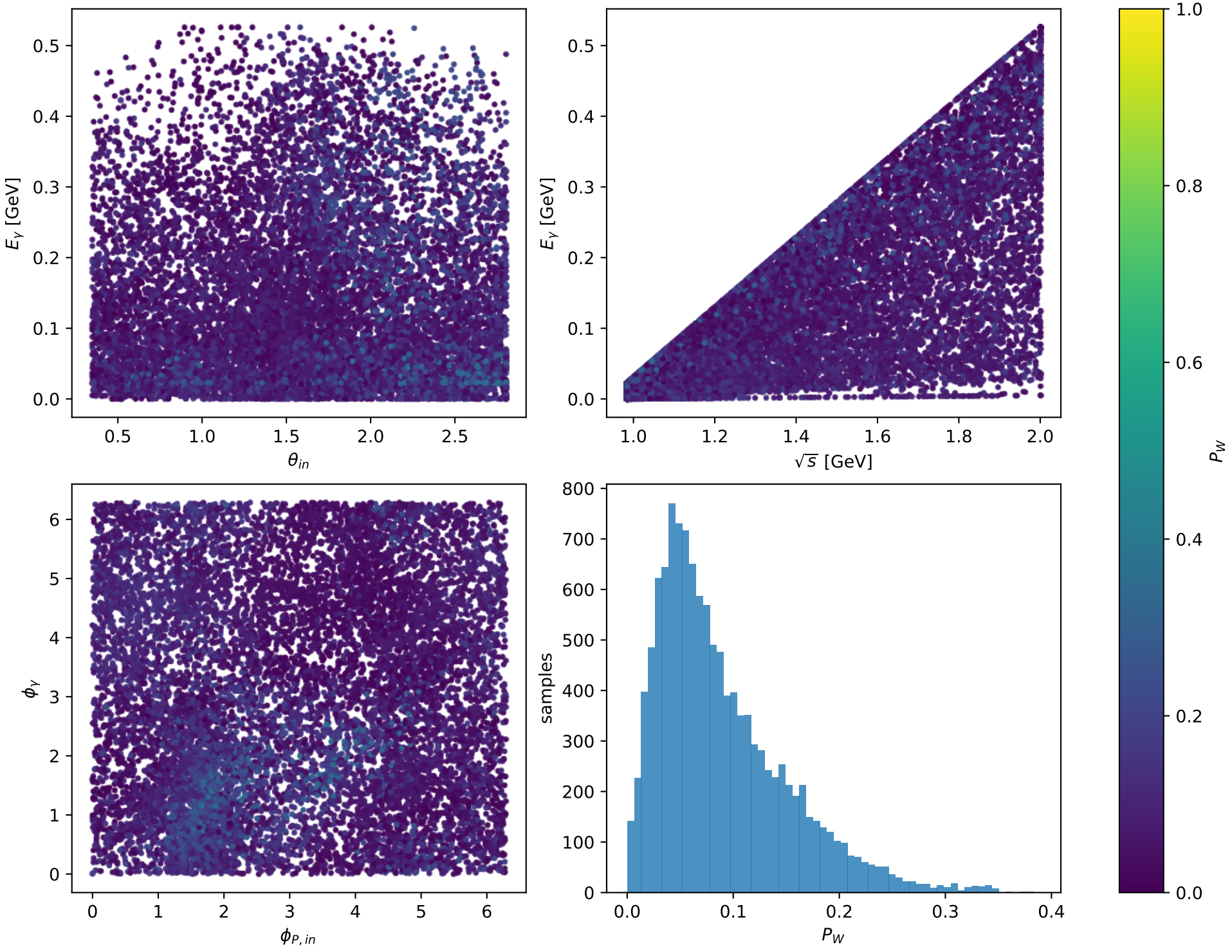
Phase-space scan: Ty massless lepton [Ty_electron], max P_W=0.38938
