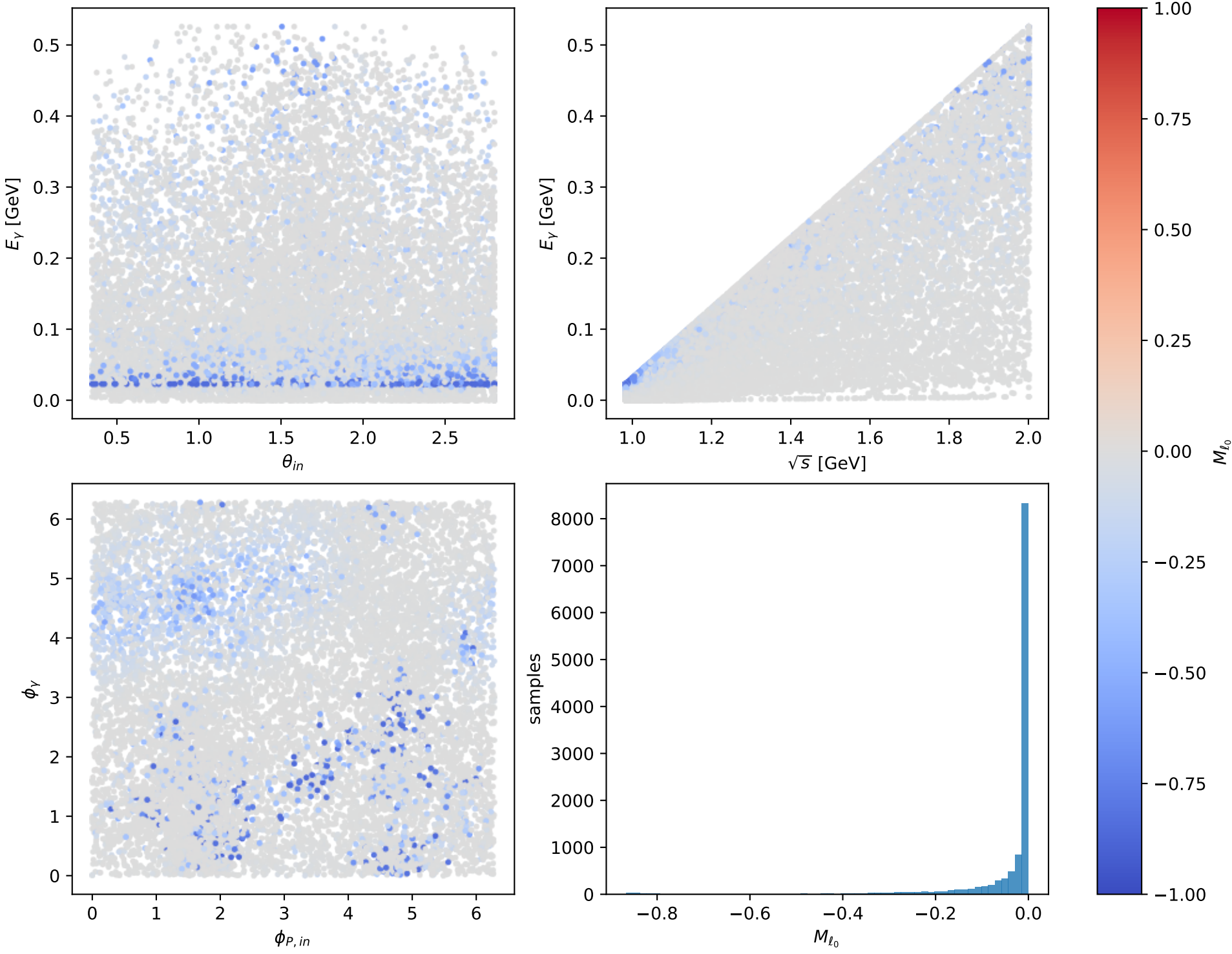
Phase-space scan: Ty massless lepton [Ty_electron], max M_{\ell_0} = -0
