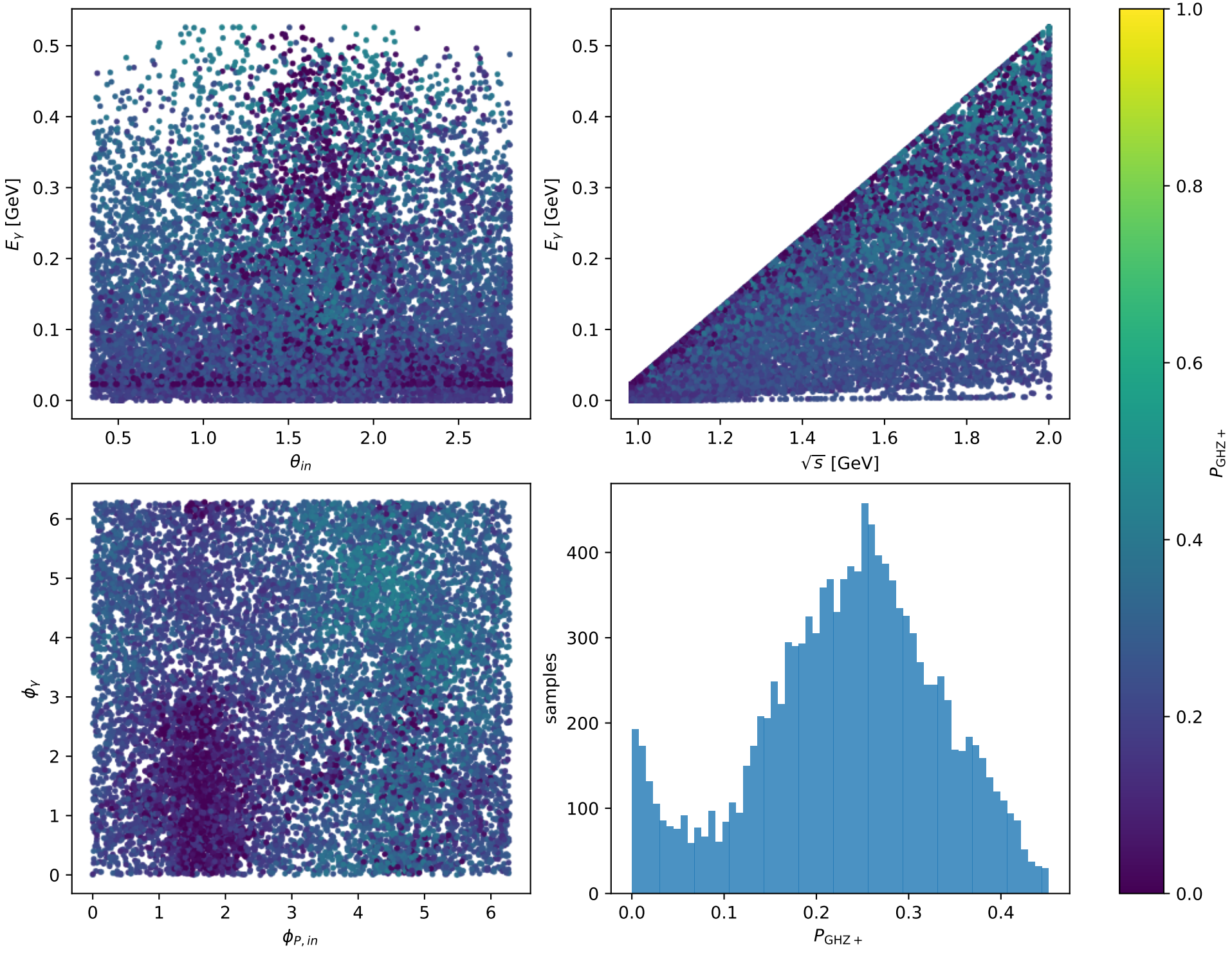
Phase-space scan: Ty massless lepton [Ty_electron], max P_{\text{GHZ}+}=0.45193
