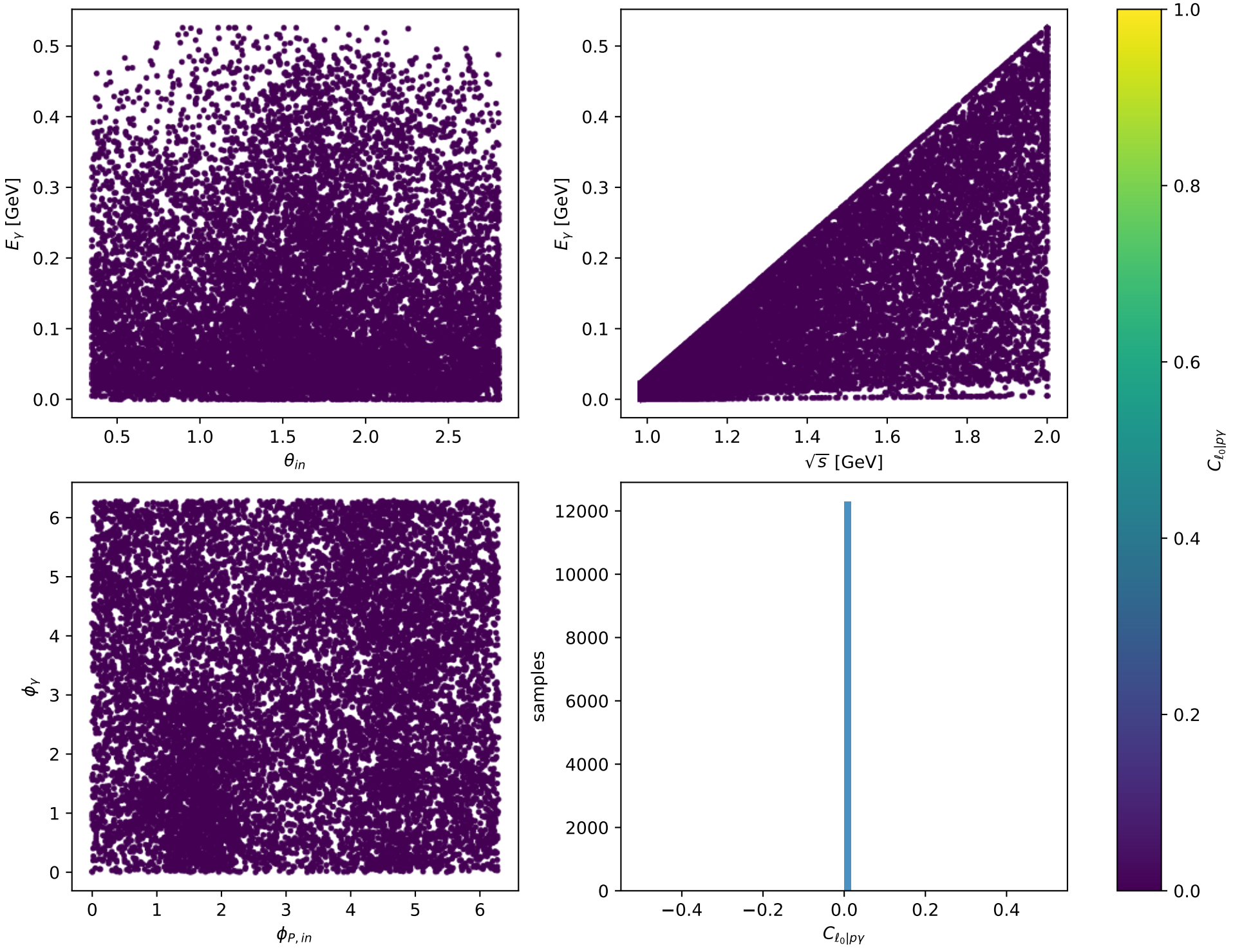
Phase-space scan: Ty massless lepton [Ty_electron], max C_{\ell_0|p\gamma}=0
